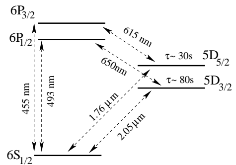
FIG. 1: Energy levels of \text{Ba}^+ showing the different transitions between 6s , 6p and 5d states.
