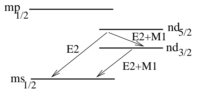
FIG. 1: Schematic diagram for the energy levels of the ms , mp and nd states transition lines in \text{Ca}^+ , \text{Sr}^+ and \text{Ba}^+ . The m and n represent the principal quantum numbers of the ground and metastable states.
