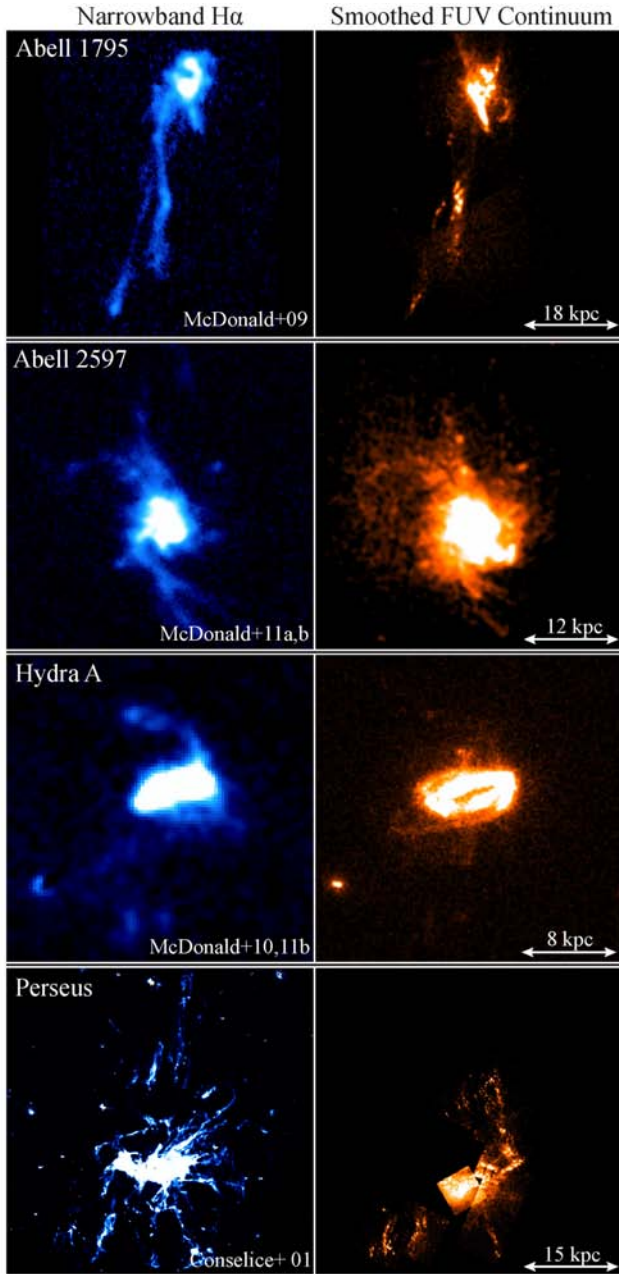
Figure 3. A comparison of H \alpha and FUV continuum morphologies for a subset of our sample. In blue, we show the narrow-band H \alpha images from McDonald et al. (2010, 2011a,b); Conselice et al. (2001), and in orange we show the FUV continuum images after Gaussian smoothing to (approximately) match the spatial resolution of the H \alpha maps. All image pairs are aligned and shown on a common spatial scale, with east left and north up. The morphologies are very similar overall, though it is important to note that some H \alpha filaments lack detected cospatial FUV continuum, and some FUV filaments lack detected cospatial H \alpha emission (though non-detection of course does not necessarily imply absence). Many works have demonstrated that continuum emission from young stars can account for a dominant fraction of the ionizing photons needed to power the H \alpha nebula (e.g. O’Dea et al. 2010; McDonald et al. 2011a). However, an additional ionization mechanism (e.g. shocks, cosmic rays, thermal conduction, etc.) is needed in all cases (see Section 1).
