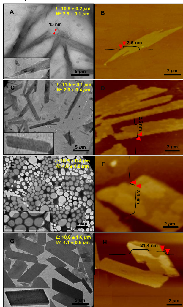
Figure 3. TEM and AFM images of the 2D aggregates formed by the hierarchical self-assembly of GC-91 in THF–water (v/v 4:1) at 10 °C after (A, B) 5 h, (C, D) 1 days, (E, F) 5 days, and (G, H) 10 days. The average lengths ( L ), widths ( W ), and thicknesses of the aggregates are indicated in the corresponding TEM and AFM images.
