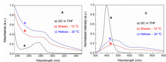
Figure 4. (A) UV-vis and (B) photoluminescence spectra of GC-91 in THF as well as of the helices and the sheets in THF-water (v/v 4:1) at different temperatures (concentration: 2 \times 10^{-4} mg mL -1 ).
