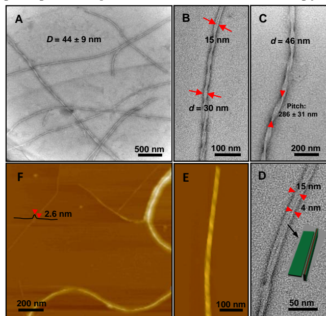
Figure 2. TEM and AFM images of the helices formed by the hierarchical self-assembly of the GC-91 graft copolymers in THF–water (v/v 4:1) at 20 °C. (A) A low-magnification TEM image of the helices ( D denotes the average diameter); (B, C) high-magnification TEM images of the double- and triple-stranded helices with related sizes indicated ( d expresses a diameter of a specific helix); (D) an HRTEM micrograph of an untwisted region in a double-stranded helix, in which a ribbon-like aggregate is positioned vertical to the substrate (inset); (E) an AFM height profile of a helix; (F) an AFM height image scanned after strong sonication of the helix dispersion in THF–water.
