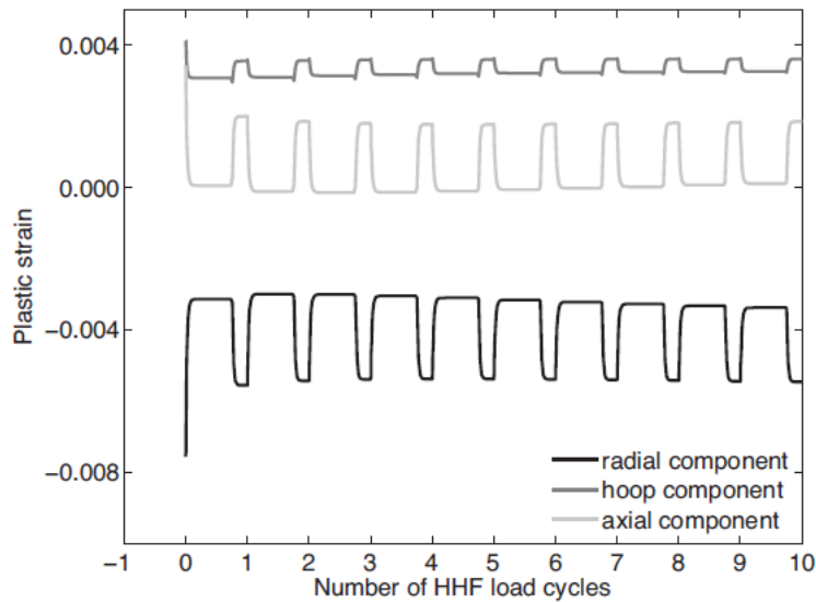
Fig. 14. History of the principal plastic strain components in the copper interlayer during the HHF load cycles. The fabrication process and pre-heating to standby state are also considered [30].
