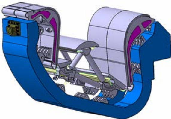
Fig. 1. Initial version of the CAD model of the DEMO divertor cassette [3].
