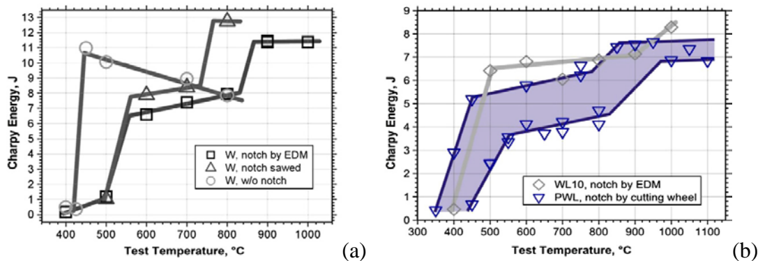
Fig. 7. Data of Charpy impact tests conducted for rod specimens of pure W (a) and La oxide-doped W (b) [28].
