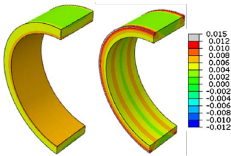
Fig. 12. Hoop (left) and axial (right) component of the plastic strain in the cooling tube after 10 load cycles (heat flux load: 15 MW/m 2 , coolant temperature of 200 °C) [30].
