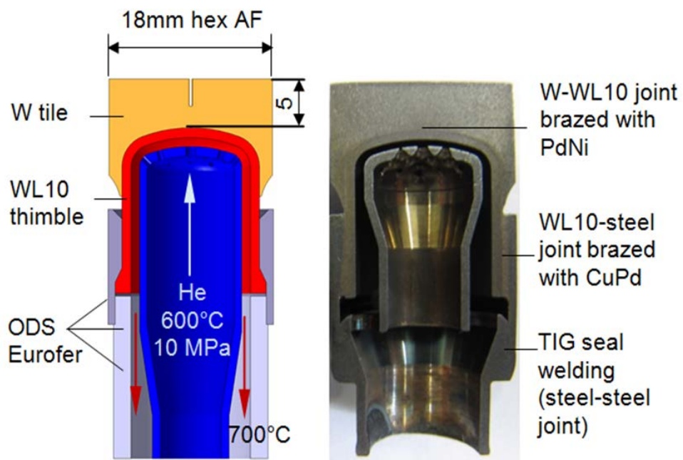
Fig. 15. Longitudinal section view of a multi-jet modular finger target unit with a schematic illustration (left) and photograph (right) [37].
