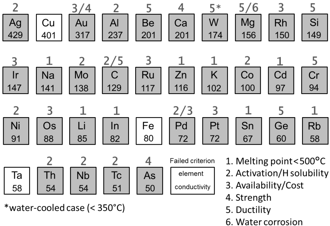
Fig. 2. Pure materials in solid state which possess thermal conductivity higher than 50 W/m·K. In each box the value of conductivity is given. The grey-shaded boxes indicate the materials that fail to meet at least one or two of the criteria. The 'failed' item of the criteria is indicated on the top of the individual boxes, respectively.
