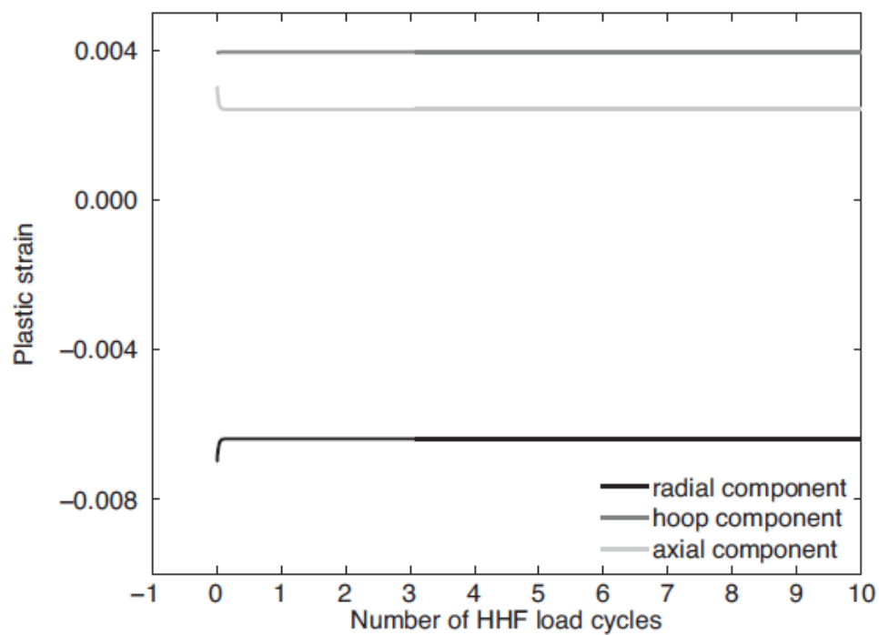
Fig. 13. History of the principal plastic strain components in the cooling tube bulk during the HHF load cycles (cylindrical coordinate system). The fabrication process and pre-heating to standby state are also considered [30].
