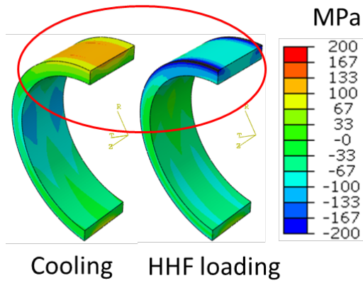
Fig. 11. Hoop component of the thermal stress field produced in the cooling tube after 10 load cycles (heat flux load: 15 MW/m 2 , coolant temperature of 200 °C) [30].
