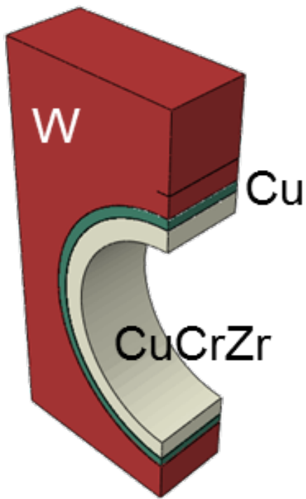
Fig. 9. Schematic of the water-cooled target model (symmetric half) considered for FEA. W armor block: 23 mm×22 mm×4 mm, cooling tube thickness: 1 mm, inner diameter: 12 mm, Cu interlayer thickness: 0.5 mm.
