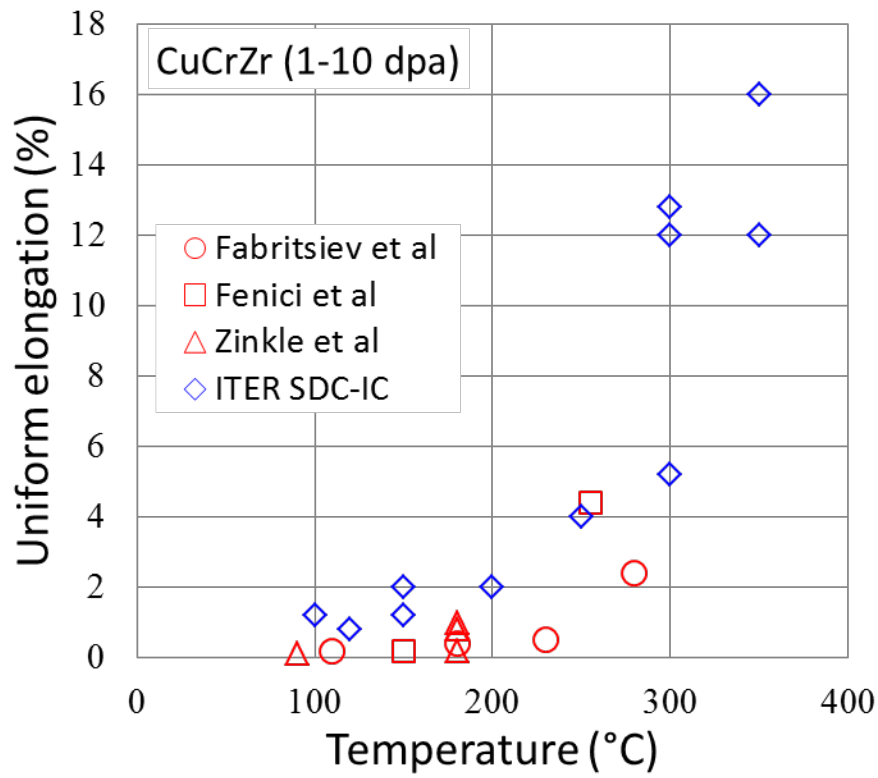
Fig. 3 Uniform elongation data of CuCrZr alloy irradiated to 1-10 dpa plotted as a function temperature. The data were collated from several different test reports published in literature [19-21].
