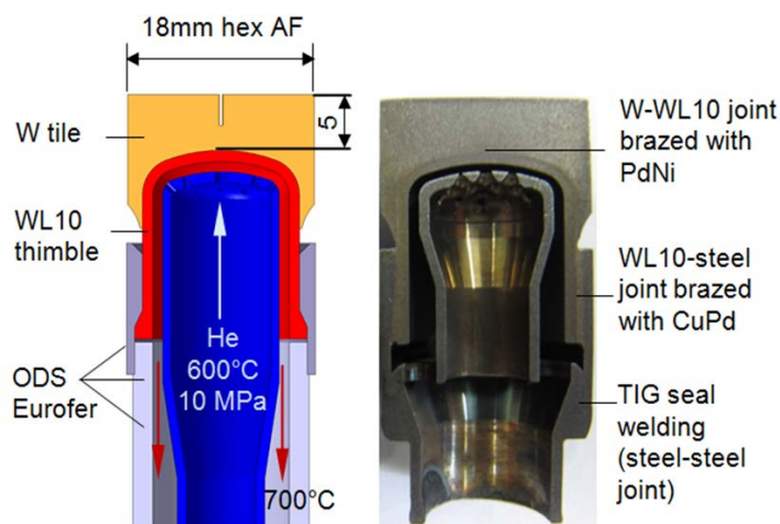
Fig. 15. Longitudinal section view of a multi-jet modular finger target unit with a schematic illustration (left) and photograph (right) [38].
