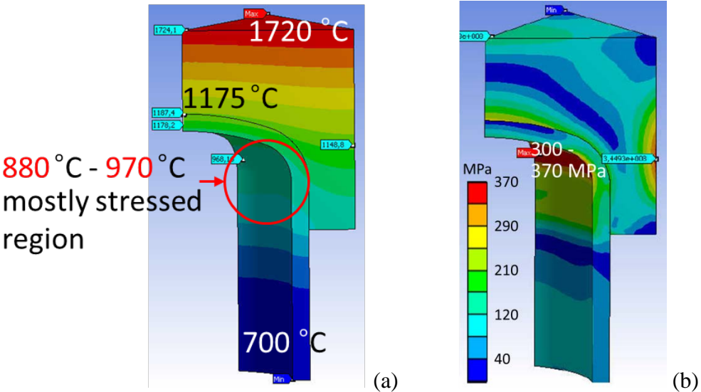
Fig. 16. Temperature (a) and von Mises stress (b) fields produced in a modular finger target unit (symmetric one sixth part is modelled) computed by a thermo-hydraulic FEA [38].
