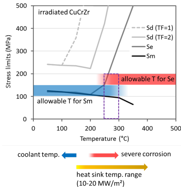
Fig. 5. Selected stress limits of CuCrZr alloy from the SDC-IC code plotted as a function of temperature. The subscript ‘irr’ and ‘unirr’ stands for the data of an irradiated and pristine specimen, respectively [22].
