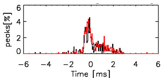
Figure 1: Filament activity along a Type-I ELM cycle in JET. PDFs of detection times of positive (black) and negative (red) V_r peaks, F=73.44 \text{ GHz} .
