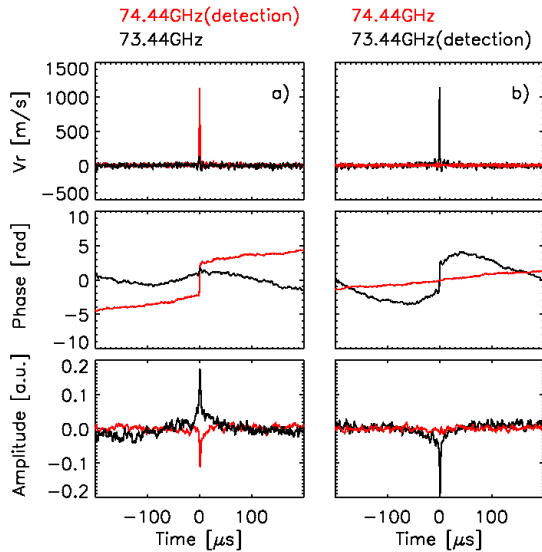
Figure 2: Inter-ELM filament signatures on reflectometry signals at JET using CA and detection signals from F=74.44\text{GHz} a) and F=73.44\text{GHz} b).
