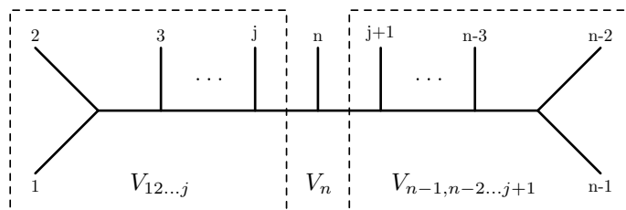
Figure 2. The (n - 2)! half-ladder diagrams with legs 1 and n - 1 attached to opposite endpoints encode the complete kinematic dependence in a BCJ representation.
