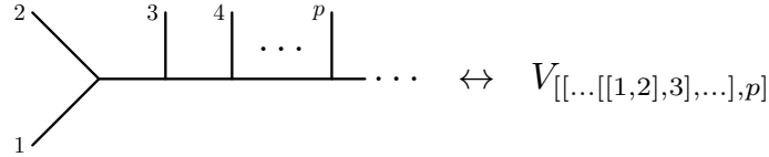
Figure 1. The tree diagram with an off-shell leg is represented by the local superfield (4.6).
