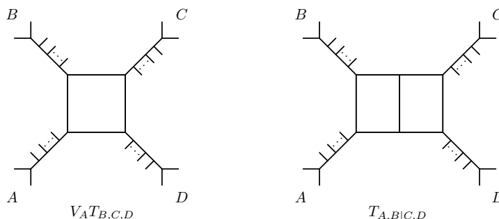
Figure 2. The pure spinor expressions of arbitrary box and double-box numerators are given by certain multiparticle building blocks V_A T_{B,C,D} [14] and T_{A,B|C,D} [15]. They furnish a manifestly local representation that satisfies the BCJ identities within each external tree subdiagram when the SYM superfields are in the BCJ gauge.
