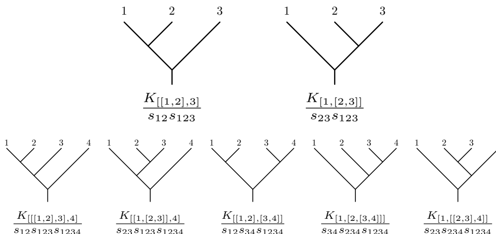
Figure 3. The planar binary trees used to define \mathcal{K}_{123} and \mathcal{K}_{1234} .
