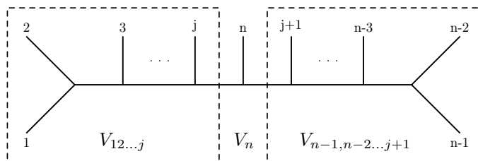
Figure 1. The basis of half-ladder diagrams with legs 1 and n-1 attached to opposite endpoints furnish the manifestly-local pure spinor representation of tree-level numerators V_{12\dots j}V_nV_{n-1,n-2,\dots,j+1} built from SYM superfields in the BCJ gauge.
