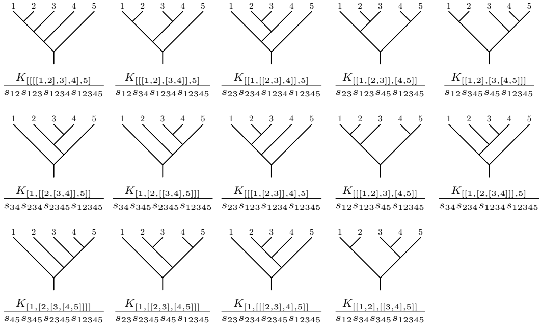
Figure 4. The fourteen binary trees used in the definition of \mathcal{K}_{12345} .
