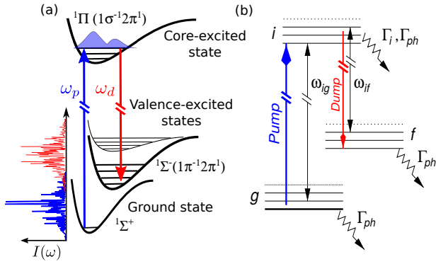
FIG. 1. Two-color stimulated RIXS scheme driven by a pair of temporally overlapping SASE pulses. a) The pump field of frequency \omega_p is resonant to the intermediate core-excited state {}^1\Pi of CO; the probe field of frequency \omega_d stimulates inelastic Raman scattering channel from the core-excited to a valence-excited state {}^1\Sigma^- . b) Generalized electronic-vibrational level scheme of stimulated RIXS in molecules.
