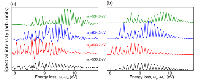
FIG. 8. (a) SRIXS spectra obtained with the help of the covariance map of Fig. 7(d) using a narrow spectral window (0.2 eV) around \omega_p = 532.2, 533.7, 534.2, and 534.6 eV. (b) Conventional RIXS simulations at the narrow band (0.05 eV) excitation for the same \omega_p energies as in (a).
