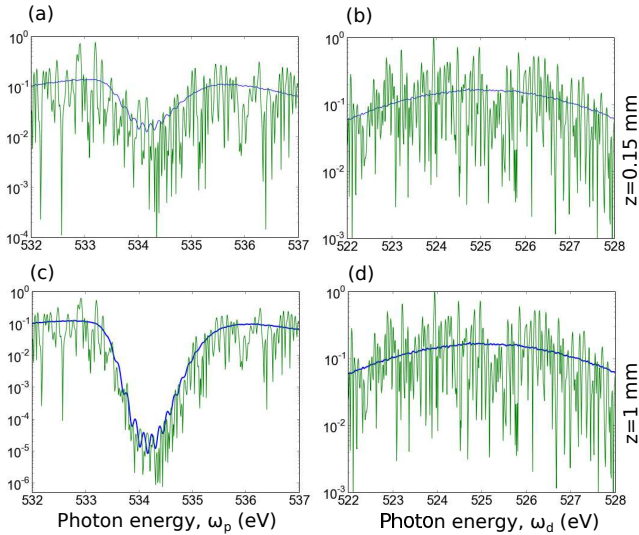
FIG. 9. The spectrum of a typical transmitted pair of SASE pulses (green) at the excitation (a and c) and emission (b and d) transitions and their ensemble average (blue). Panels (a) and (b) correspond to the transmitted spectrum of a propagation distance of z = 0.15 mm and (c) and (d) z = 1 mm. Due to strong resonant absorption of the pump radiation a larger dynamic range of the spectrometer set-up is required for the longer medium.
