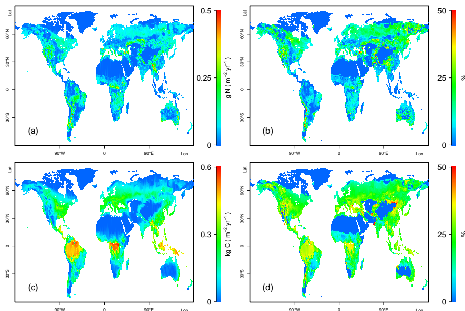
Figure 5. Responses in simulated biological nitrogen (N) fixation (BNF) and net primary production (NPP) rates to elevated atmospheric \text{CO}_2 concentrations ( \text{eCO}_2 ), taken as the difference between the simulations B ( \text{eCO}_2 ) and A (ambient \text{CO}_2 ), averaged over the experiment years 140–153, corresponding to a difference in atmospheric \text{CO}_2 concentrations of 211 ppm. (a) Absolute model-median BNF responses. (b) Relative model-median BNF responses ( (\text{treatment/control} - 1) \times 100 , %). (c) Absolute model-median NPP responses. (d) Relative model-median NPP responses. Figures B3 and B4 provide BNF and NPP maps for each model separately.
