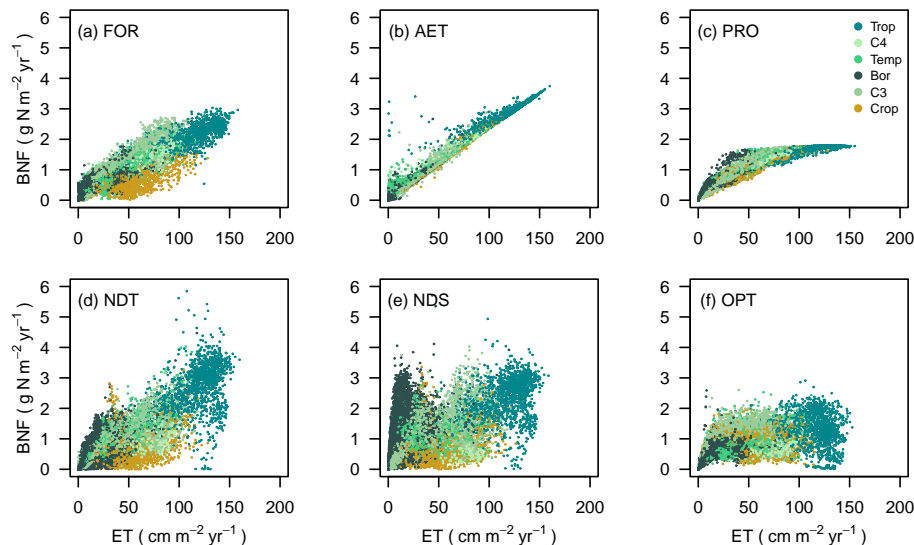
Figure B5. Simulated (simulation A) global relationship between biological nitrogen (N) fixation (BNF) and evapotranspiration (ET), averaged for 2000–2013. Each marker represents one O-CN grid cell. Colors indicate the dominant vegetation type in each grid cell. Trop = Tropical forest, C4 = C 4 grassland, Temp = Temperate forest, Bor = Boreal forest, C3 = C 3 grassland, Crop = Agriculture.
