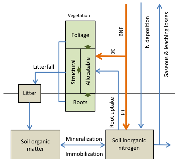
Figure 1. Scheme of nitrogen (N) cycle representation in O-CN. Reactive N species (ammonium, nitrate) enter the ecosystem through atmospheric deposition directly into the pool of soil inorganic N, as well as through biological N fixation (BNF, as ammonium). N from asymbiotic BNF (a) enters the soil inorganic N pool, whereas N from symbiotic BNF (s) becomes directly available to plants for allocation to their various organs. N in plant litter is assimilated into soil organic matter and may be mineralized and transferred to the soil inorganic N pool, depending on that pool's size and the C:N ratio of the soil organic matter. The soil inorganic N pool is depleted by plant root N uptake, immobilization (transfer to soil organic matter), as well as by leaching or gaseous loss processes. Global magnitudes of the key N fluxes in O-CN can be found in Table 2. O-CN does not include fluxes of geological N inputs, plant organic N uptake, or canopy N uptake.
