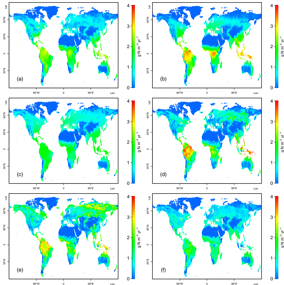
Figure B1. Global biological nitrogen (N) fixation (BNF) rates, as simulated by O-CN applying the six different BNF models for 2000–2013. (a) FOR; (b) AET; (c) PRO; (d) NDT; (e) NDS; (f) OPT.
