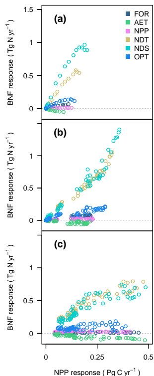
Figure 6. Net primary productivity (NPP) and biological nitrogen (N) fixation (BNF) responses to elevated atmospheric \text{CO}_2 concentrations ( \text{eCO}_2 ), taken as the absolute difference between the simulations B ( \text{eCO}_2 ) and A (ambient \text{CO}_2 ), averaged over the experiment years 140–153, corresponding to a difference in atmospheric \text{CO}_2 concentrations of 211 ppm. Each marker represents one global latitudinal band of 1^\circ extent. (a) Responses in the boreal latitudes ( 90^\circ \text{N} – 61^\circ \text{N} ). (b) Responses in the temperate latitudes ( 60 – 31^\circ \text{N} , 31 – 60^\circ \text{S} ). (c) Responses in the tropical latitudes ( 30^\circ \text{N} – 30^\circ \text{S} ).
