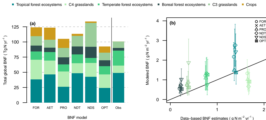
Figure 4. Average biological nitrogen (N) fixation (BNF) rates in different biome types as simulated by O-CN, applying the different BNF models for 2000–2013 (simulation A). (a) Total global BNF rates (Tg N yr -1 ), segments indicate the contributions of individual biome types. “Obs” denotes data-based estimates, as published in Table 13 of Cleveland et al. (1999) (conservative estimates of total N fixation). (b) BNF rates (g N m -2 yr -1 ) as simulated by the different BNF models, compared with the conservative estimates by Cleveland et al. (1999). For the modeled BNF rates, markers indicate the mean value over all grid cells that included the respective biome type, error bars indicate the corresponding standard deviation. The black line is the one-to-one line. Details on the classification of vegetation types from the data source into the plant functional types applied in O-CN can be found in Table B1.
