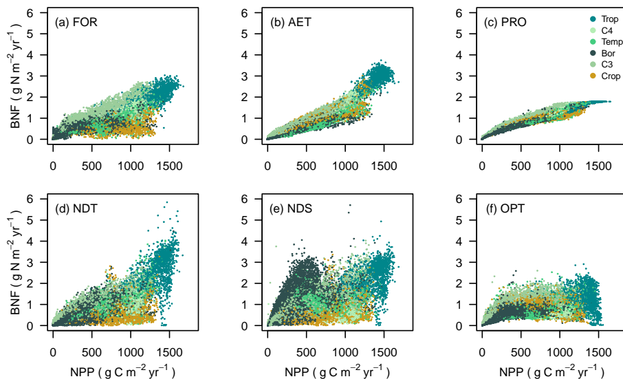
Figure B6. Simulated (simulation A) global relationship between biological nitrogen (N) fixation (BNF) and net primary productivity (NPP), averaged for 2000–2013. Each marker represents one O-CN grid cell. Colors indicate the dominant vegetation type in each grid cell. Trop = Tropical forest, C4 = C 4 grassland, Temp = Temperate forest, Bor = Boreal forest, C3 = C 3 grassland, Crop = Agriculture.
