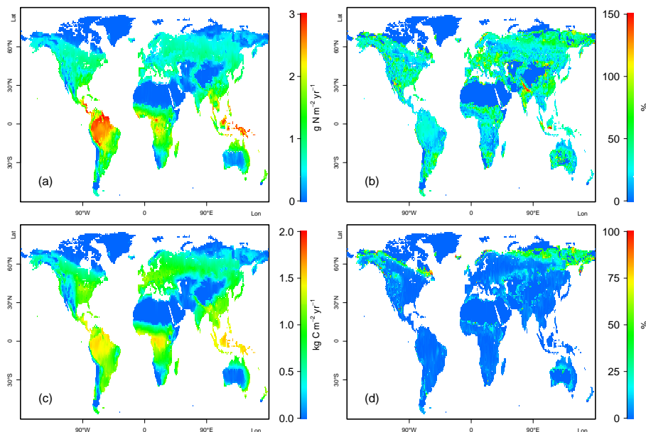
Figure 3. Global biological nitrogen (N) fixation (BNF) and net primary production (NPP) rates, as simulated by O-CN (simulation A) applying the six different BNF models for 2000–2013. (a) Model-median BNF ( \text{g N m}^{-2} \text{yr}^{-1} ). (b) Median relative deviation (MRD) from the median BNF across models (%). (c) Model-median NPP ( \text{kg C m}^{-2} \text{yr}^{-1} ). (d) MRD from the median NPP across models (%). Figures B1 and B2 provide BNF and NPP maps for each model separately.
