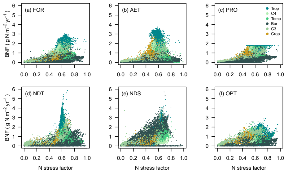
Figure B7. Simulated (A) global relationship between biological nitrogen (N) fixation (BNF) and the relative distance of leaf C : N ratios from the minimal value (“N stress factor”), averaged for 2000–2013. Each marker represents one O-CN grid cell. Colors indicate the dominant vegetation type in each grid cell. Trop = Tropical forest, C4 = \text{C}_4 grassland, Temp = Temperate forest, Bor = Boreal forest, C3 = \text{C}_3 grassland, Crop = Agriculture.
