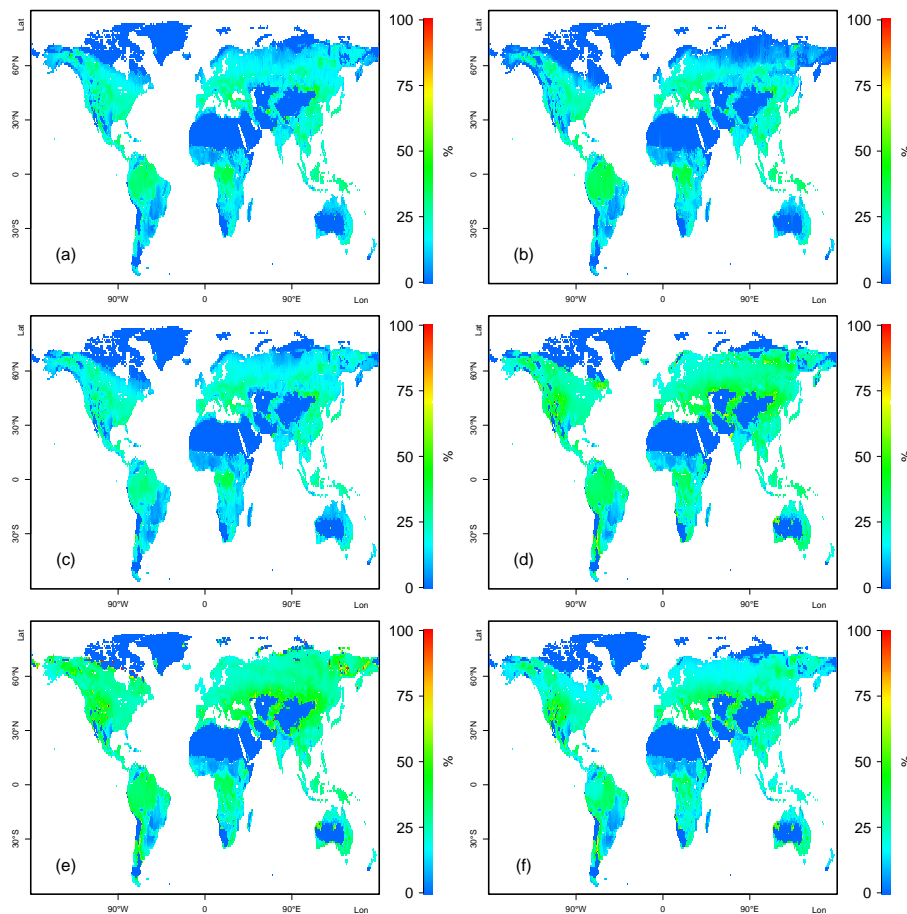
Figure B4. Responses in simulated net primary productivity (NPP) rates to elevated atmospheric \text{CO}_2 concentrations ( \text{eCO}_2 , Fig. 5, (treatment/control – 1) \times 100), averaged over the experiment years 140–153. (a) FOR; (b) AET; (c) PRO; (d) NDT; (e) NDS; (f) OPT.
