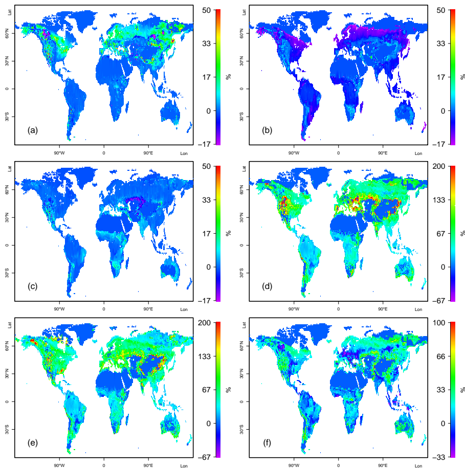
Figure B3. Responses in simulated biological nitrogen (N) fixation (BNF) rates to elevated atmospheric CO 2 concentrations (eCO 2 , Fig. 5, (treatment/control – 1) × 100), averaged over the experiment years 140–153. (a) FOR; (b) AET; (c) PRO; (d) NDT; (e) NDS; (f) OPT.
