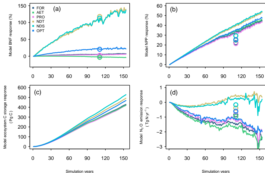
Figure 7. Simulated ecosystem responses to elevated atmospheric \text{CO}_2 concentrations ( \text{eCO}_2 ) as global time series, obtained using six different biological nitrogen (N) fixation (BNF) schemes. Curves show the differences between the simulations B (atmospheric \text{CO}_2 concentrations gradually increasing from 286 to 600 ppm) and C (atmospheric \text{CO}_2 fixed at 286 ppm). Markers show the responses between the simulations D (observed atmospheric \text{CO}_2 + 200 ppm) and A (observed atmospheric \text{CO}_2 ), calculated as averages over the simulation years 136–140. They are plotted at the simulation year 108, so that for all responses, the difference between control and treatment in atmospheric \text{CO}_2 concentration was approximately 200 ppm. (a) Relative BNF responses ( (\text{treatment}/\text{control} - 1) \times 100 ). (b) Relative net primary production (NPP) responses. (c) Absolute ecosystem carbon (C) storage responses ( \text{treatment} - \text{control} ). (d) Absolute \text{N}_2\text{O} emission responses.
