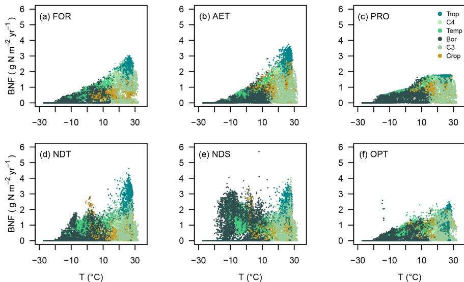
Figure B8. Simulated (A) global relationship between biological nitrogen (N) fixation (BNF) and surface temperature (T), averaged for 2000–2013. Each marker represents one O-CN grid cell. Colors indicate the dominant vegetation type in each grid cell. Trop = Tropical forest, C4 = C 4 grassland, Temp = Temperate forest, Bor = Boreal forest, C3 = C 3 grassland, Crop = Agriculture.
