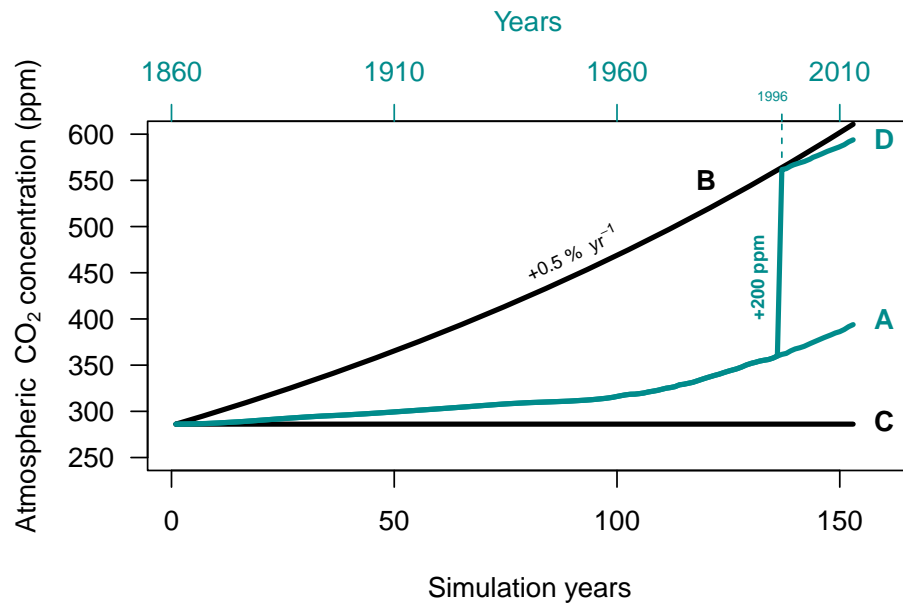
Figure 2. Atmospheric CO 2 concentrations applied in the simulations.
