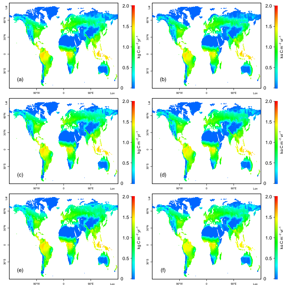
Figure B2. Global net primary productivity (NPP) rates, as simulated by O-CN applying the six different biological nitrogen fixation models for 2000–2013. (a) FOR; (b) AET; (c) PRO; (d) NDT; (e) NDS; (f) OPT.
