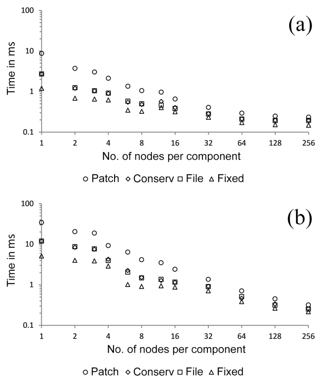
Figure 1. Time required for ping-pong exchange between (a) an ICONR2B06 and a 405 \times 405 cubed-sphere grid and (b) an ICONR2B07 and a 810 \times 810 cubed-sphere grid.
