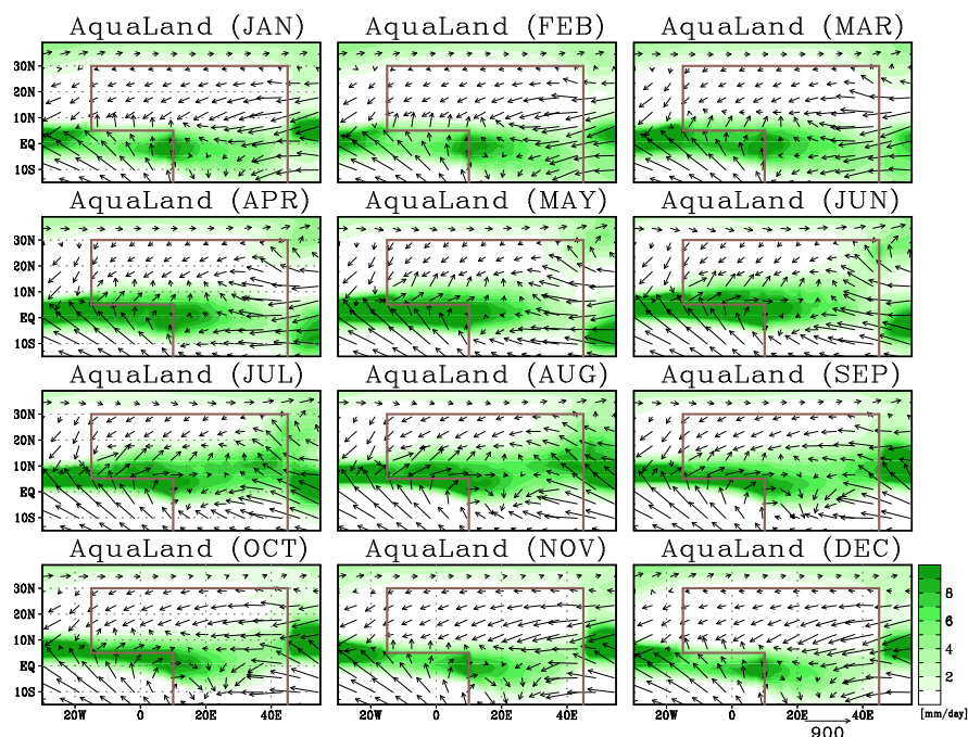
Figure 5.3. The climatological-mean rainfall (shading, unit: \text{mm day}^{-1} ) and vertically-integrated low-level (1000-700hPa) moisture flux (arrows, unit: \text{kg m}^{-2}\cdot\text{m s}^{-1} ) from January to
