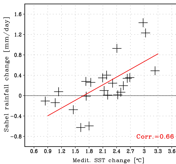
Figure 4.2. Scatter plots of future changes (i.e. mean difference between the twenty-first-century and twentieth-century) in Sahel rainfall versus Mediterranean SST across the CMIP5
