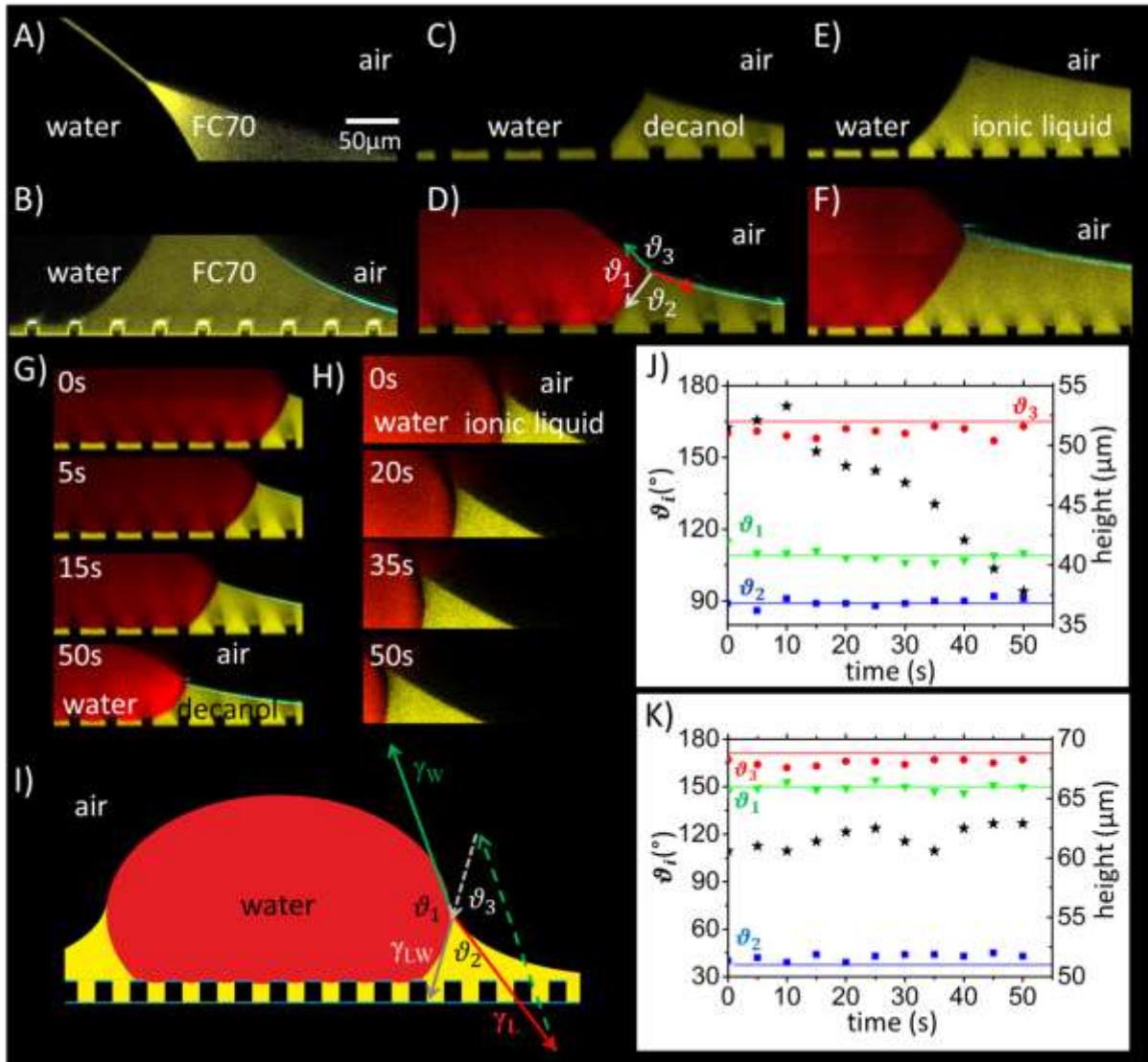
Figure 4. Cloaking of drops or a liquid-three phase contact line. A-B) Confocal images of vertical sections through a water drop placed on lubricant-impregnated micropillar arrays (black rectangles). FC70, decanol and ionic liquid were used as lubricants. A, B) Fluorescence signals (yellow) of FC70 and the reflection of light from the lubricant–air interface (cyan). C, D) Fluorescence signals (yellow) of decanol. The combined image (D) shows the fluorescence signal of the lubricant, the water drop (red) and reflection of light (cyan). E, F) Fluorescence signals (yellow) of ionic liquid. The combined image (F) shows the fluorescence signal of the lubricant, the water drop (red) and reflection of light (cyan). G,H) Time series of an evaporating water drop on (G) a decanol and (H) an ionic liquid lubricated micropillar array. I) Sketch of the Neumann triangle with the interfacial tensions and the contact angles \vartheta_i . Measured and calculated contact angles (left) and the height of the wetting ridge for a water drop deposited on (J) a decanol lubricated micropillar array and (K) an ionic liquid lubricated micropillar surface. The solid lines show the calculated angles according to Eq. 2. The \vartheta_i are defined according to Fig. 4I.
