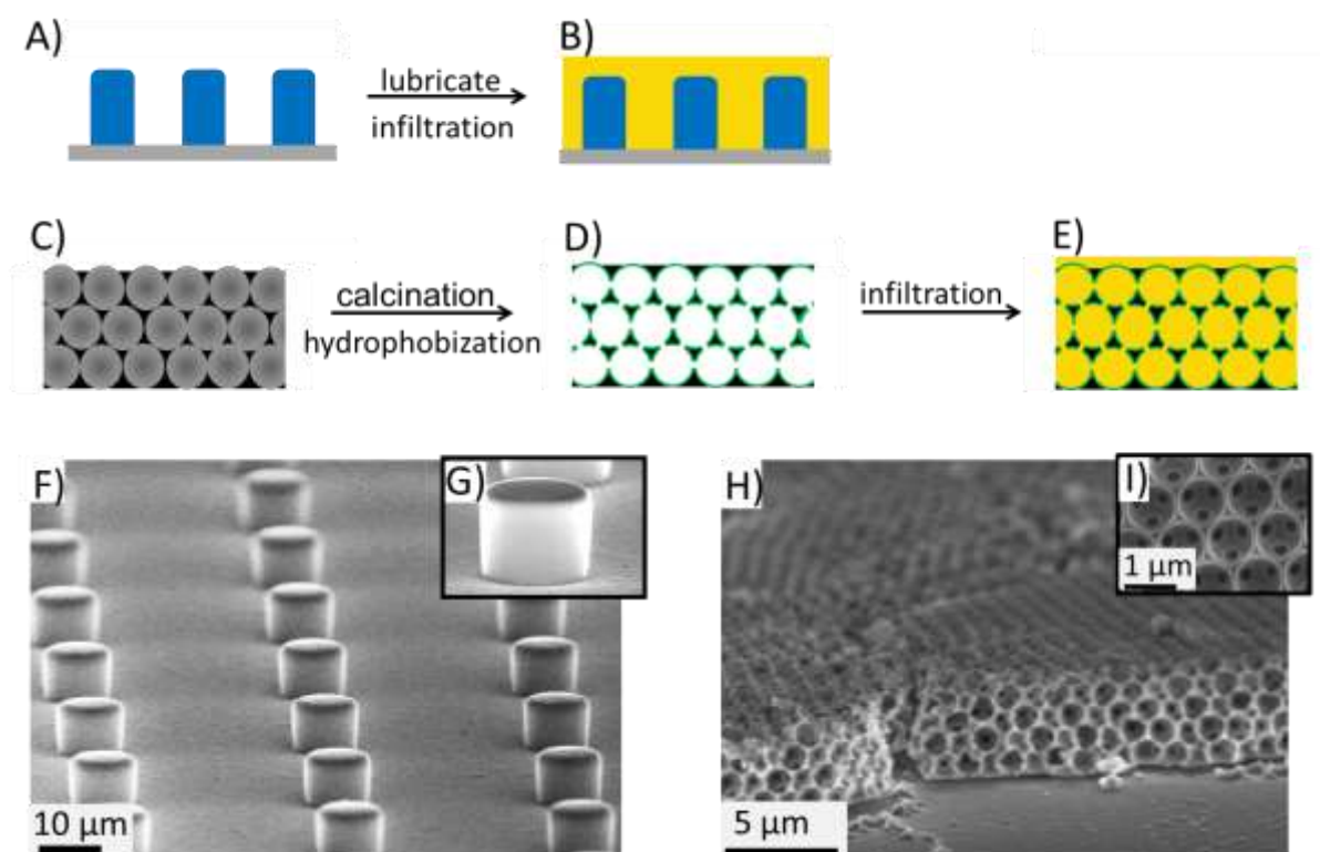
Figure 2. Schematic illustration of the fabrication of slippery surfaces. A-B) Cylindrical micropillar arrays (blue) infiltrated with a lubricant (yellow). The dimensions of the pillars employed in this study
