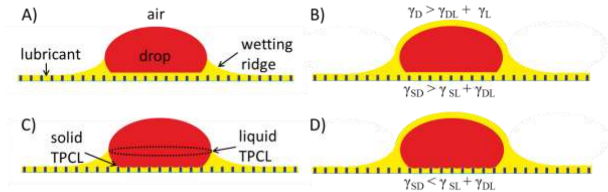
Figure 1. Wetting configurations. Schematic illustrations of possible wetting configurations of a slippery lubricant-infused textured surface. A, C) The drop (red) resting on a micropillar array (blue) is surrounded by an annular wetting ridge that may end in a pulled-up liquid three phase contact line (liquid-TPCL). The lubricant (yellow) does not cloak (A, C) or it may cloak (B, D) the drop. Drops on slippery surfaces can exhibit zero, one, or two three-phase contact lines. The liquid-TPCL is the line at which the air, drop, and lubricant meet, and the solid-TPCL is where the substrate, drop, and lubricant meet. The interfacial tensions \gamma_{ij} are denoted as follows: \gamma_{DL} - interfacial tension between the drop and the lubricant; \gamma_{SD} - interfacial tension between the surface and the drop; \gamma_{SL} - interfacial tension between the surface and the lubricant. \gamma_D represents the surface tension drop-air and \gamma_L the surface tension lubricant-air.
