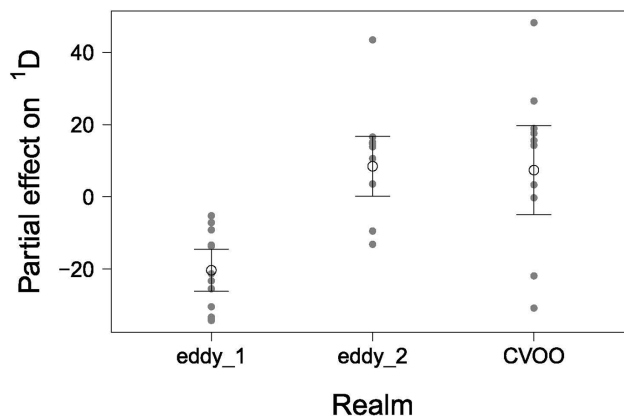
Figure 6. Alpha diversity analysis of eddy sampling stations (first observation (eddy_1), second observation (eddy_2)) and CVOO expressed as Shannon numbers equivalent ( 1 D). A strong and significant decrease in diversity is observed in the eddy. Partial response residuals (black symbols) were extracted from full GLS model refitted without the “Realm” main effect. Predicted values for partial residuals modelled by the “Realm” main effect alone (and thus adjusted for differences in O 2 concentration) are shown as blue symbols. Error bars represent 95 % confidence interval for fitted values.
