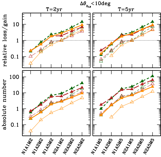
FIG. 10. Number of detections such that the absolute error in the measurement of both misalignment angles \theta_{\chi 1} and \theta_{\chi 2} at the innermost stable circular orbit is less than 10 degrees. Left and right panels are for a mission lifetime of two years and five years, respectively. Inspirational-only waveforms have been used in all cases. The bottom panels represent the number of sources as a function of the eLISA configuration, while the top panels represent the gain/loss of a given configuration with respect to NGO, i.e., the ratio [number of sources for (NiAjMkLl)]/[number of sources with (N2A1MkL4)]. Long-dashed brown lines are for model popIII, solid orange lines for model Q3-d, and short-dashed green lines for model Q3-nod. Thick lines with filled triangles are for six links (L6), while thin lines with open triangles are for four links (L4).
