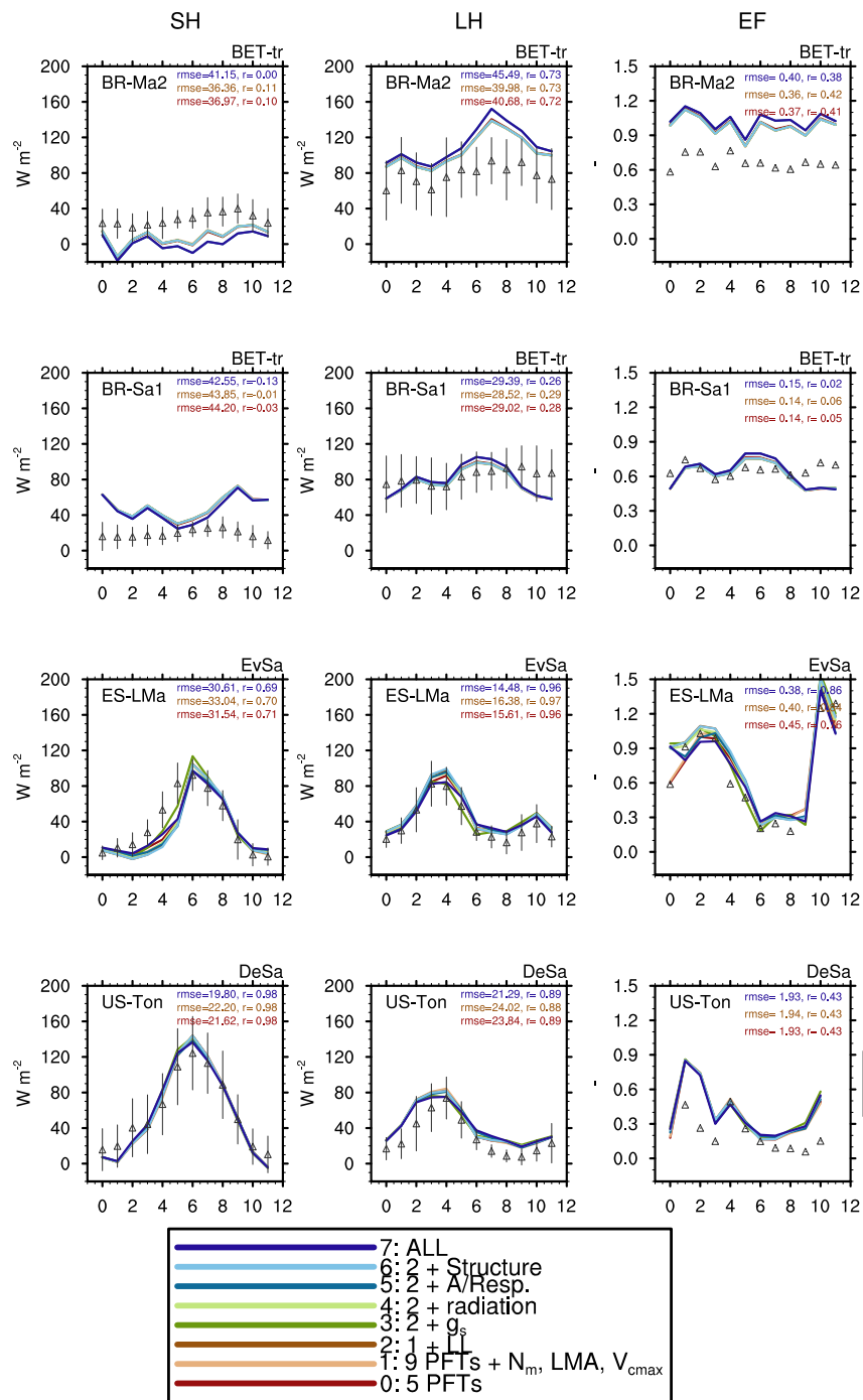
Figure S4a. Monthly mean fluxes of latent heat, sensible heat, and evaporative fraction ( =LE/(SH+LE) ) at two tropical forest sites (BET-tr) and two savannah sites (EvSa=Evergreen Savannah, DeSa=Deciduous Savannah). Observations \pm standard deviation from Fluxnet are shown with triangles and vertical lines.
