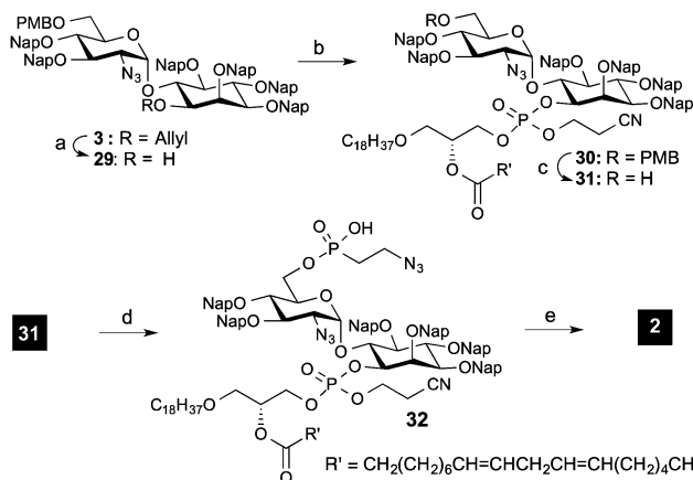
Scheme 5 Reagents and conditions: (a) i. \text{Ir}(\text{COD})_2\text{Cl}_2 , THF, rt, 5 h, ii. \text{HgCl}_2 , \text{HgO} , acetone, rt, 1 h, 91%; (b) i. 4 , 1 H -tetrazole, \text{CH}_2\text{Cl}_2 , rt, ii. t -BuOOH, \text{Me}_2\text{S} , -40^\circ\text{C} , 2 h, 87% (2 steps); (c) TFA, \text{CH}_2\text{Cl}_2 , 0^\circ\text{C} , 80%; (d) i. 5a , 1 H -tetrazole, DIPEA, toluene, 0^\circ\text{C} , 2 h, ii. \text{H}_2\text{O} , rt, 1 h, 87%; (e) i. DBU, \text{CH}_2\text{Cl}_2 , rt, ii. Zn, AcOH, \text{CH}_2\text{Cl}_2 , rt, iii. TFA, toluene, 0^\circ\text{C} , 72% (calculated from 32 ).
