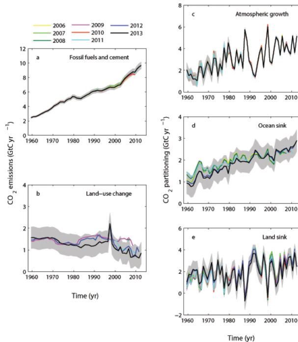
Fig. 6. Comparison of global carbon budget components released annually by GCP since 2005. CO 2 emissions from both (a) fossil-fuel combustion and cement production ( E_{FF} ), and (b) land-use change ( E_{LUC} ), and their partitioning among (c) the atmosphere ( G_{ATM} ), (d) the ocean ( S_{OCEAN} ), and (e) the land ( S_{LAND} ). See legend for the corresponding years, with the 2006 carbon budget from Raupach et al. (2007); 2007 from Canadell et al. (2007); to 2008 published online only; 2009 from Le Quéré et al. (2009); 2010 from Friedlingstein et al. (2010); 2011 from Peters et al. (2012b); 2012 from Le Quéré et al. (2013); and this year's budget (2013). The budget year corresponds to the year of the budget was first release. All values are in GtC yr -1 .
