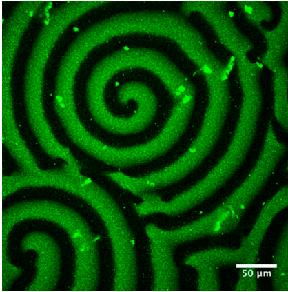
Spontaneous spiral wave patterns form when MinD, MinE, and ATP are added to a supported membrane.
