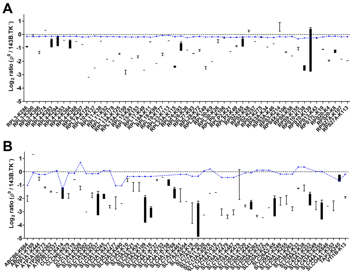
FIG. 7. De-ubiquitinated target proteins in \rho^0 cells. Proteins and their specific de-ubiquitination sites are shown for A, cytosolic ribosomal proteins and B, SLC transporter proteins and other transporter or channel proteins. The \log_2 ratios of all replicates ( n = 1 - 4 ) are shown (reversed values for label switches) in a box plot. For comparison, the mean of according \log_2 protein ratios is indicated by connected blue dots.
