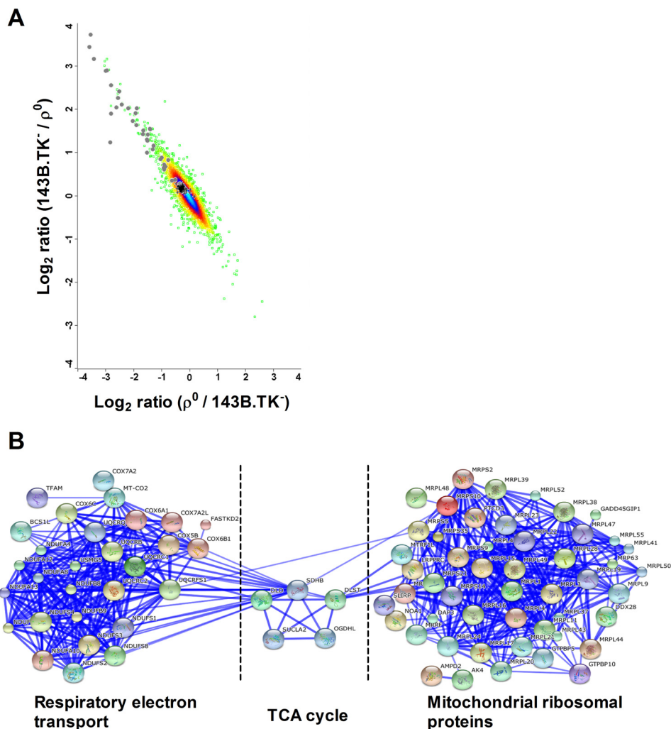
FIG. 4. Intensity scatter plot of protein abundances and a PPI network of down-regulated proteins in \rho^0 versus parental cells. A , Shown are unregulated cytoplasmic 80S ribosomal proteins, indicated by black crosses and mitochondrial 55S ribosomal proteins, which were down-regulated in \rho^0 cells, indicated by gray dots. B , Protein–protein interaction (PPI) network analysis of significantly down-regulated proteins in \rho^0 cells (average of valid values), featuring subunits of the respiratory electron chain, proteins involved in the TCA cycle and mitochondrial 55S ribosomal proteins. The proteins that are known to interact with each other are linked with a blue line. The cut off for regulated proteins was determined using two standard deviations from the median.
