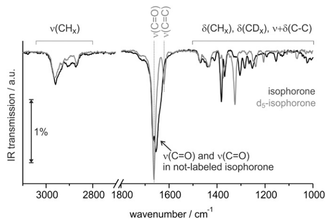
Fig. 2. IR spectra of 3 ML isophorone (black) and d_5 -isophorone (gray) at 120 K on Pd(111). The region characteristic for \text{C}\text{--H} stretching vibrations ( 3100\text{--}2800\text{ cm}^{-1} ), \text{C}=\text{O} and \text{C}=\text{C} stretching vibrations ( 1800\text{--}1600\text{ cm}^{-1} ), and \text{C}\text{--H} and \text{C}\text{--D} deformation and \text{C}\text{--C} deformation and stretching vibrations ( 1500\text{--}1000\text{ cm}^{-1} ).
