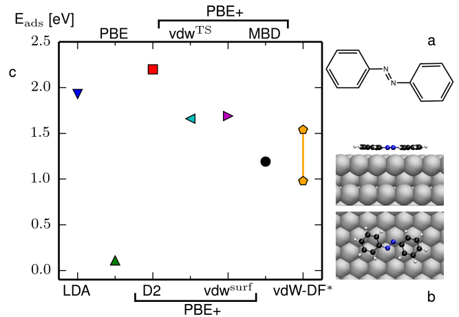
FIG. 1. a, Chemical formula of planar azobenzene. b, Side and top view of azobenzene adsorbed at a Ag(111) surface. c, Absolute adsorption energy E_{\text{ads}} = |\Delta U_{0\text{K}}| of azobenzene from Ag(111) as given by different DFT approximations. vdW-DF* refers to results from vdW-DF methods by Li et al. [11] using different underlying xc-functionals.
