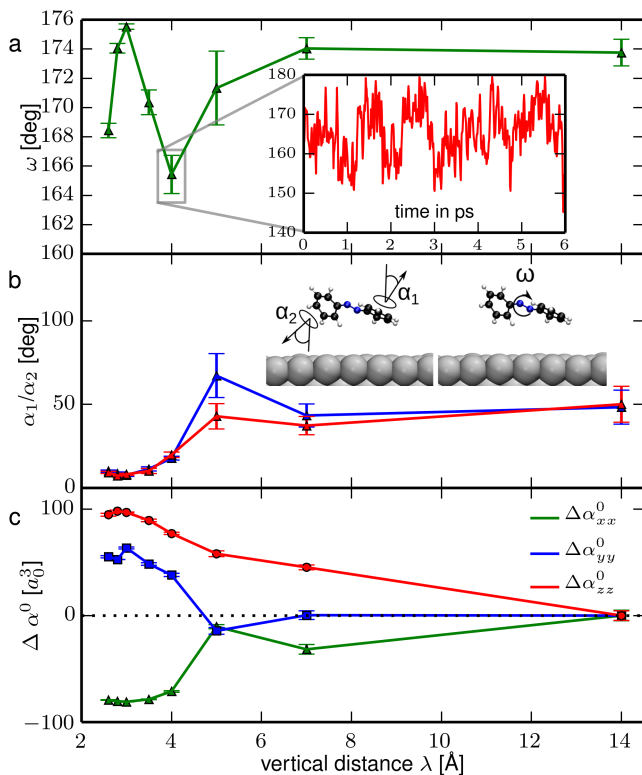
FIG. 3. a, Average central CNNC dihedral angle \omega as a function of the reaction coordinate \lambda . Also shown as inset is the real-time dynamics of \omega at 4 Å surface distance. b, Average angles \alpha_1 and \alpha_2 between the normal formed by the two phenyl rings and the surface normal. c, Change in Cartesian static polarizability components. All data points are given with statistical variances shown as error bars.
