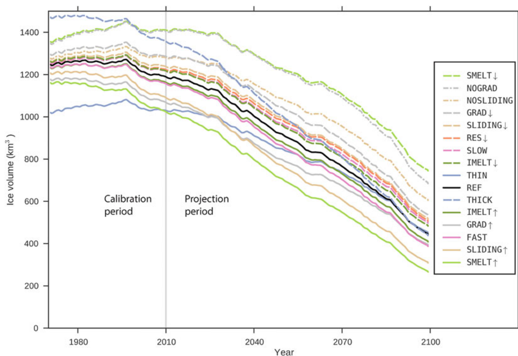
Fig. 8. Modeled evolution of annual ice volumes over the period 1971–2100 for the reference run and the sensitivity experiments (Table 2). The legend is sorted by final ice volume. Experiments in which the same parameter is varied share the same color.
