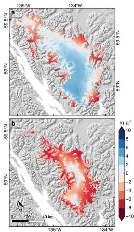
Fig. 13. Modeled surface mass balance over the ice-covered area (m w.e. a^{-1} ) (a) averaged over the period 1971–2000, and (b) averaged over the period 2070–99.
