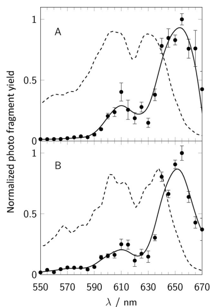
Figure 3. Total 2.3-photon-corrected action spectra for the dimer complexes compared to the monomer complexes (dashed lines). A) Complexes with charge tag 1^+ . B) Complexes with charge tag 3^+ . Line smoothing using spline functions was performed because of the low resolution of the dimer spectra. For the purpose of consistency between data sets, the same smoothing was applied to the monomer spectra.
