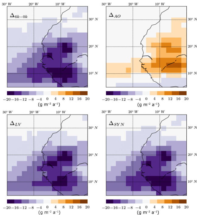
Figure 8. Differences in simulated dust deposition along the northwest African margin (30–17° W; 5–35° N) between 6k and 0k \Delta_{6k-0k} (top left), \Delta_{AO} (top right), \Delta_{LV} (bottom left) and the synergy effect \Delta_{SYN} (bottom right).
