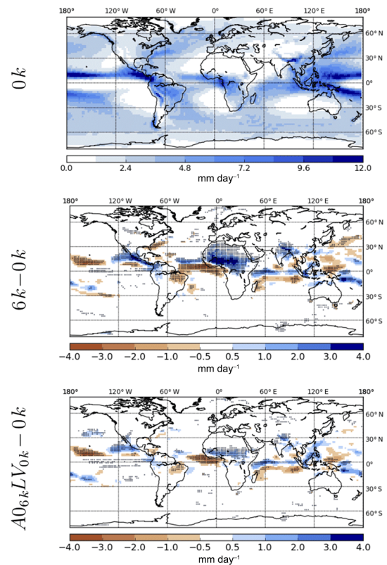
Figure B1. Mean annual precipitation for 0k and for the differences 6k-0k and AO_{6k}LV_{0k}-0k . Hatched areas in the difference plots show significant precipitation differences (99 % confidence level) according to a Student's t test.
