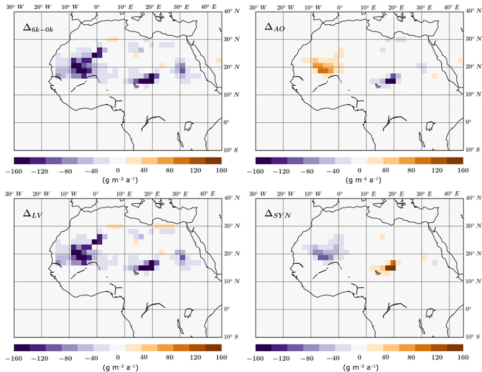
Figure 7. Differences in simulated dust emission in North Africa ( 17^{\circ} W– 40^{\circ} E; 10^{\circ} – 30^{\circ} N) between 6k and 0k, \Delta_{6k-0k} (top left), \Delta_{AO} (top right), \Delta_{LV} (bottom left) and the synergy effect \Delta_{SYN} (bottom right).
