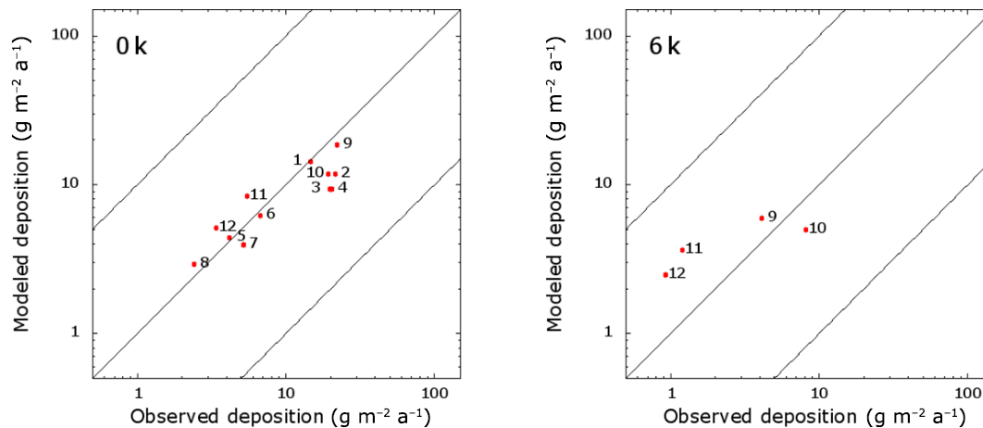
Figure 4. Simulated dust deposition flux for 0k (left, \text{AO}_{0k}\text{LV}_{0k} ) and 6k (right, \text{AO}_{6k}\text{LV}_{6k} ) compared with data from marine sediment cores and sediment traps (Table 4). Log correlation coefficients are 0.89 (0k) and 0.85 (6k).
