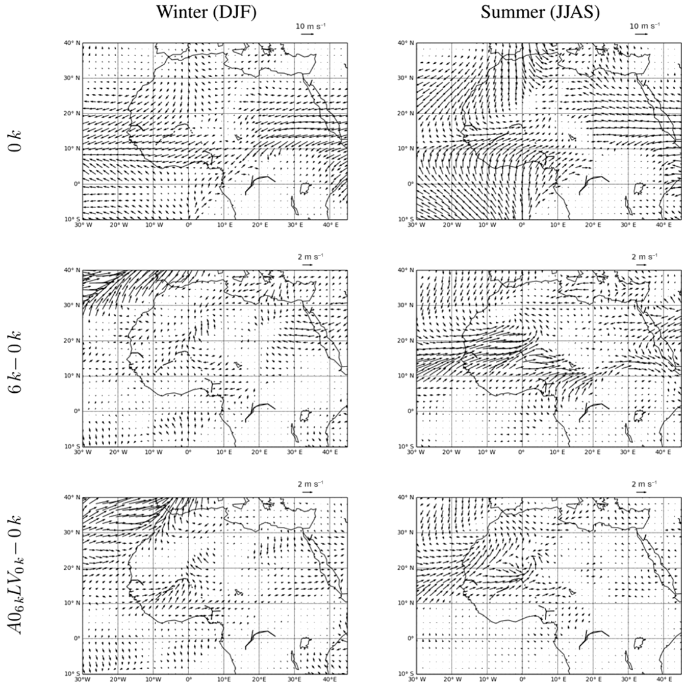
Figure A1. Simulated 10m surface wind speed and directions for winter (DJF; left) and summer (JJAS; right) for 0k and for the differences 6k-0k and A0_{6k}LV_{0k}-0k .
