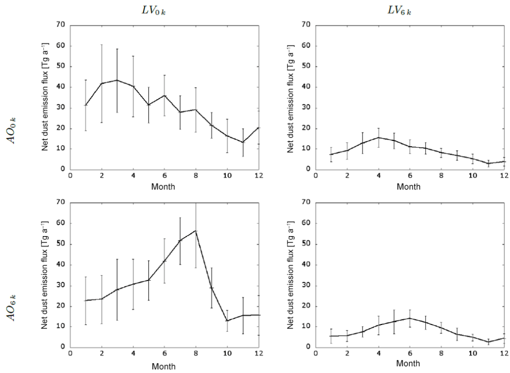
Figure A2. Mean annual cycle of simulated dust emission for altering atmosphere-ocean (AO) and land surface (LV) conditions in North Africa (17° W–40° E; 10–30° N).
