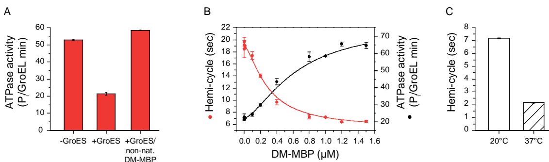
Figure 4.13 Presence of substrate stimulates GroEL ATPase activity
