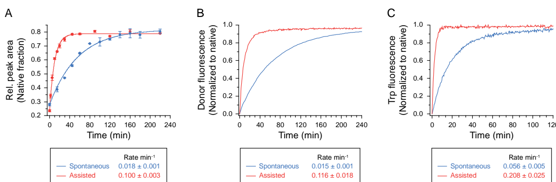
Figure 4.5 DM-MBP refolding is accelerated by GroEL/ES at single molecule level
