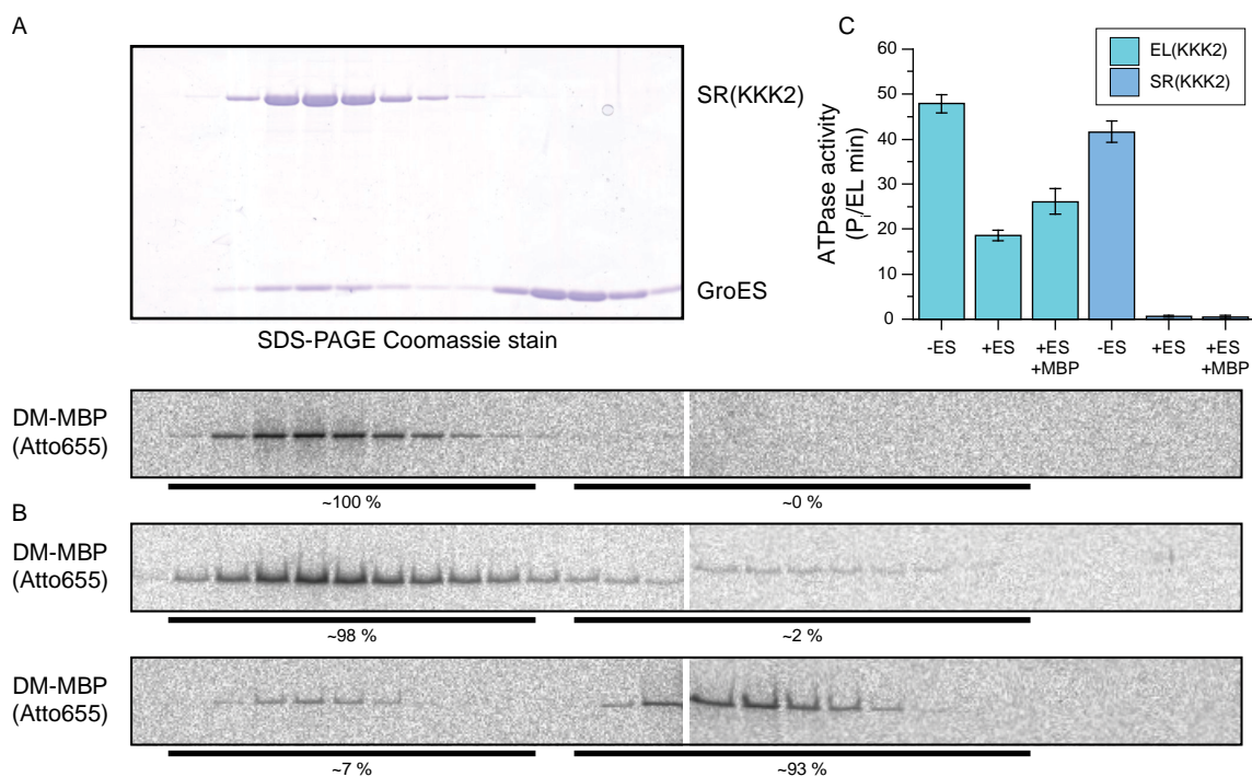
Figure 4.16 SR(KKK2) forms a stable cis-like complex with GroES that stably encapsulates DM-MBP
