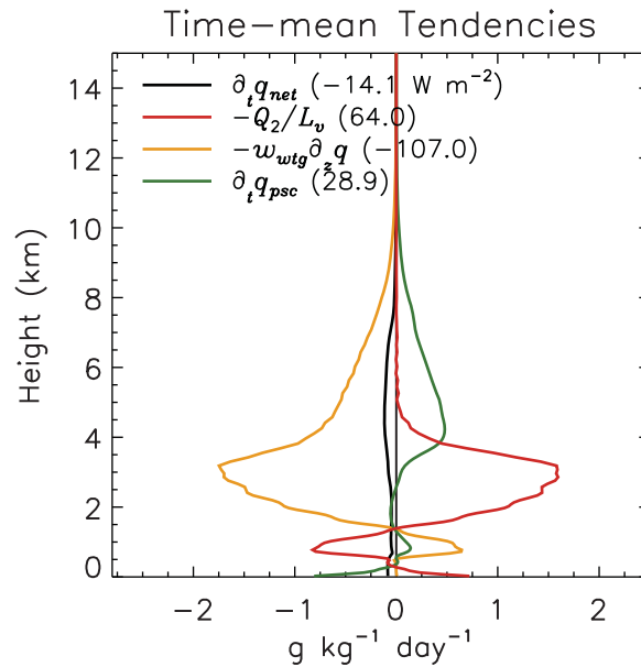
Figure 4. Moisture tendencies (in Eulerian form; see equation (3)) averaged over the fourth and fifth days of CTL, including the net source ( \partial_t q ; black), the convective source ( -Q_2/L_v ; red), the source due to vertical advection ( -w_{wtg} \partial_z q ; orange), and the constant prescribed source ( \partial_t q_{psc} ; green). Values in parentheses are the corresponding column-integrated values ( W m^{-2} ).
