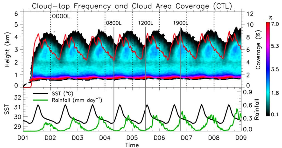
Figure 5. Time-height series from CTL of (top) cloud-top frequency (shaded; %) and cloud area coverage (right ordinate; red; %), and (bottom) SST (black; left ordinate; °C) and domain-averaged rainfall (green; right ordinate; mm d -1 ). The black-dashed line (top) indicates mixed-layer top, i.e., the level of minimum vertical eddy heat flux. The large abscissa ticks indicate 0000L, beginning with the simulation start at midnight on day 1 (D01). Three-point temporal boxcar smoothing has been applied to cloud-top frequency. The vertical gray-solid lines are provided for reference at the indicated times.
