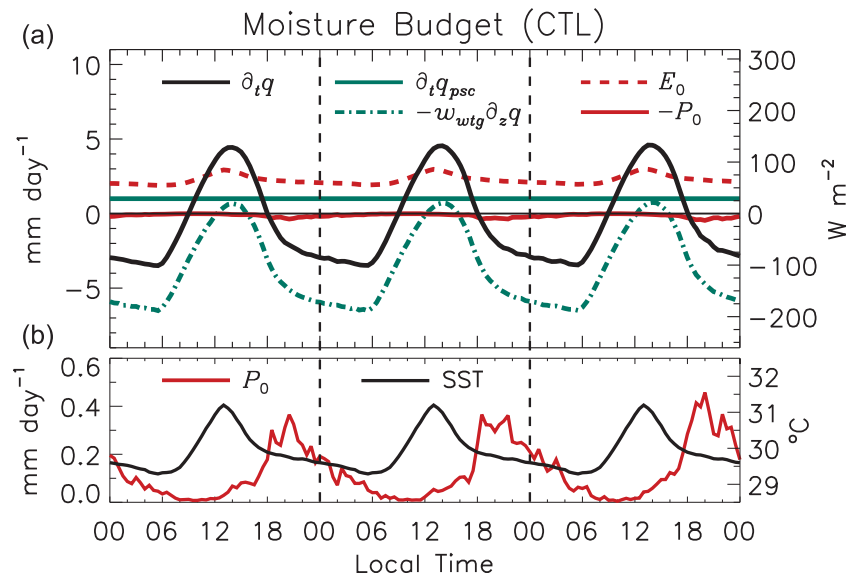
Figure 10. (a) Column-integrated moisture budget in the Eulerian framework for CTL, according to (3), with the local time-tendency ( \partial_t \bar{q} ; black), prescribed tendency ( \partial_t \bar{q}_{psc} ; turquoise-solid), vertical-advection tendency ( w_{wtg} \partial_z \bar{q} ; turquoise-dot-dashed), surface evaporation ( E_0 ; red-dashed), and the negative of surface precipitation ( -P_0 ; red-solid) (left ordinate: \text{mm d}^{-1} ); and (b) P_0 (repeated for detail; red; \text{mm d}^{-1} ; left ordinate) and SST (black; ^{\circ}\text{C} ; right ordinate). Multiplying terms in Figure 10a by L_v yields energy units (right ordinate; \text{W m}^{-2} ).
