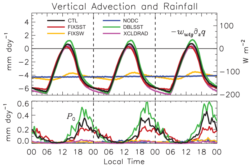
Figure 14. As in Figure 10 except only showing (top) w_{wtg} \partial_z q and (bottom) P_0 for each sensitivity test, as indicated in the legend.
