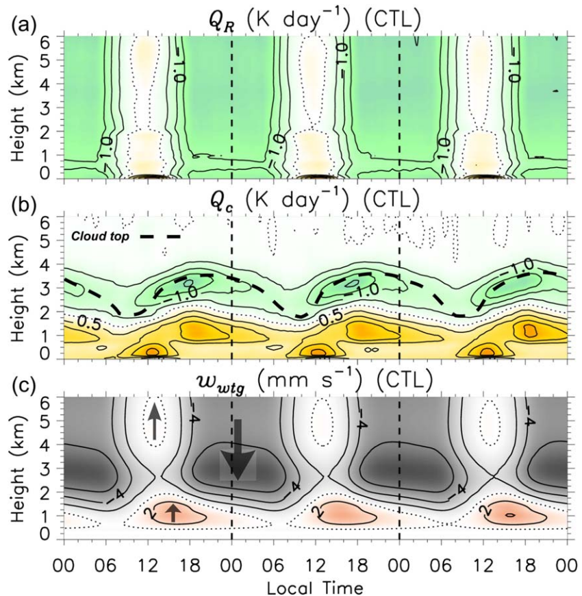
Figure 8. Time-height series of heat tendencies (see section 2.4) in CTL due to (a) total radiative heating Q_R and (b) convective heating Q_c (contoured every 0.5 \text{ K d}^{-1} ). Shown in (c) is w_{wtg} (contoured every 2 \text{ mm s}^{-1} ). Five-point boxcar smoothing has been applied to each variable in both time and height. The approximate cloud-top height (i.e., the upper 1.3% cloud-top frequency contour; Figure 5) is included in Figure 8b. The arrows in Figure 8c indicate the direction of w_{wtg} vertical motion. The zero-contour is dotted, here and henceforth. The time axis only spans D04–D07 for brevity and to emphasize detail in the diurnal cycle (here and henceforth).
