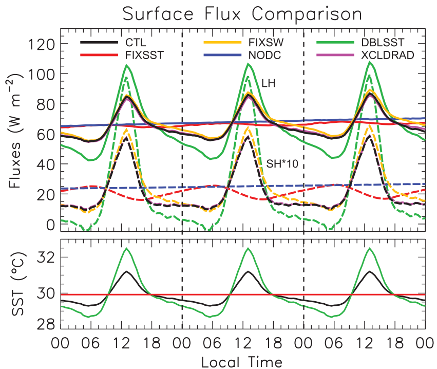
Figure 12. Surface LH (solid) and SH ( \times 10 ; dashed) (top; W m^{-2} ) and SST (bottom; ^{\circ}C ) for each sensitivity test, as indicated in the legend.
