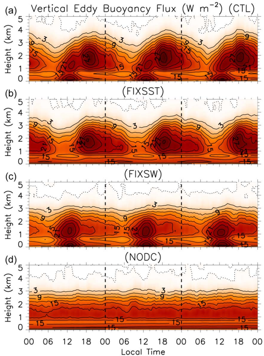
Figure 13. Vertical eddy buoyancy flux in (a) CTL, (b) FIXSST, (c) FIXSW, and (d) NODC (contoured every 3 \text{ W m}^{-2} ).
