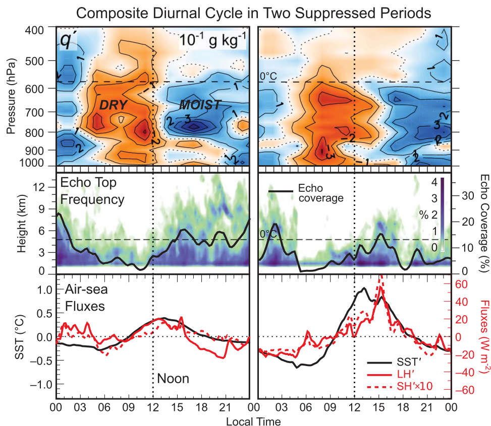
Figure 1. Composite diurnal cycle of shallow moist convection during the (left) October and (right) November MJO suppressed periods of the DYNAMO field experiment (Dynamics of the Madden-Julian Oscillation). (top) Water vapor mixing ratio q with the daily-mean removed ( q' ; every 10^{-1} \text{ g kg}^{-1} ); (middle) cloud echo-top frequency (shaded; %) and echo area coverage (solid line; %; right ordinate); and (bottom) sea surface temperature SST (black; ^{\circ}\text{C} ; left ordinate), latent heat flux LH (red-solid line; \text{W m}^{-2} ; right ordinate), and sensible heat flux \text{SH} \times 10 (red-dashed line; \text{W m}^{-2} ; right ordinate) with composite means removed (i.e., \text{SST}' , \text{LH}' , and \text{SH}' , respectively). Composite date ranges include 7–13 October and 11–16 November 2011, respectively. Modified from Ruppert and Johnson [2015], supplemental figure, copyright 2015, with permission from the American Meteorological Society.
