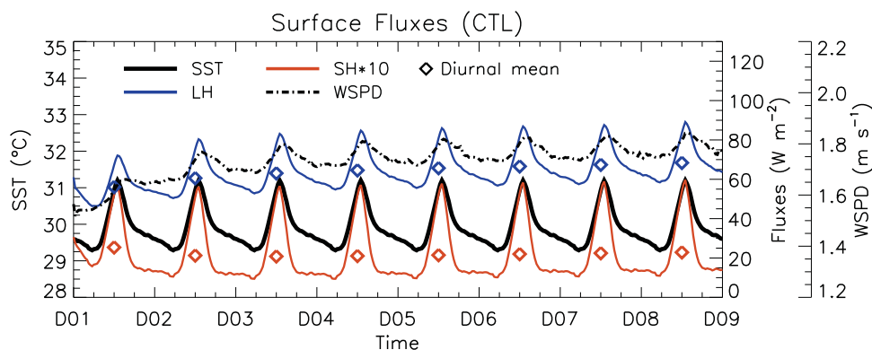
Figure 7. Time series from CTL of SST (black-solid; left ordinate; °C) and domain-averaged LH (blue) and SH×10 (red) (inner-right ordinate; \text{W m}^{-2} ) and wind speed (WSPD) at the lowest scalar level (25 m) (outer-right ordinate; black-dashed-dotted; \text{m s}^{-1} ). Open squares indicate the daily-mean (midnight-midnight) surface flux values, according to color.
