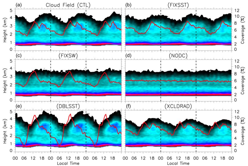
Figure 11. Cloud-top frequency (shaded; %; see Figure 5 for color bar) and cloud area coverage (right ordinate; red; %) in (a) CTL, (b) FIXSST, (c) FIXSW, (d) NODC, (e) DBLSST, and (f) XCLDRAD.
