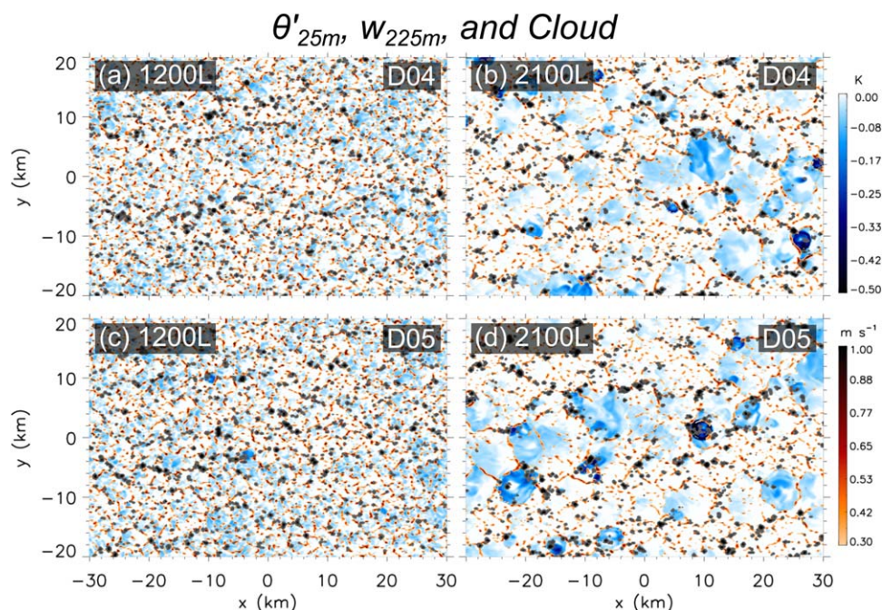
Figure 6. Potential temperature \theta at 25 m (i.e., the lowest scalar level) with the horizontal average removed ( \theta'_{25m} ; K; upper color bar), w at 225 m ( w_{225m} ; \text{m s}^{-1} ; lower color bar), and cloud (i.e., columns where total cloud-liquid water path exceeds 5 \times 10^{-3} mm; gray shading) from CTL at (a) 1200L and (b) 2100L D04, and (c) 1200L and (d) 2100L D05. No smoothing has been applied. About 50% of the total model domain is shown in each plot.
