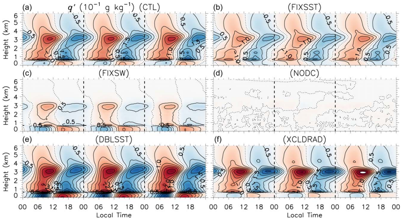
Figure 15. q' in (a) CTL, (b) FIXSST, (c) FIXSW, (d) NODC, (e) DBLSST, and (f) XCLDRAD (contoured every 0.5 \times 10^{-1} \text{ g kg}^{-1} ).
