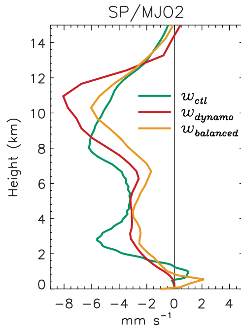
Figure 3. Large-scale vertical motion comparison: simulated w_{wtg} averaged over the second and third days of CTL (i.e. “ w_{ctl} ”); vertical motion from the DYNAMO northern sounding array averaged over SP/MJO2 (“ w_{dynamo} ”); and the vertical motion diagnosed from WTG balance using the apparent heat source Q_1 and static stability from DYNAMO during SP/MJO2 (i.e., “ w_{balanced} ”) ( \text{mm s}^{-1} ).
