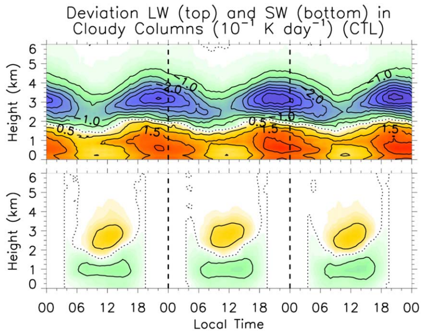
Figure 16. Deviation of (top) longwave (LW) and (bottom) shortwave (SW) radiative heating rates averaged over cloudy columns from their respective domain-averaged tendencies in CTL (contoured every 0.5 \times 10^{-1} \text{ K d}^{-1} ).
