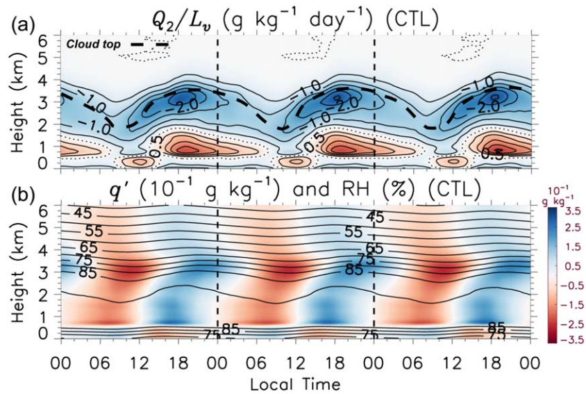
Figure 9. As in Figure 8 except with (a) Q_2/L_v (contoured every 0.5 g kg -1 d -1 ), and (b) q' (shaded according to the color bar; 10 -1 g kg -1 ) and relative humidity RH (contoured every 5%).
