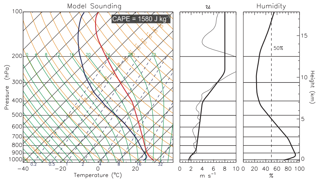
Figure 2. Model input sounding, based on the mean sounding from the DYNAMO–MJO2 suppressed phase (13–15 November 2011) from the R/V Revelle . (left) Skew T–logp diagram, (middle) zonal wind speed u ( \text{m s}^{-1} ), and (right) relative humidity RH (%; the vertical dashed line highlights the 50% level). CAPE (convective available potential energy; \text{J kg}^{-1} ) is indicated (left), as is observed wind speed from the R/V Revelle mean sounding (thin line in middle plot; smoothed with a 25 hPa running mean). Left and right ordinates are pressure (hPa) and height (km), respectively.
