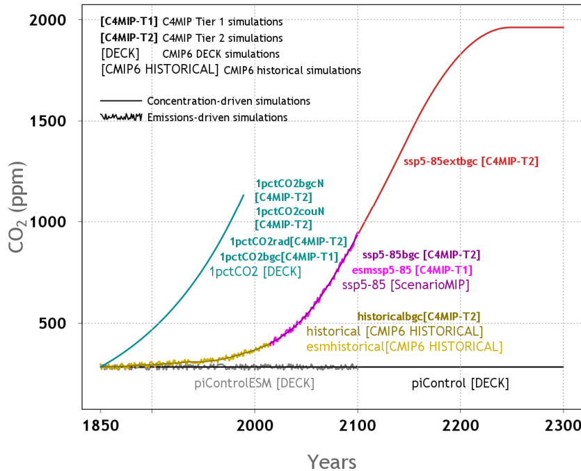
Figure 1: Relation of C4MIP simulations to CMIP6 DECK and historical simulations and the ssp5-85 future scenario simulation proposed for the ScenarioMIP.
