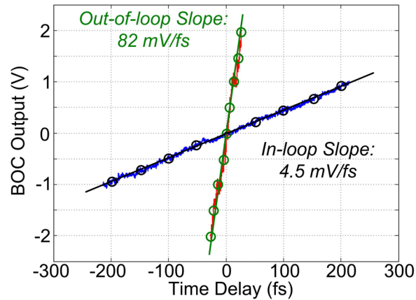
FIG. 5. Measurement results of the FC-BOC output versus the delay between the pulses. Blue curve corresponds to the in-loop and red curve corresponds to the out-of-loop FC-BOC response. Linear fits to five different measurements give average timing sensitivity of 4.5 mV/fs ( \pm 0.32 mV/fs) and 82 mV/fs ( \pm 4.9 mV/fs) for the in-loop and out-of-loop FC-BOC, respectively.
