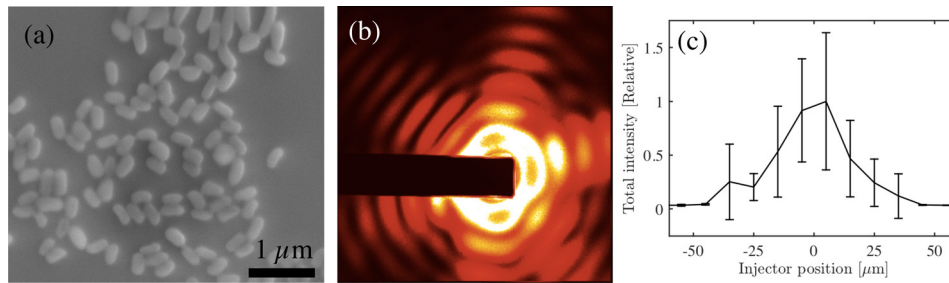
FIG. 5. (a) A scanning electron microscope image of granulevirus particles. (b) A single-shot diffraction pattern from an isolated granulevirus, isolated from the much greater number of aggregated particle clusters. (c) A plot of the average total diffracted x-ray photon counts as a function of injector position. Error bars indicate the standard deviation in each measurement.
