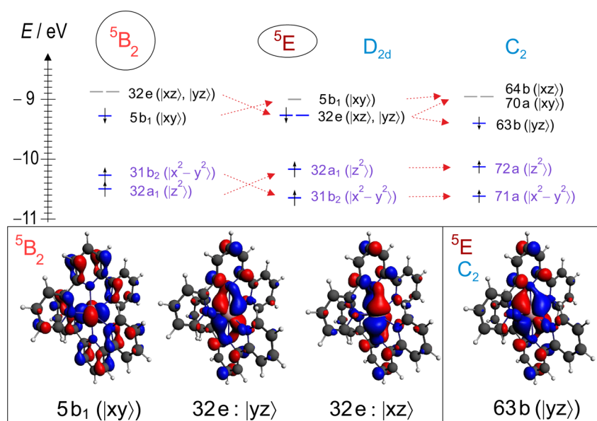
Figure 8. Diagram of the spin-unrestricted KS molecular orbitals for the quintet states of [\text{Fe}(\text{terpy})_2]^{2+} for {}^5E , and both the highly symmetric ( D_{2d} ) and the Jahn–Teller distorted ( C_2 ) form is also shown. (Note that in a rigorous description the latter should be denoted as {}^5B in C_2 symmetry.) The energy levels (top) as well as the 3D representation (bottom) of the most relevant MOs of the {}^5B_2 and {}^5E states with relevant 3d character are shown.
