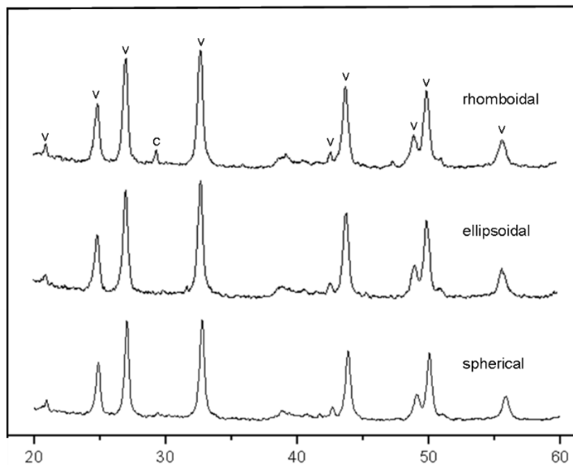
Figure S1. Powder X-ray diffraction analysis of rhomboidal, ellipsoidal, and spherical vaterite particles. C= calcite, V= vaterite.
