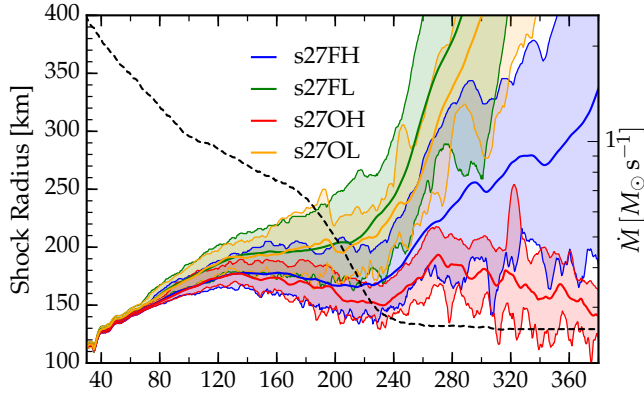
Figure 3. Evolution of the supernova shock. The thick lines show the angular average of the shock radius for all four models considered in this work. For the models s27FH, s27FL, and s27OH, the shaded regions show the minimum and maximum radius of the shock at a given time. The dashed line shows the mass accretion rate in s27OL just outside the shock. The accretion rates for the other three models are similar.
