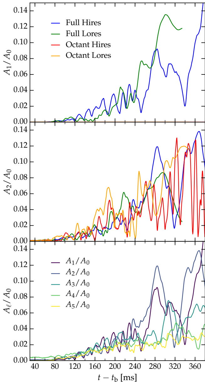
Figure 5. Evolution of the real spherical harmonic deformation of the supernova shock front. Top Panel: The rms m modes of the \ell = 1 spherical harmonic normalized to the \ell = 0 , m = 0 mode. Octant symmetry forces all \ell = 0 modes to be zero. Middle Panel: Similar to the top panel, except for the \ell = 2 mode. Bottom Panel: Evolution of the first five \ell -modes of s27FH.
