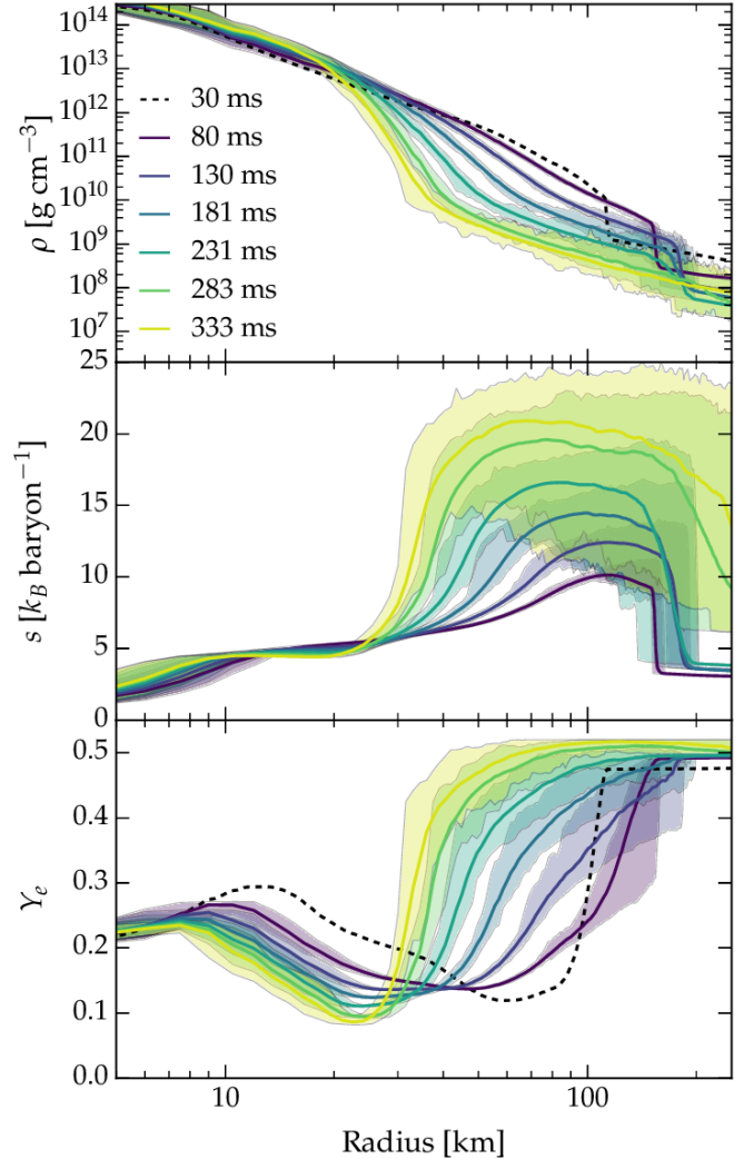
Figure 2. Evolution of the thermodynamic state of the gain region of s27FH. The solid lines show the angle averaged density, entropy, and electron fraction of the ejecta, while the shaded regions show the minimum and maximum of these quantities on spherical shells. The dashed lines show the initial conditions of our 3D simulations.
