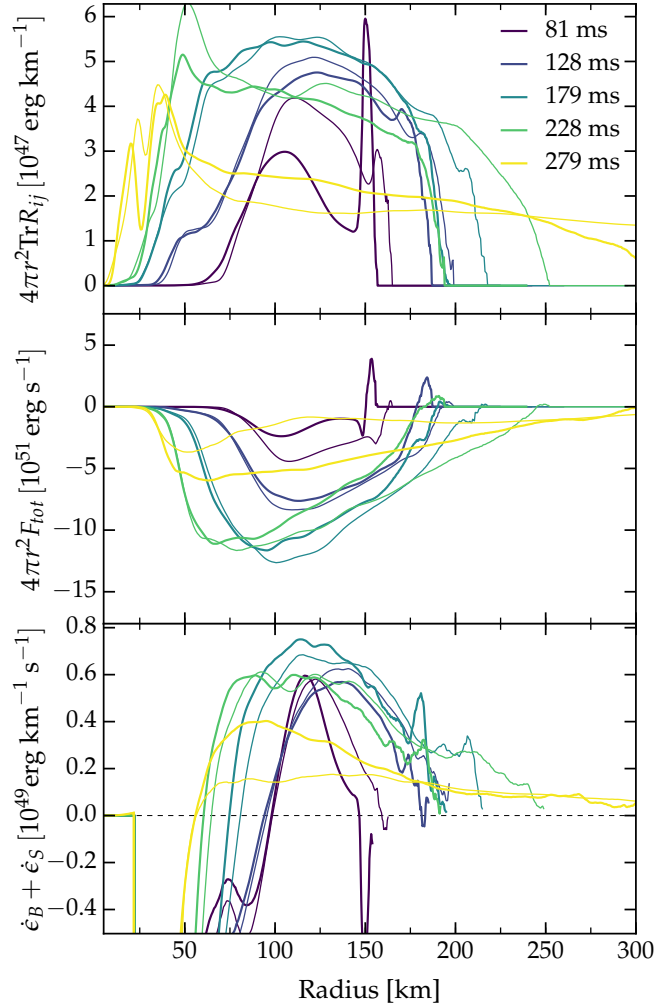
Figure 9. The trace of the Reynolds stress and related quantities versus radius at various times in s27FH (thick lines) and s27FL (thin lines). Top Panel: The trace of the Reynolds stress integrated over angle. Middle Panel: The total flux of the trace of the Reynolds stress. Throughout most of the gain region, the flux is dominated by the average velocity advection term. Near the shock, both pressure fluctuations and turbulent convection significantly contribute. Bottom Panel: The Reynolds production by buoyancy and shear. Buoyancy is the dominant contributor throughout most of the gain region, but the shear term contributes significantly near the shock.
