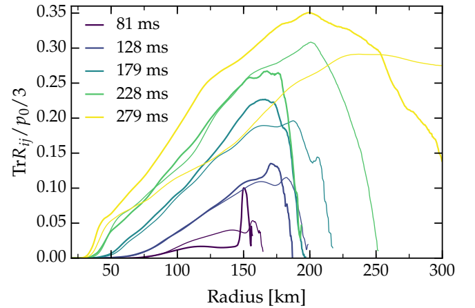
Figure 8. The ratio of the Reynolds pressure (i.e. \text{Tr}R_{ij}/3 ) to the average thermal pressure in the gain region. The ratio as a function of radius is shown at various times in s27FH (thick lines) and s27FL (thin lines). Comparing with the rr component of the Reynolds stress gives similar results, although the maximum of R_{rr}/p_0 \approx 0.5 .
