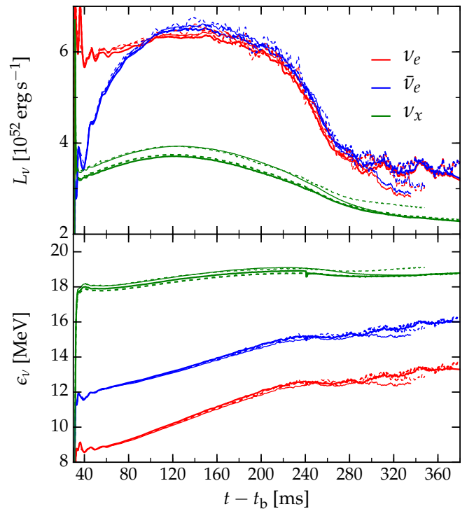
Figure 6. Spherically averaged properties of the neutrino field at a radius of 450 km for the models s27FH (thick solid lines), s27FL (thin solid lines), s27OH (thick dashed lines), and s27OL (thin dashed lines). The top panel shows the \nu_e (red lines), \bar{\nu}_e (blue lines), and \nu_x (green lines) luminosities as functions of time. The luminosities of s27OH are indistinguishable from those of the model s27FH for the first 280 ms. The lower panel shows mean neutrino energies as a function of time.
