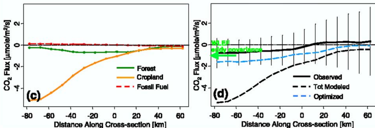
Figure 6. Same as Figure 4, but for the WI#2 experiment. The arrow in light green in Figure 6d refers to the observed \text{CO}_2 flux from eddy covariance at WLEF for the same period between 22 and 23 August.
