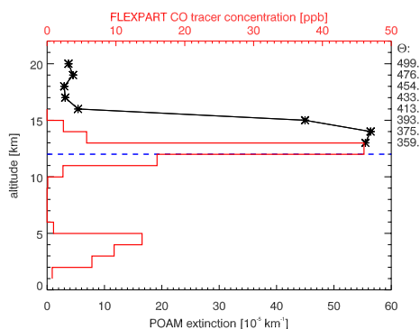
Figure 5. POAM III satellite extinction measurements above James Bay ( 54^{\circ}\text{N} , 102^{\circ}\text{W} ) on June 29 at 01:57 UTC. Dashed blue line represents tropopause at POAM location. The red line represents predicted CO at the POAM location from the FLEXPART model.
