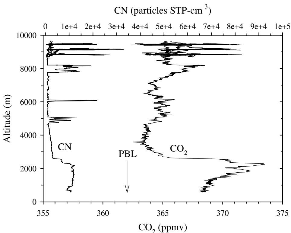
Figure 18. Vertical profile of CN (left) and CO 2 (right) as observed on 21 July. The planetary boundary layer (PBL) is discernible by high mixing ratios of CO 2 and a high CN concentration (below 2.6 km; ground at 0.6 km altitude).
