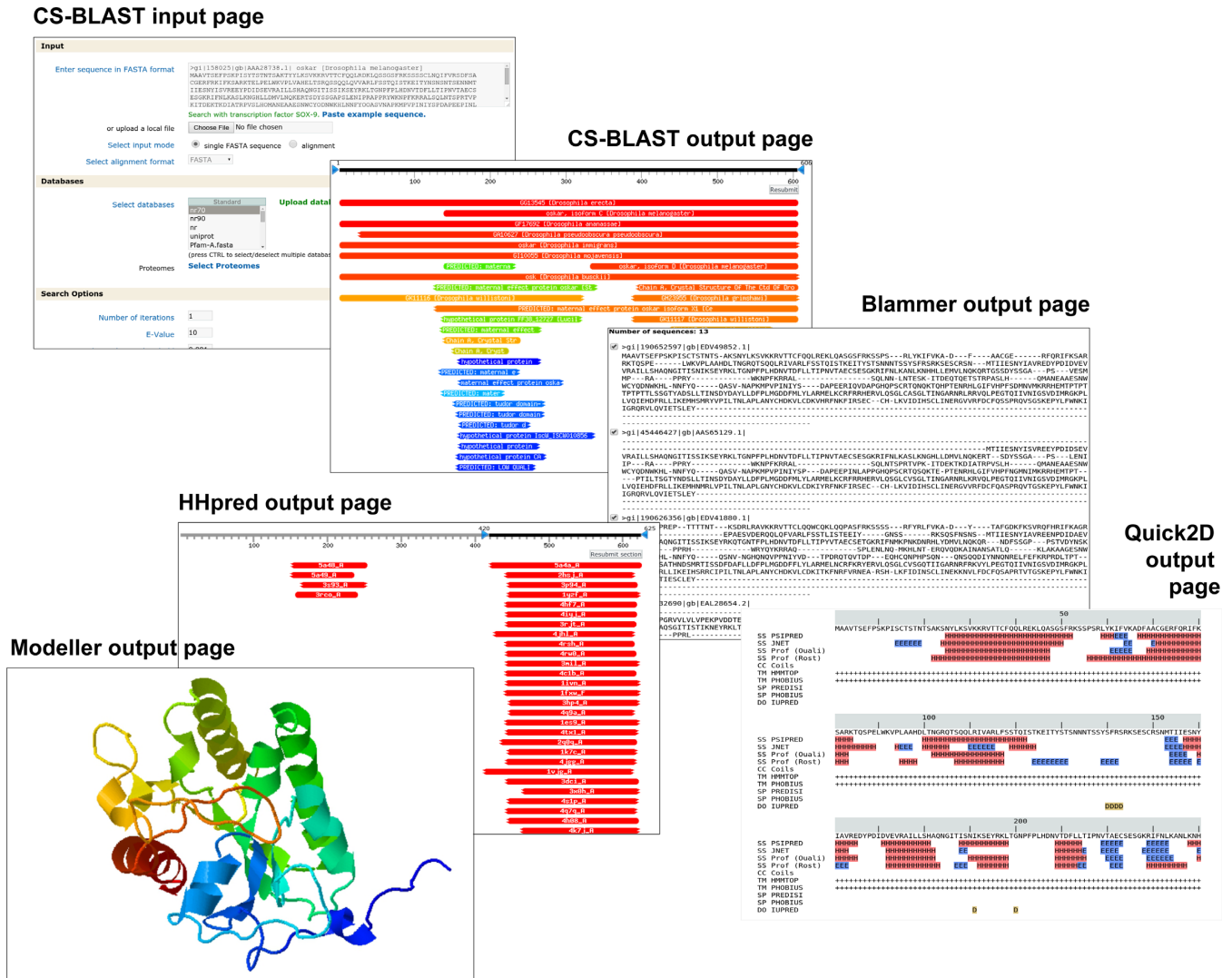
Figure 2. Interconnection of the tools in the Toolkit. The output of most tools can be forwarded as input to many other tools. One such possible forwarding pipeline is shown, wherein the output of the sensitive search method CS-BLAST is forwarded to Blammer to parse out a multiple alignment, which is subsequently forwarded to Quick2D for secondary structure prediction and HHpred for the identification of remote homologs. The output of HHpred is then forwarded to Modeller in order to obtain a structural model.
