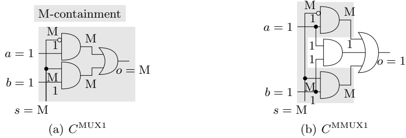
Figure 5: Multiplexer behavior for a = b = 1 , in which case the output should be 1, regardless of the select bit s . For s = M , however, the standard multiplexer (a) can become metastable, but the metastability-containing multiplexer (b) outputs 1.
