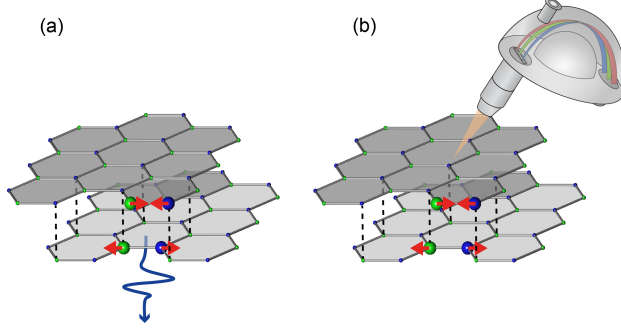
FIG. 1: The effects of resonant excitation of the in-plane E_{1u} mode in bilayer graphene (the atomic motions are indicated by red arrows) are investigated with TeraHertz time-domain spectroscopy (a) and time-and angle-resolved photoemission spectroscopy (b).
