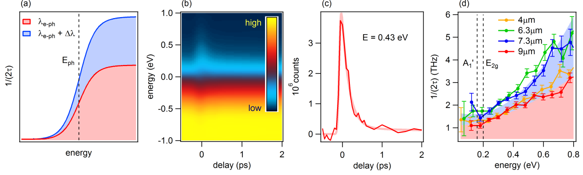
FIG. 3: (a) Expected increase of the energy-resolved relaxation rate due to a pump-induced enhancement of \lambda_{e-ph} . (b) Momentum-integrated photocurrent measured along the \Gamma K -direction in the vicinity of the K-point as a function of pump-probe delay after excitation at \lambda_{pump} = 6.3 \mu m . These experiments were performed at 30 K with energy and temporal resolutions of 600 meV and 100 fs, respectively. (c) Lineouts at constant energy (here E = 0.43 eV) are fitted with an exponential decay to obtain the energy-dependent relaxation time \tau . (d) Relaxation rate 1/(2\tau) as a function of energy for different pump wavelengths in the mid-infrared. For \lambda_{pump} = 6.3 \mu m and 7.3 \mu m (at resonance with the E_{1u} phonon) the energy-integrated relaxation rate is enhanced, indicating an increase of the electron-phonon coupling constant \lambda_{e-ph} .
