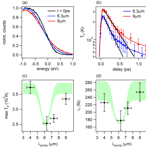
FIG. 4: (a) Momentum-integrated photocurrent as a function of energy at negative delay (black) and at the peak of the pump-probe signal for \lambda_{pump} = 6.3 \mu m (on-resonance, blue) and \lambda_{pump} = 9 \mu m (off-resonance, red) together with Fermi-Dirac fits. (b) Electronic temperature as a function of pump-probe delay for \lambda_{pump} = 6.3 \mu m (blue) and \lambda_{pump} = 9 \mu m (red) together with double-exponential fits. Black lines illustrate the difference in the fast time constant between on- and off-resonance excitation. Electronic peak temperature (c) and fast relaxation time (d) as a function of pump wavelength (data points) together with a simulation based on a two-temperature model (green lines). The width of the green lines represents the experimental uncertainty in \lambda_{e-ph} .
