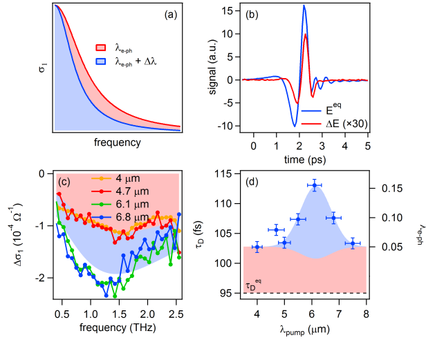
FIG. 2: (a) An increase of the electron-phonon coupling constant \lambda_{e-ph} is predicted to enhance the scattering time and thus reduce the width of the Drude peak in the real part of the optical conductivity. (b) Transmitted electric THz field without pump (blue) and pump-induced changes of the field at the peak of the pump-probe signal for \lambda_{pump} = 6.1 \mu m . (c) Pump-induced changes of the real part of the optical conductivity as a function of energy for different pump wavelengths in the mid-infrared together with Drude fits. (d) Drude scattering time (left axis) and electron phonon-coupling constant (right axis) as a function of pump wavelength. The red(blue)-shaded area indicates the increase in \tau_D due to heating (an enhanced \lambda_{e-ph} ). The black dashed line indicates the equilibrium value of \tau_D .
