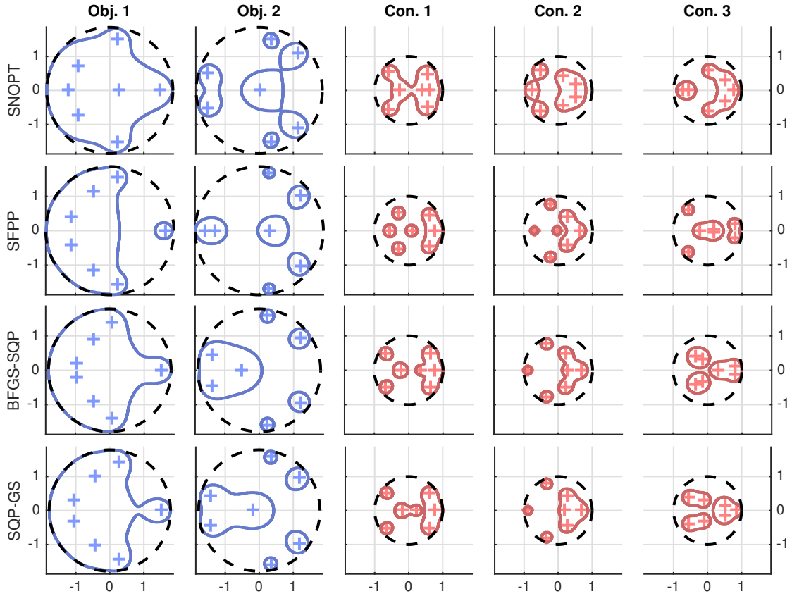
Figure 15: The four rows show the final pseudospectral configurations for the four controllers found by SNOPT, SFPP, BFGS-SQP, and SQP-GS (top to bottom) for the problem described in Figure 14. The left two columns indicate the plants in the objective while the right three columns indicate the plants in the constraint, with the plus signs indicating the eigenvalues. On the objective plots, the dashed black circle corresponds to the max pseudospectral radius of the two plants in the objective for that particular algorithm's controller. The dashed black circle on the plots for constraints is the unit circle (the stability boundary). The solid lighter circles indicate the pseudospectral boundaries of each plant.
