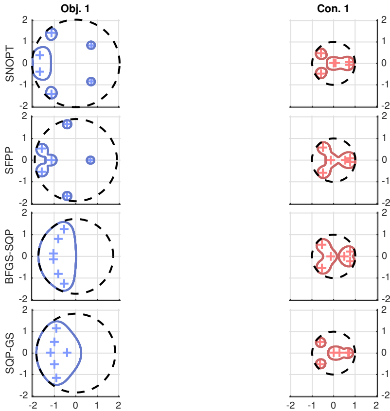
Figure 13: The four rows show the final pseudospectral configurations for the four controllers found by SNOPT, SFPP, BFGS-SQP, and SQP-GS (top to bottom) for the problem described in Figure 12. The left column indicates the single plant in the objective while the right column indicates the single plant in the constraint, with the plus signs indicating the eigenvalues. On the objective plots, the dashed black circle corresponds to the pseudospectral radius of the plant in the objective for that particular algorithm's controller. The dashed black circle on the plots for constraints is the unit circle (the stability boundary). The solid lighter circles indicate the pseudospectral boundaries of each plant.
