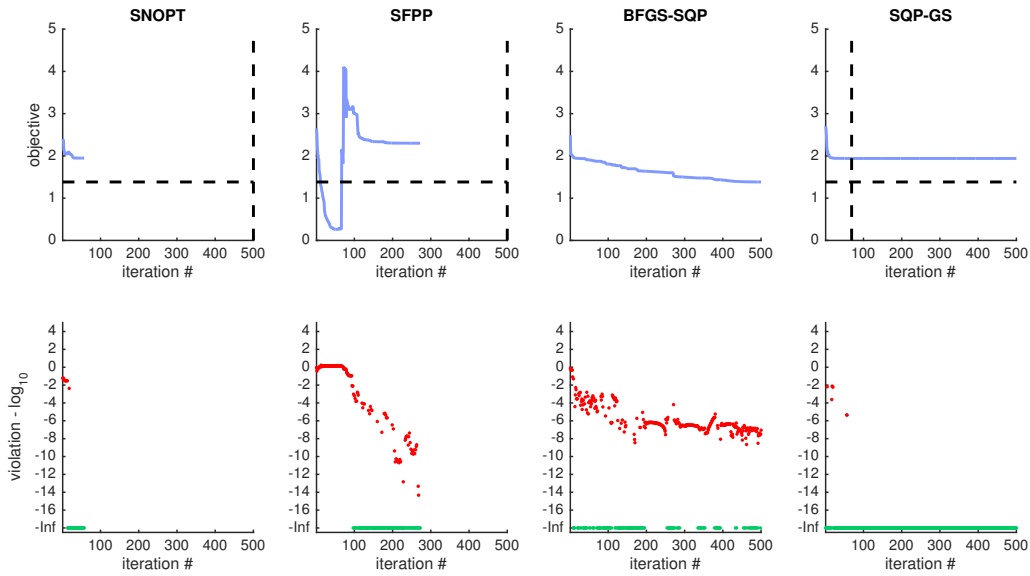
Figure 8: The plots in the top row track the value of the spectral-radius-based objective function in terms of iteration number for SNOPT, SFPP, BFGS-SQP, and SQP-GS (left to right) on a randomly generated example of dimension N = 5 comprised of one plant in the objective and one in the constraint and where the controller matrix has MP = 4 \times 2 = 8 variables. In the top row of plots, the vertical dashed line indicates the iteration number whose elapsed CPU-time was closest to BFGS-SQP total elapsed CPU-time while the horizontal dashed line indicates the value of BFGS-SQP's best feasible solution. The \log_{10} -scaled plots in the bottom row show the amount of violation tracking with the iteration counts with “-Inf” indicating zero violation (feasible points).
