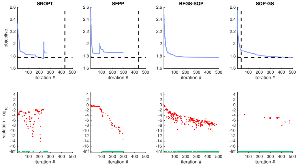
Figure 14: The plots in the top row track the value of the pseudospectral-radius-based objective function in terms of iteration number for SNOPT, SFPP, BFGS-SQP, and SQP-GS (left to right) on a randomly generated example of dimension N = 7 comprised of two plants in the objective and three in the constraint and where the controller matrix has MP = 5 \times 4 = 20 variables. In the top row of plots, the vertical dashed line indicates the iteration number whose elapsed CPU-time was closest to BFGS-SQP total elapsed CPU-time while the horizontal dashed line indicates the value of BFGS-SQP's best feasible solution. The log 10 -scaled plots in the bottom row show the amount of violation tracking with the iteration counts with “-Inf” indicating zero violation (feasible points).
