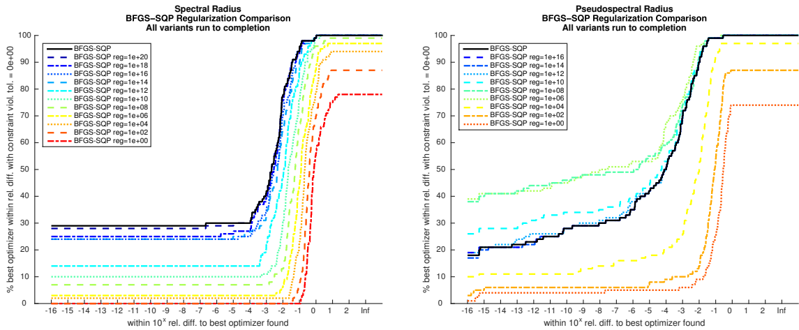
Figure 7: Left: the spectral radius test set. Right: the pseudospectral radius test set. Both RMPs show how the performance of BFGS-SQP changes over the test sets when increasing amount of regularization is applied to the inverse of the Hessian approximation.
