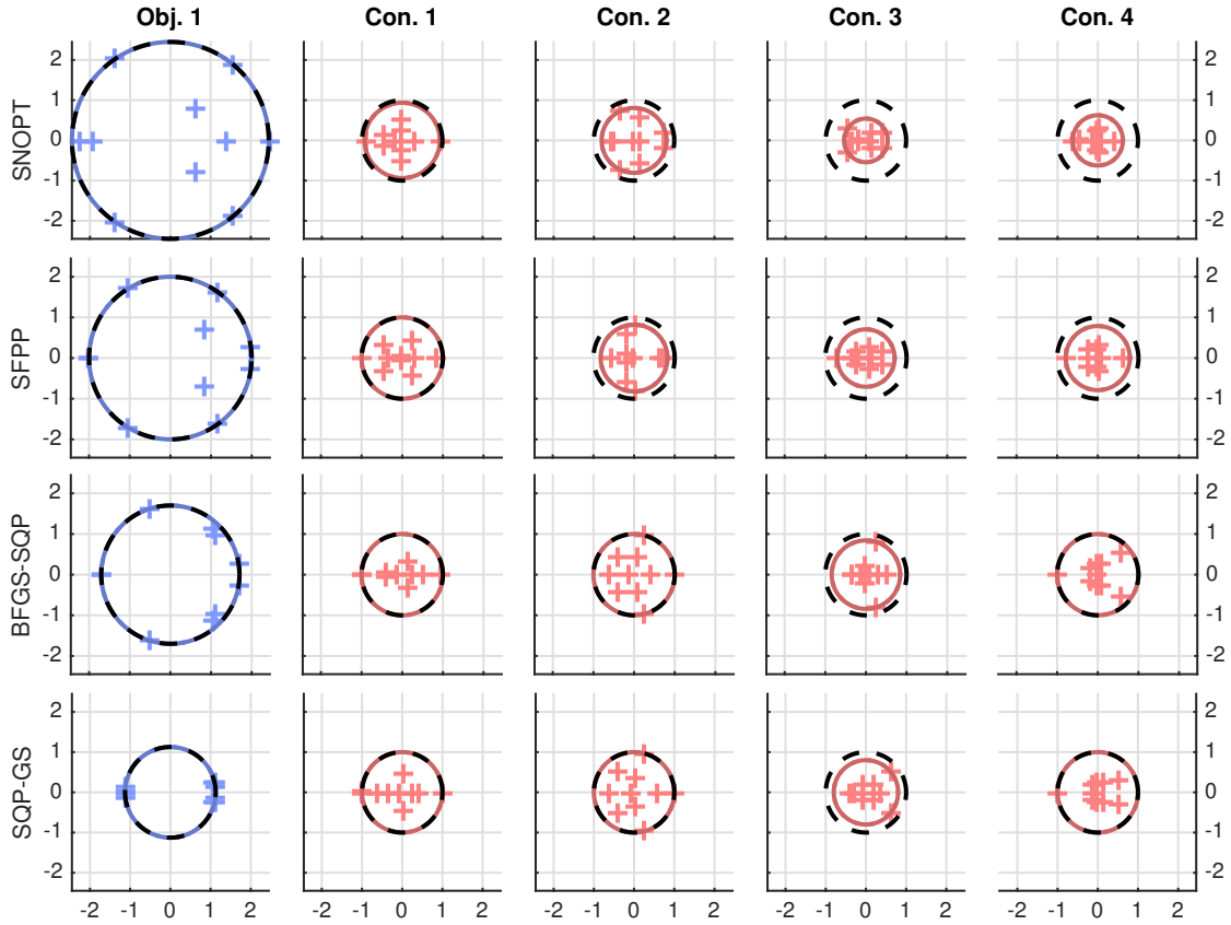
Figure 11: The four rows show the final spectral configurations for the four controllers found by SNOPT, SFPP, BFGS-SQP, and SQP-GS (top to bottom) for the problem described in Figure 10. The left column indicates the single plant in the objective while the right four columns indicate the plants in the constraint, with the plus signs indicating the eigenvalues. On the objective plots, the dashed black circle corresponds to the spectral radius of the plant in the objective for that particular algorithm's controller. The dashed black circle on the plots for constraints is the unit circle (the stability boundary). The solid lighter circles indicate the spectral radius of each plant.
