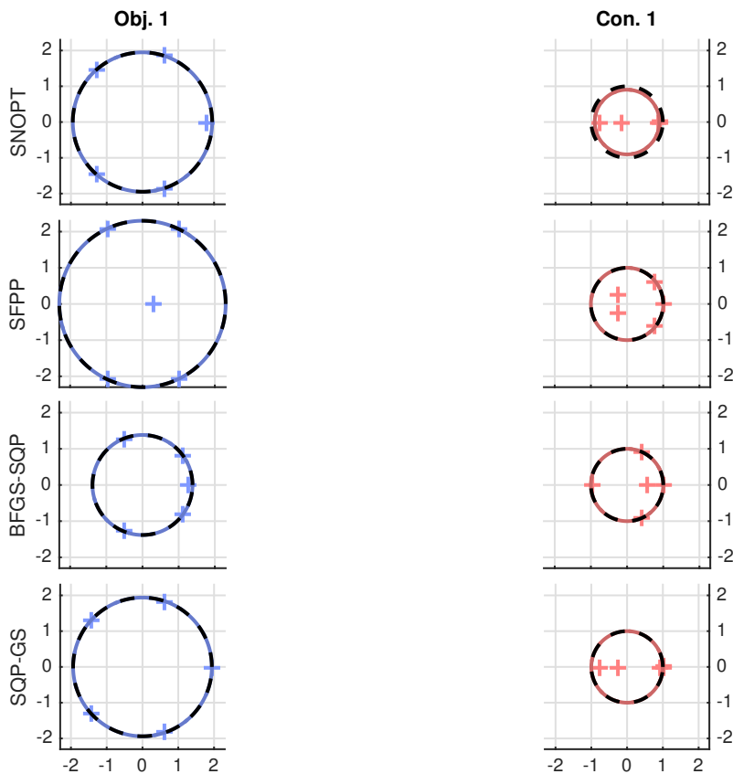
Figure 9: The four rows show the final spectral configurations for the four controllers found by SNOPT, SFPP, BFGS-SQP, and SQP-GS (top to bottom) for the problem described in Figure 8. The left column indicates the single plant in the objective while the right column indicates the single plant in the constraint, with the plus signs indicating the eigenvalues. On the objective plots, the dashed black circle corresponds to the spectral radius of the plant in the objective for that particular algorithm's controller. The dashed black circle on the plots for constraints is the unit circle (the stability boundary). The solid lighter circles indicate the spectral radius of each plant.
