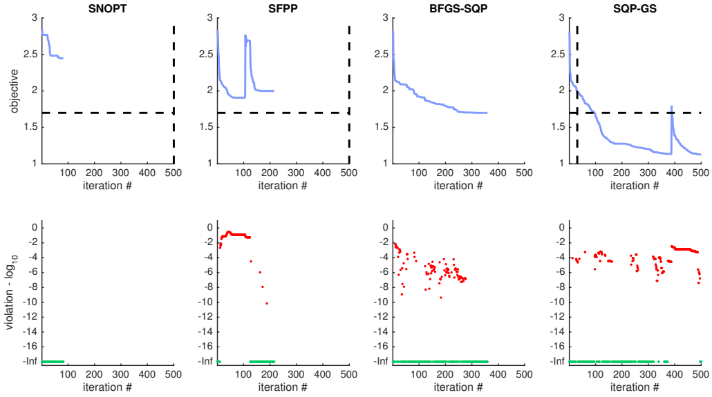
Figure 10: The plots in the top row track the value of the spectral-radius-based objective function in terms of iteration number for SNOPT, SFPP, BFGS-SQP, and SQP-GS (left to right) on a randomly generated example of dimension N = 10 comprised of one plant in the objective and four in the constraint and where the controller matrix has MP = 16 \times 1 = 16 variables. In the top row of plots, the vertical dashed line indicates the iteration number whose elapsed CPU-time was closest to BFGS-SQP total elapsed CPU-time while the horizontal dashed line indicates the value of BFGS-SQP's best feasible solution. The \log_{10} -scaled plots in the bottom row show the amount of violation tracking with the iteration counts with “-Inf” indicating zero violation (feasible points).
