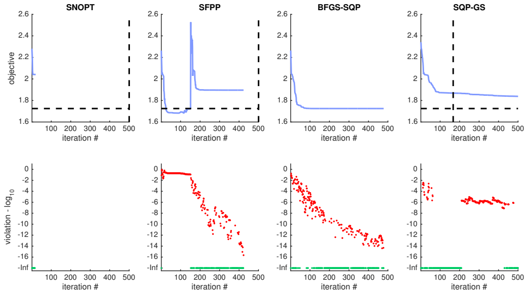
Figure 12: The plots in the top row track the value of the pseudospectral-radius-based objective function in terms of iteration number for SNOPT, SFPP, BFGS-SQP, and SQP-GS (left to right) on a randomly generated example of dimension N = 6 comprised of one plant in the objective and one in the constraint and where the controller matrix has MP = 7 \times 1 = 7 variables. In the top row of plots, the vertical dashed line indicates the iteration number whose elapsed CPU-time was closest to BFGS-SQP total elapsed CPU-time while the horizontal dashed line indicates the value of BFGS-SQP's best feasible solution. The \log_{10} -scaled plots in the bottom row show the amount of violation tracking with the iteration counts with “-Inf” indicating zero violation (feasible points).
