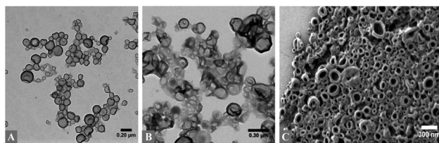
Fig. 2 TEM micrographs of the desilylated nanocapsules prepared via a surfactant-free emulsion-solvent evaporation technique with A: P(S 0.87 - stat -TMSMA 0.13 ), B: P(S 0.71 - stat -TMSMA 0.29 ). C: SEM micrograph of the P(S 0.87 - stat -TMSMA 0.13 ) nanocapsules with encapsulated dicyclopentadiene.
