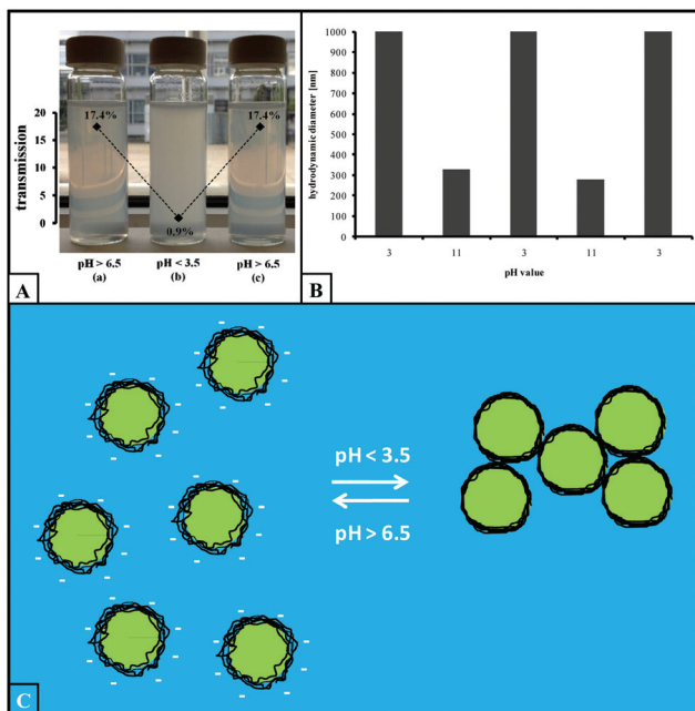
Fig. 3 The destabilization and redispersion of the P(S 0.71 -stat-TMSMA 0.29 ) nanocapsules can be monitored visually and by turbidimetry (A), and by DLS (B). C: Schematics of the aggregation–redispersion of the nanocapsule dispersion upon switching of the pH value.
