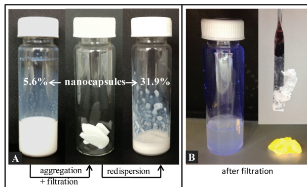
Fig. 4 The aggregation and subsequent redispersion allow increasing the concentration of the P(S 0.71 -stat-TMSMA 0.29 ) nanocapsules in water (A). The nanocapsules can be used to encapsulate organic molecules, for instance a fluorescent dye. After pH-triggered aggregation, the dye is present in the residue as identified by irradiating ( \lambda = 366 nm) the filtrate and the residue (B). The inset shows the appearance of the residue under normal sunlight.
