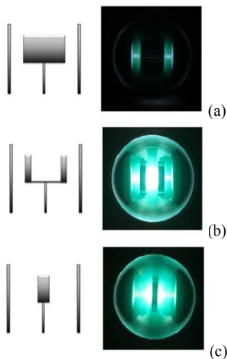
FIG. 2. Anode design schematics (not to scale) and pictures taken with a 20 MP camera of the (a) NSTX-U anode, (b) double ring anode, and (c) single ring anode. Magnetic field is horizontal for this view.
