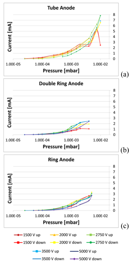
FIG. 3. Measured ion current at the cathode for the (a) NSTX-U anode, (b) double ring anode, and (c) single ring anode at various voltages while sweeping the pressure up and down.
