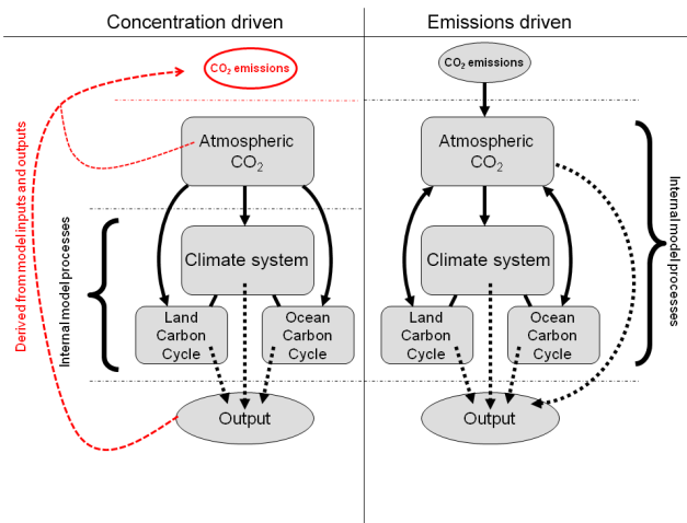
Figure 2. Schematic representation of carbon cycle numerical experimental design. Concentration-driven (left) and emissions-driven (right) simulation experiments make use of the same Earth system models (ESMs), but configured differently. Concentration-driven simulations prescribe atmospheric CO 2 as a pre-defined input to the climate and carbon cycle model components. Compatible emissions can be calculated from the output of the concentration-driven simulations. Emissions-driven simulations prescribe CO 2 emissions as the input, and atmospheric CO 2 is an internally calculated state variable within the ESM. Adapted from Ciais et al. (2013). Solid arrows depict internal data flow within the model, dashed arrows depict data output from the model.
