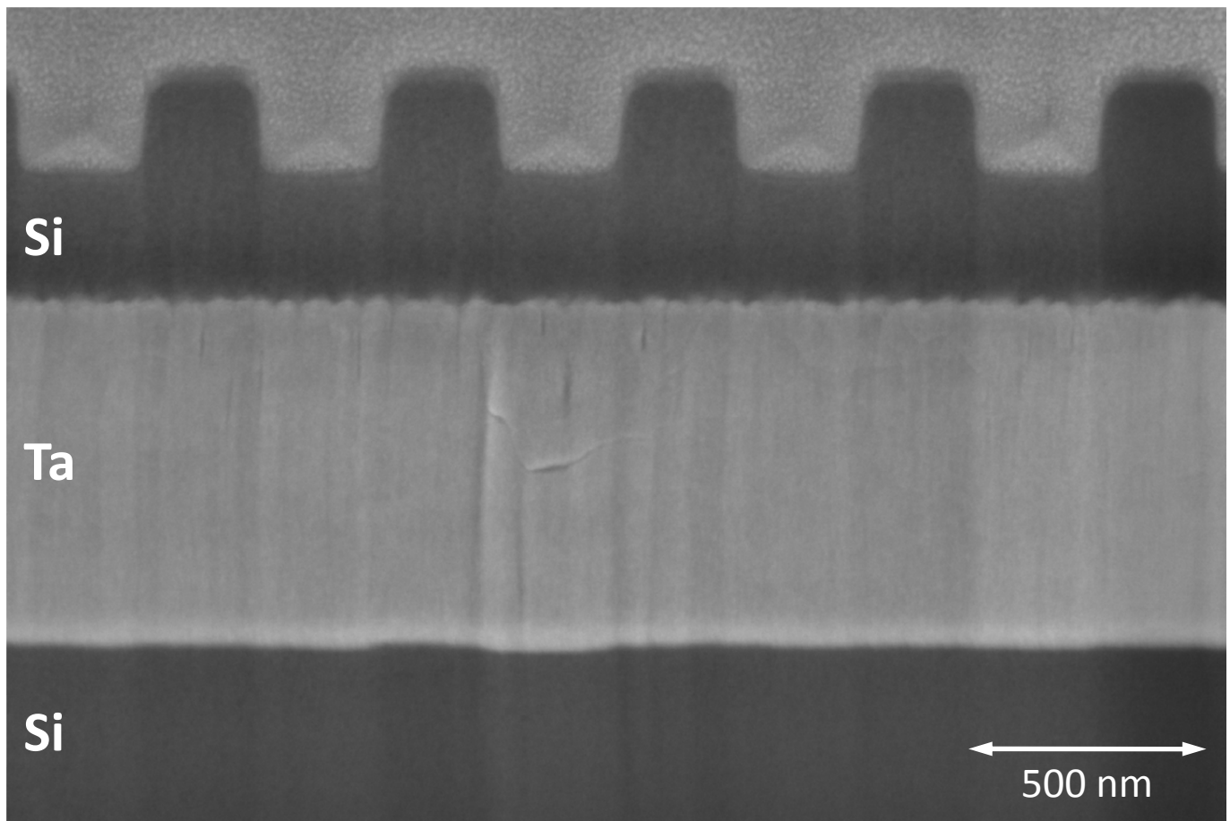
Fig. 1: Focused ion beam cross-section through the silicon grating sample consisting of a structured silicon layer on top of a tantalum interlayer on top of silicon substrate.
