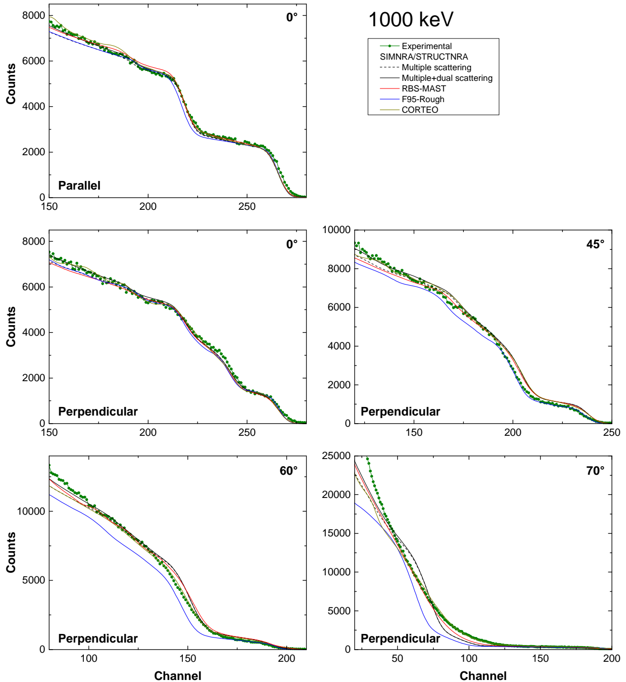
Fig. 7: Experimental and simulated backscattering spectra from the silicon grating shown in Fig. 1 using 1000 keV ^4\text{He} ions at incident angles from 0^\circ to 70^\circ . Top left: Parallel orientation of the grating at 0^\circ , see Fig. 2 left. All other: Perpendicular orientation of the grating. The angle of incidence is indicated. Green symbols: Experimental data; Dashed black lines: SIMNRA/STRUCTNRA with multiple small-angle scattering; Solid black lines: SIMNRA/STRUCTNRA with multiple small-angle scattering plus dual scattering; Solid red line: RBS-MAST; Solid blue line: F95-Rough; Solid yellow lines: CORTEO.
