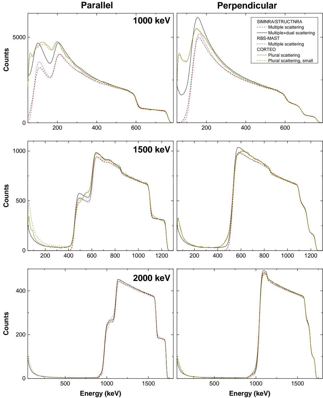
Fig. 5: Simulated spectra for 1000, 1500 and 2000 keV ^4\text{He} backscattered at normal incidence from the Si/Ta target shown in Fig. 3 including multiple and plural scattering. Left column: Parallel orientation of the grating, see Fig. 2 left; Right column: Perpendicular orientation, see Fig. 2 right. Top row: 1000 keV incident energy; Middle row: 1500 keV; Bottom row: 2000 keV. Dashed black lines: SIMNRA/STRUCTNRA using multiple small-angle scattering induced energy spread; Solid black lines: SIMNRA/STRUCTNRA using multiple small-angle scattering induced energy spread plus dual scattering; Dashed red lines: RBS-MAST using multiple small-angle scattering induced energy spread; Solid yellow lines: CORTEO using all plural scattering contributions; Dashed yellow lines: CORTEO using all plural scattering contributions with a smaller detector.
