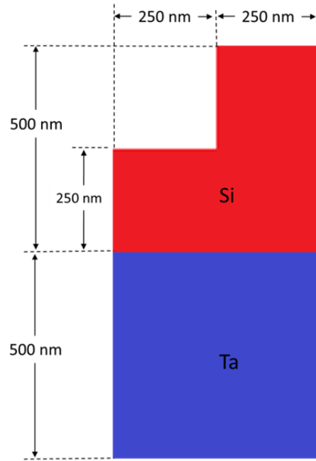
Fig. 3: Idealized sample structure used for the code-code comparison. The sample has periodic boundary conditions in horizontal direction, Si and Ta have natural mass densities.
