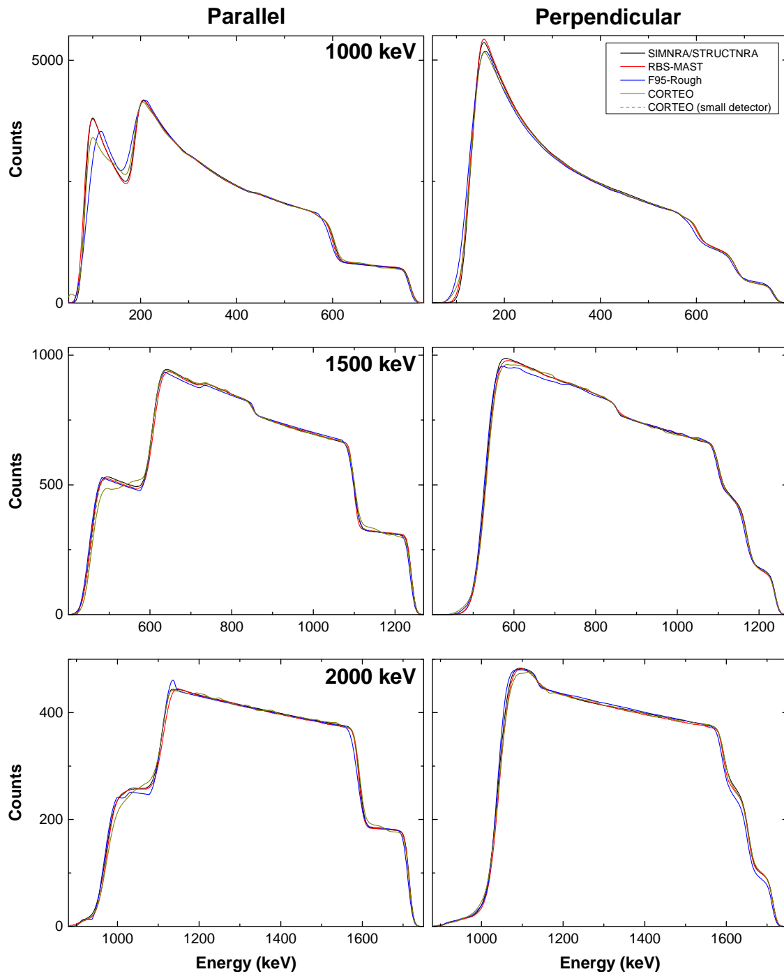
Fig. 4: Simulated spectra for 1000, 1500 and 2000 keV ^4\text{He} backscattered at normal incidence from the Si/Ta target shown in Fig. 3 in single-scattering approximation. Left column: Parallel orientation of the grating, see Fig. 2 left; Right column: Perpendicular orientation, see Fig. 2 right. Top row: 1000 keV incident energy; Middle row: 1500 keV; Bottom row: 2000 keV. Solid black lines: SIMNRA/STRUCTNRA; Solid red lines: RBS-MAST; Solid blue lines: F95-Rough; Solid yellow lines: CORTEO using single scattering and large detector; Dashed yellow line: CORTEO using single scattering and small detector (only for 1500 keV parallel orientation).
