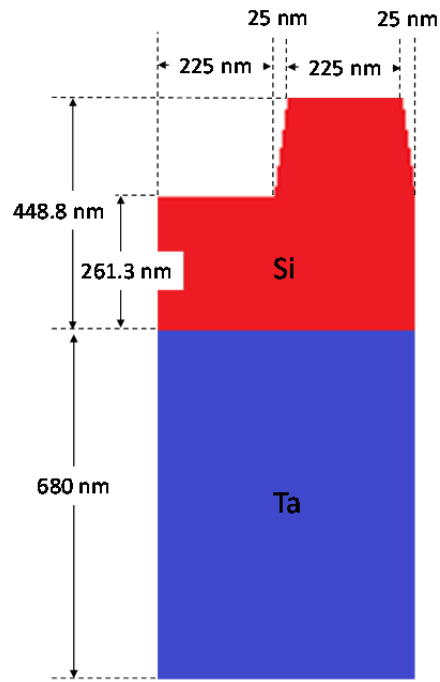
Fig. 6: Sample used for the comparison to experimental data. The sample has periodic boundary conditions in horizontal direction, Si and Ta have natural mass densities.
