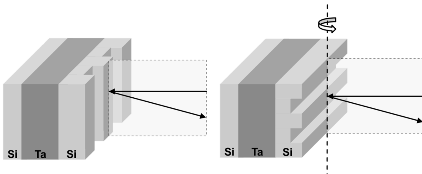
Fig. 2: Geometry of the measurements with the grating parallel to the plane formed by incident and exit beams (left) and perpendicular to this plane (right). The thick dashed line is the rotation axis of the sample for measurements at oblique incidence.
