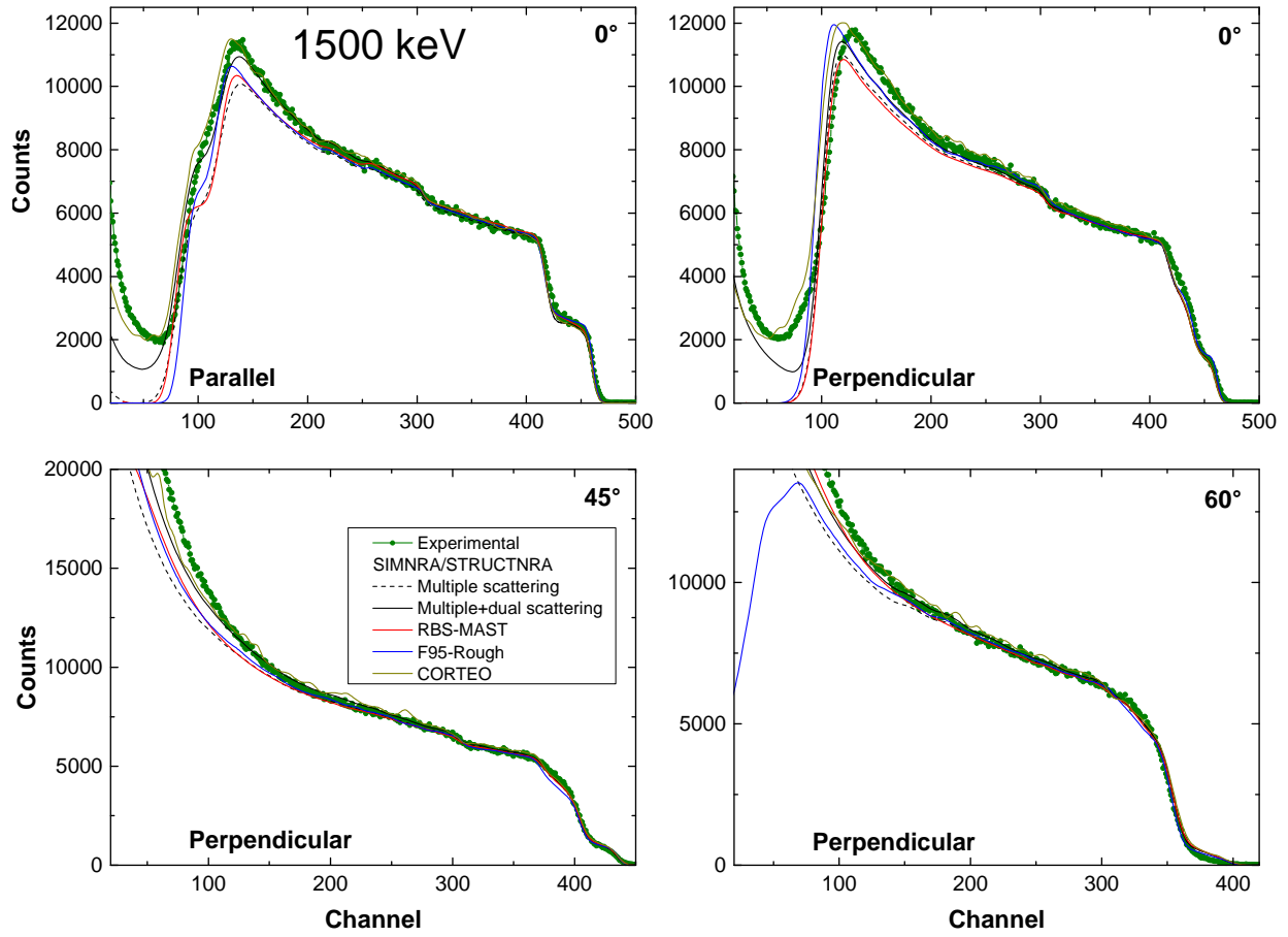
Fig. 8: Experimental and simulated backscattering spectra from the silicon grating shown in Fig. 1 using 1500 keV ^4\text{He} ions at incident angles from 0^\circ to 60^\circ . Top left: Parallel orientation of the grating at 0^\circ , see Fig. 2 left. All other: Perpendicular orientation of the grating. The angle of incidence is indicated. Green symbols: Experimental data; Dashed black lines: SIMNRA/STRUCTNRA with multiple small-angle scattering; Solid black lines: SIMNRA/STRUCTNRA with multiple small-angle scattering plus dual scattering; Solid red line: RBS-MAST; Solid blue line: F95-Rough; Solid yellow lines: CORTEO.
