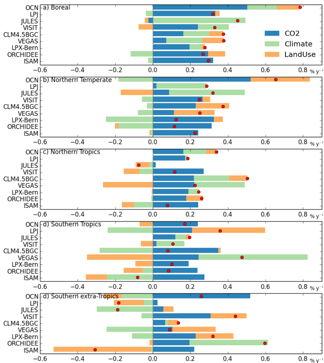
5 Figure 6. Attribution of the seasonal amplitude trend of regional (boreal (50-90N), Northern temperate (23.5-50N), Northern tropics (0-23.5N), Southern tropics (0-23.5S) and Southern extra-tropics (23.5-90S)) net land carbon flux for the period 1961-2012 to three key factors CO 2 , climate and land use/cover. The red dots represent models' global amplitude increase of F_{TA} from the S3 experiment. The increasing seasonal amplitude of F_{TA} is decomposed into the influence of time varying atmospheric CO 2 (blue), climate (light green), and land use/cover change (gold).
