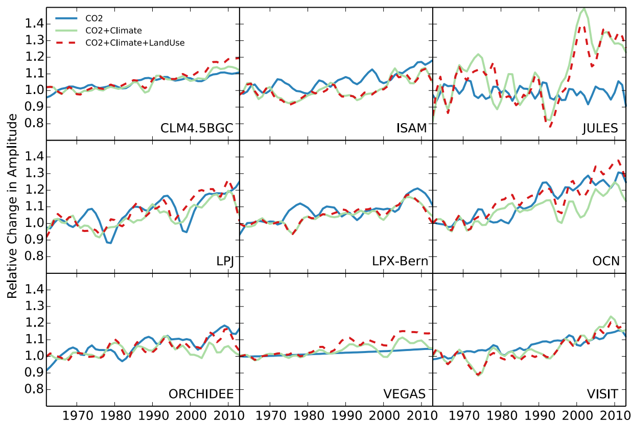
Figure 7. Trends for seasonal amplitude of global total net carbon fluxes from S1 (CO 2 ), S2 (CO 2 +Climate) and S3 (CO 2 +Climate+LandUse) for each individual TRENDY model. All amplitude time series are relative to their own 1961-1970 mean amplitude.
