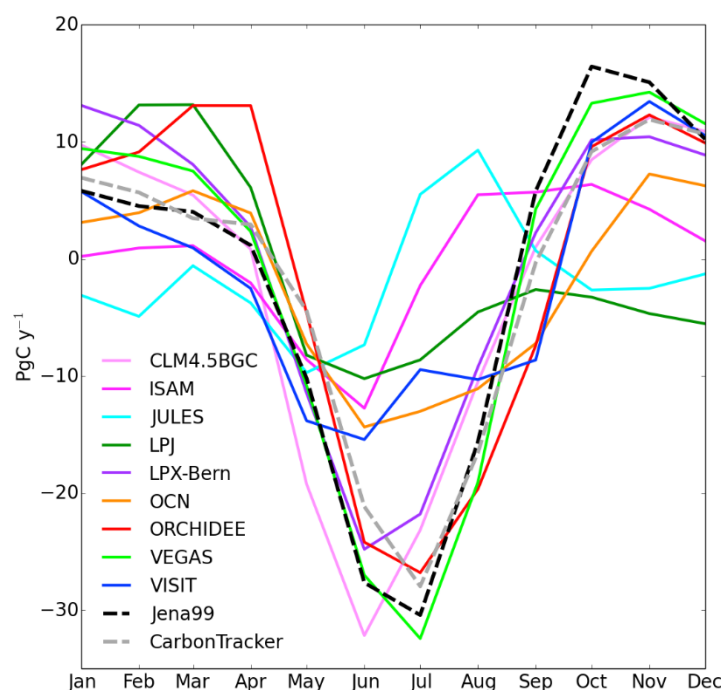
20 Figure 1. Mean seasonal cycle of global net carbon flux from nine TRENDY models (S3 experiment) and two inversions, Jena99 and CarbonTracker, averaged over 2001–2010.
