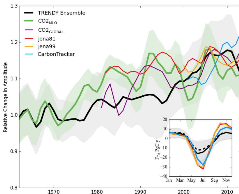
Figure 4. Trends for seasonal amplitude of TRENDY simulated multi-model ensemble mean land-atmosphere carbon flux F_{TA} (black), of MLO CO 2 mixing ratio (CO 2 MLO , green) and global CO 2 mixing ratio (CO 2 GLOBAL , purple), and of F_{TA} from atmospheric inversions of Jena81 (red), Jena99 (orange), and CarbonTracker (blue). The trends are relative to the 1961-70 mean for the TRENDY ensemble and Mauna Loa CO 2 , and the other time series are offset to have the same mean as the TRENDY ensemble for the last ten years (2003-2012). A 9-year Gaussian smoothing (Harris, 1978) removes inter-annual variability for all time series, and its 1- \sigma standard deviation is shown for CO 2 MLO (green shading). Note that the grey shading here instead indicates 1- \sigma models' spread, which is generally larger than the standard deviation of TRENDY ensemble's decadal variability. Inset: average seasonal cycles of models' ensemble mean F_{TA} (PgC y -1 ) for the two periods: 1961-1970 (dashed, lighter grey shade indicates 1- \sigma model spread) and 2001-2010 (solid, darker grey shade indicates 1- \sigma model spread), revealing enhanced CO 2 uptake during spring/summer growing season. Mean seasonal cycles global F_{TA} from the atmospheric inversions for 2001-2010 are also shown (same color as the main figure) for comparison.
