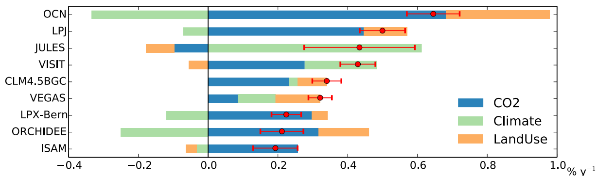
5 Figure 5. Attribution of the seasonal amplitude trend of global net land carbon flux for the period 1961-2012 to three key factors of CO 2 , climate and land use/cover. The red dots represent models' global amplitude increase of F_{TA} from the S3 experiment, and error bars indicate 1- \sigma standard deviation. The increasing seasonal amplitude of F_{TA} is decomposed into the influence of time varying atmospheric CO 2 (blue), climate (light green), and land use/cover change (gold).
