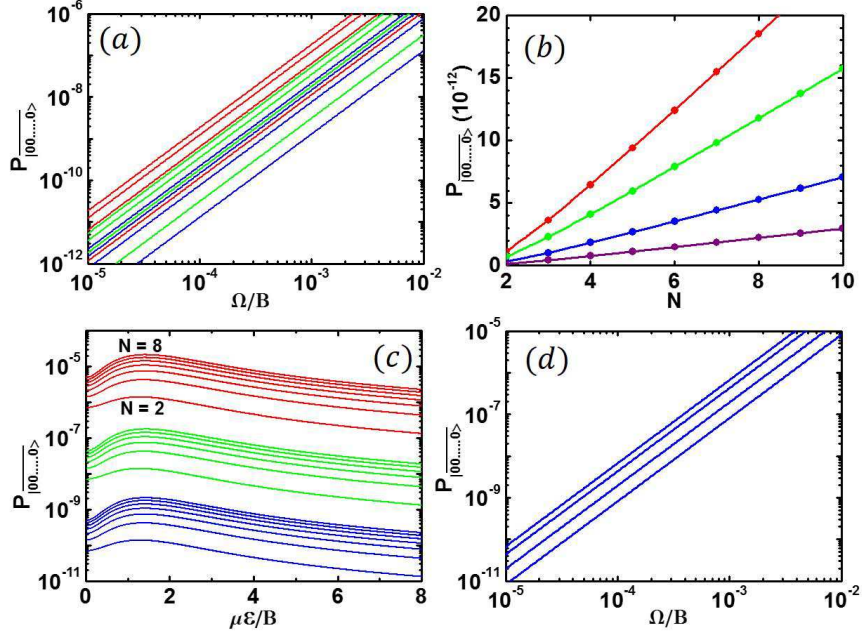
Figure 3: (a) P_{|00\dots 0\rangle} as a function of \Omega/B for different external electric fields: \mu\varepsilon/B = 2 (red), 3 (green) and 4.9 (blue). For each \mu\varepsilon/B , number of polar molecules are from bottom, N = 2, 4, 6, 8 , respectively. (b) P_{|00\dots 0\rangle} as a function of number of polar molecules in linear array when \Omega/B = 10^{-5} for different external electric fields: \mu\varepsilon/B = 2 (red), 3 (green), 4.9 (blue) and 8 (purple). (c) P_{|00\dots 0\rangle} as a function of external electric fields: \mu\varepsilon/B for different \Omega/B = 10^{-2} (red), 10^{-3} (green) and 10^{-4} (blue). For each \Omega/B , number of polar molecules are from bottom, N = 2, 3, 4, \dots, 8 , respectively. (d) P_{|00\dots 0\rangle} as a function of \Omega/B for 2-dimensional arrays in 3 \times 3 square lattice. External electric fields are from bottom, \mu\varepsilon/B = 2, 3, 4.9 and 8, respectively.
