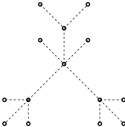
Figure 12. Example of a general tree level Feynman diagram (skeleton).
