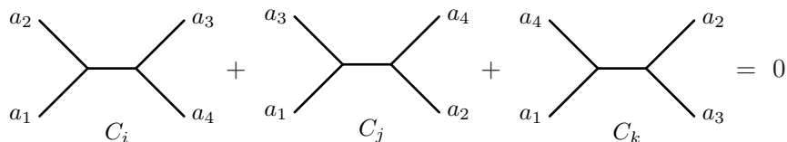
Figure 1. The Jacobi identity f^{a_1 a_2 b} f^{b a_3 a_4} + \text{cyc}(a_1, a_2, a_3) implies the vanishing of the color factors C_i, C_j and C_k associated to triplets of cubic graphs. In the above diagrams, the legs a_1, \dots, a_4 may represent arbitrary cubic tree-level subdiagrams. The duality between color and kinematics states that their corresponding kinematic numerators N_i built from polynomials of Mandelstam invariant for the cases of interest can be chosen such that N_i + N_j + N_k = 0 whenever C_i + C_j + C_k = 0 [5].
