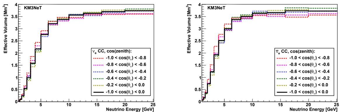
Figure 77: Effective volumes in \text{Mm}^3 ( 10^6 \text{ m}^3 ) as a function of neutrino energy for different true neutrino \cos(\text{zenith}) ranges, where \cos(\text{zenith})=-1 means vertical up-going and \cos(\text{zenith})=0 means horizontal. The solid black line corresponds to up-going neutrinos weighted according to the Bartol atmospheric neutrino flux model. Left: \nu_e CC. Right: \bar{\nu}_e CC.
