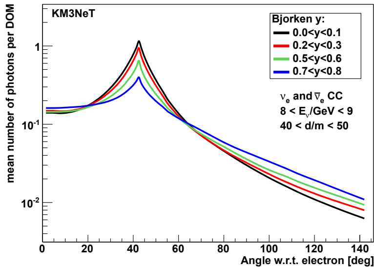
Figure 76: Number of expected photons \langle N_\gamma \rangle as a function of the angle \theta between the shower direction (which is the electron direction) and the vector from the vertex to the DOM for different inelasticity y intervals, and for shower energies of 8 \text{ GeV} < E < 9 \text{ GeV} and at distances of 40 \text{ m} < d < 50 \text{ m} .
