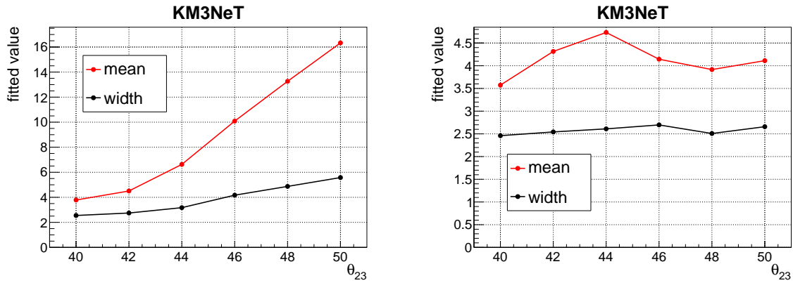
Figure 103: Mean and width of the LLR distributions for NH (left) and IH (right) pseudo-experiments as a function of \theta_{23} . These values were obtained from a Gaussian fit of the distributions.
