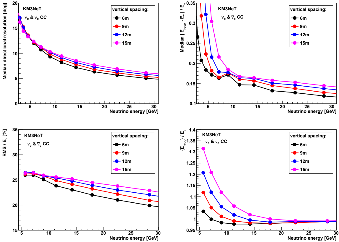
Figure 91: Resolution of the shower reconstruction for different vertical spacings for up-going \nu_e CC and \bar{\nu}_e CC events as a function of neutrino energy. Top left: median neutrino direction. Top right: median fractional energy resolution ( |E_{\text{reco}} - E_\nu|/E_\nu ). Bottom left: relative energy resolution \text{RMS}/E_\nu . Bottom right: mean relative offset in reconstructed energy \langle E_{\text{reco}} \rangle / E_\nu .
