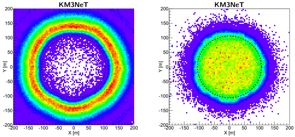
Figure 97: x-y distribution of the reconstructed track starting point for upward going reconstructed tracks: Left: atmospheric muons. Right: atmospheric neutrinos below 20 GeV. Up-going events with \Lambda > -6 are shown. The black lines represent the contour of the instrumented volume.
