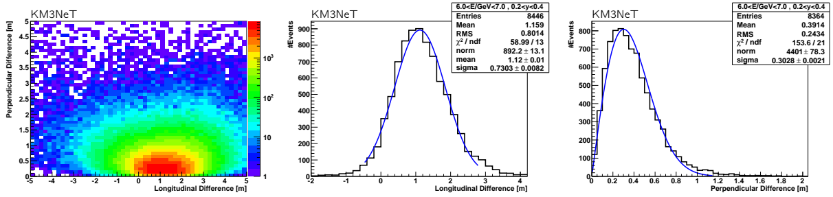
Figure 78: Longitudinal and perpendicular distance between the neutrino interaction position and the reconstructed vertex position for all selected events with E_\nu = 2 - 30 GeV (left). Longitudinal distance for 6 \text{ GeV} < E_\nu < 7 \text{ GeV} and 0.2 < y < 0.4 fitted with a Gaussian (middle). Perpendicular distance for the same E_\nu and y range fitted with 'distance \times a Gaussian' (right).
