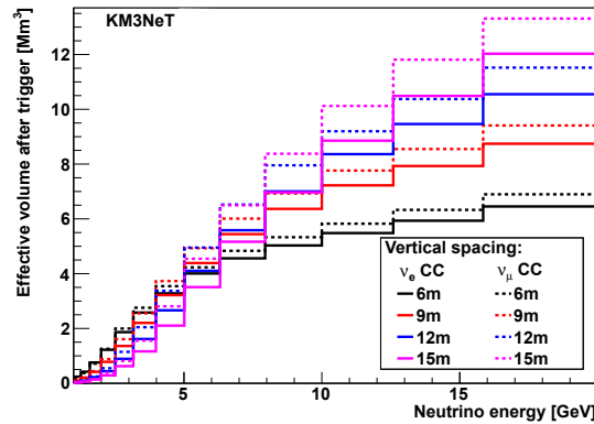
Figure 61: Effective volume at trigger level for different vertical spacings (6 m/9 m/12 m/15 m) as a function of neutrino energy for up-going \nu_e and \bar{\nu}_e CC (solid lines) and \nu_\mu and \bar{\nu}_\mu CC events (dashed lines).
