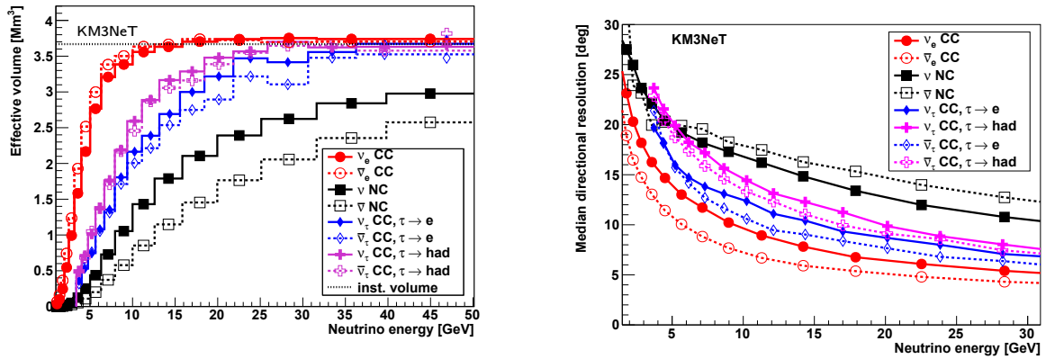
Figure 88: Effective volumes (left) and median neutrino direction resolution (right) as a function of neutrino energy for different up-going shower-like neutrino event types.
