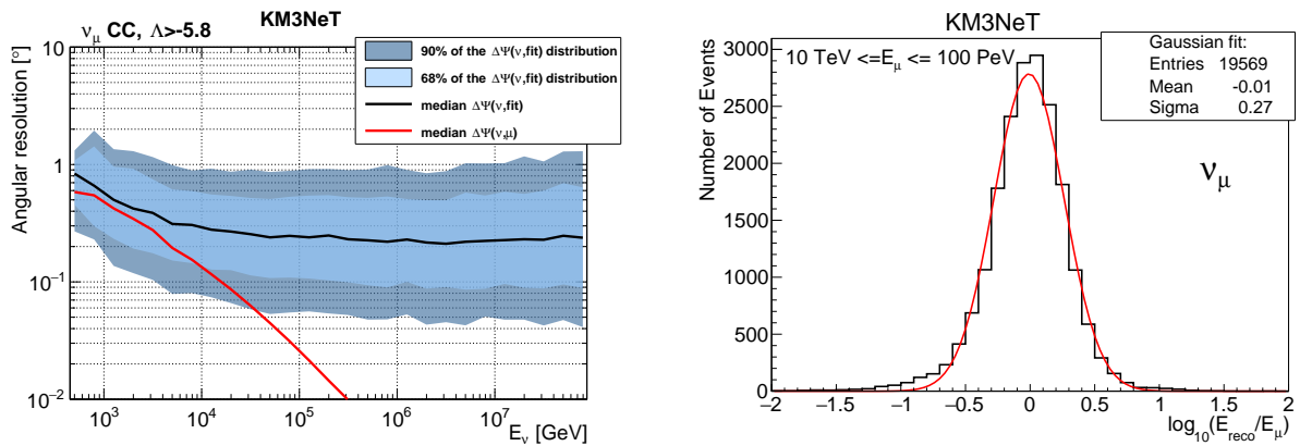
Figure 22: Left panel: median of the angle between the neutrino and the reconstructed muon direction (black line) and between the neutrino and the true muon direction (red line), for selected \nu_\mu CC events ( \Lambda > -5.8 , see below). The dark and light blue bands represent the 90% and 68% quantiles of the distributions. Right panel: distribution of \log_{10}(E_{\text{reco}}/E_\mu) , where E_{\text{reco}} is the reconstructed and E_\mu is the true muon energy for events with E_\mu \geq 10 TeV that satisfy a containment criterion. The red line represents the Gaussian fit.
