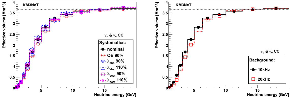
Figure 94: Effective volumes for different water properties, quantum efficiencies (QE) and optical background noise rates for up-going \nu_e CC and \bar{\nu}_e CC events. Different absorption \lambda_{\text{abs}} and scattering length \lambda_{\text{scat}} , and quantum efficiencies (left) and 10 kHz and 20 kHz single optical noise rates (right).
