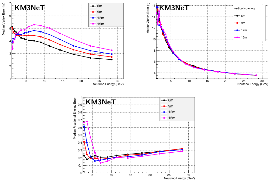
Figure 68: Median resolution as a function of the true neutrino energy, for various vertical spacings, of: the distance between the true interaction vertex and reconstructed one (top left), the absolute value of the difference between the reconstructed zenith angle and the true neutrino zenith (top right), and the fractional energy error (bottom). For muon neutrino and antineutrino events weighted according to the atmospheric spectrum, reconstructed as up-going, with vertex reconstructed within the instrumented volume and \Lambda > -5.0 .
