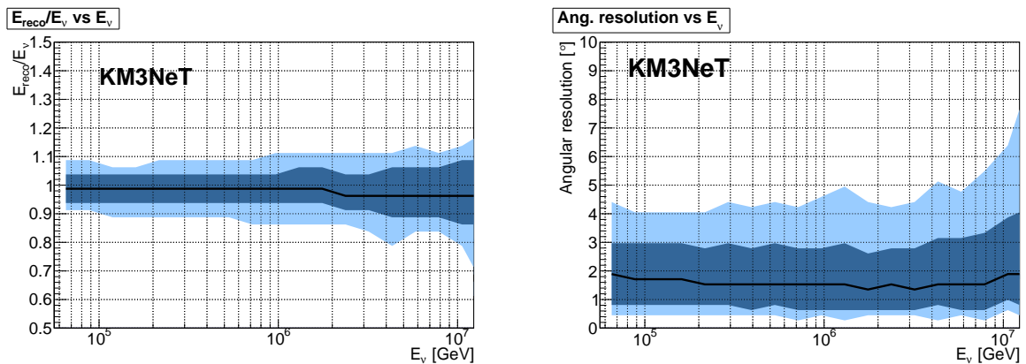
Figure 24: ARCA resolutions for contained \nu_e CC events using Algorithm 1, after the event selection of Sec. 2.3.1. Left: energy resolution, right: directional resolution. For both plots, the black line shows the median value; dark blue shaded regions give the 68% range, while light blue shaded regions give the 90% range.
