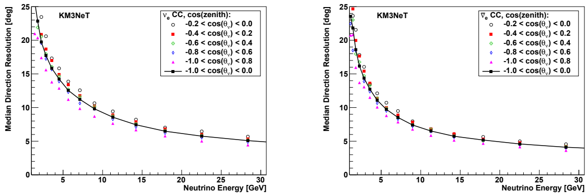
Figure 80: Median neutrino direction resolution (angle between reconstructed direction and neutrino direction) as a function of neutrino energy for different true neutrino \cos(\text{zenith}) ranges, where \cos(\text{zenith})=-1 means vertical up-going and \cos(\text{zenith})=0 means horizontal. The black line corresponds to up-going neutrinos weighted according to the Bartol flux model. \nu_e CC (left) and \bar{\nu}_e CC (right).
