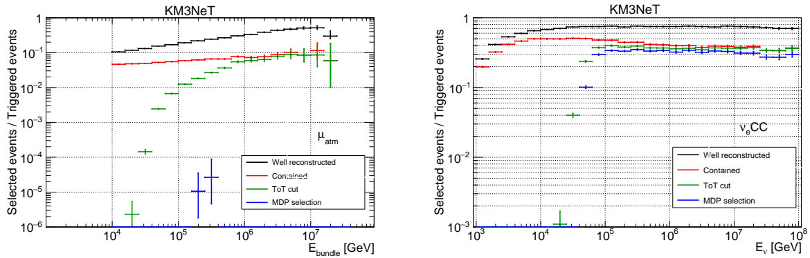
Figure 30: Ratio of the numbers of selected events and triggered events at each step of the cascade analysis (see text) for atmospheric muons (left) and \nu_e CC neutrino reactions (right) as a function of the primary energy.
