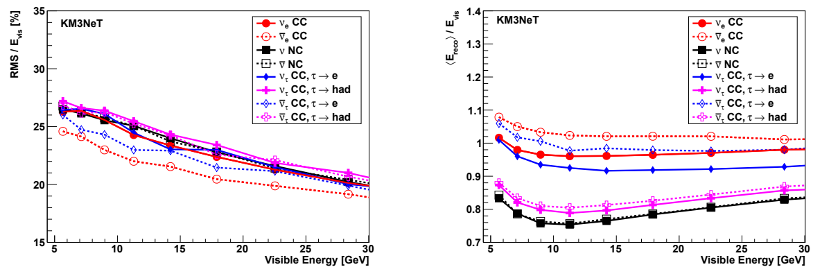
Figure 87: Relative energy resolution \text{RMS}/E_{\text{vis}} as a function of the visible energy E_{\text{vis}} for shower-like neutrino interaction channels (left) and mean relative offset in reconstructed energy – given as \langle E_{\text{reco}} \rangle / E_{\text{vis}} – as a function of E_{\text{vis}} (right).
