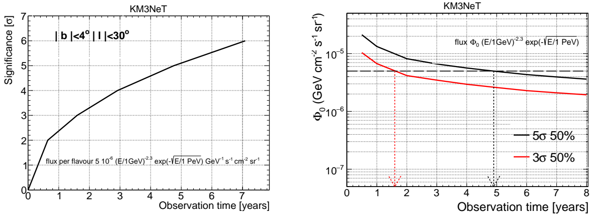
Figure 36: Significance (left) and 5\sigma and 3\sigma discovery fluxes (right) for KM3NeT/ARCA (2 building blocks) as a function of the observation time for the detection in the track channel of a diffuse flux of neutrinos from a selected region of the GP near the Galactic Center (see text).
