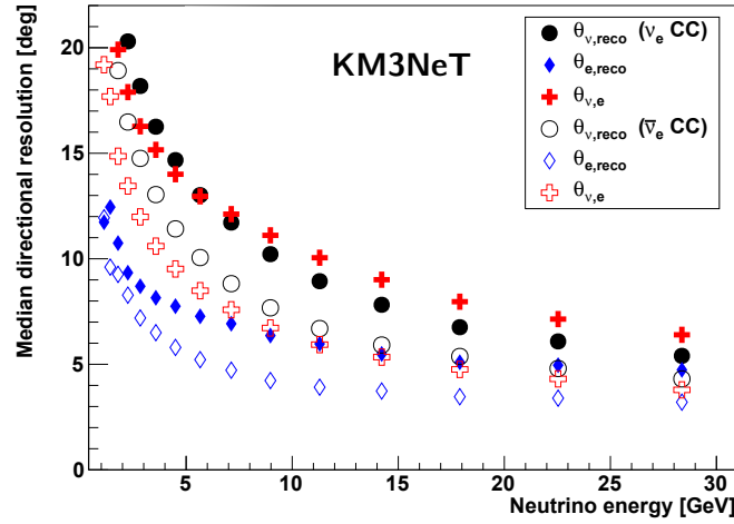
Figure 81: Median intrinsic scattering angle (red crosses), median electron direction resolution (blue diamonds) and the median neutrino direction resolution (black filled circles) as a function of neutrino energy for up-going \nu_e CC (solid marker) and \bar{\nu}_e CC (hollow marker) events weighted according to the Bartol flux model.
