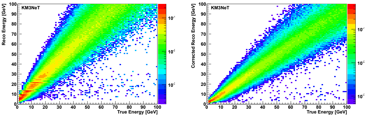
Figure 84: Reconstructed energy as a function of true neutrino energy for \nu_e CC and \bar{\nu}_e CC events weighted according to the Bartol flux model (left). Corrected reconstructed energy as a function of true neutrino energy for the same events (right).
