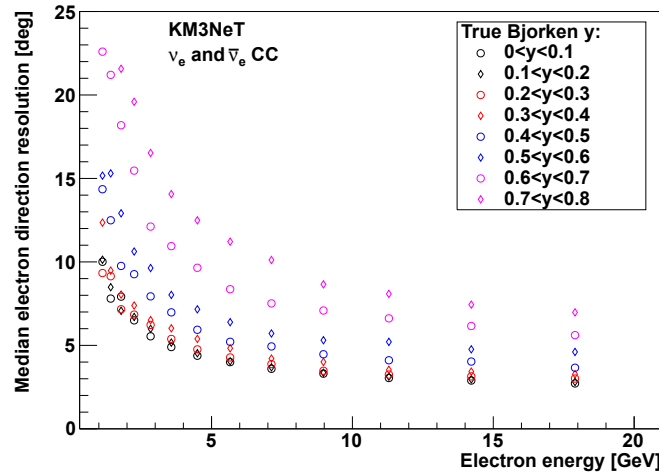
Figure 82: Median electron direction resolution (angle between reconstructed direction and electron direction) as a function of electron energy for up-going \nu_e and \bar{\nu}_e CC events weighted according to the Bartol flux model. Different marker colours and styles represent different true inelasticity y ranges.
