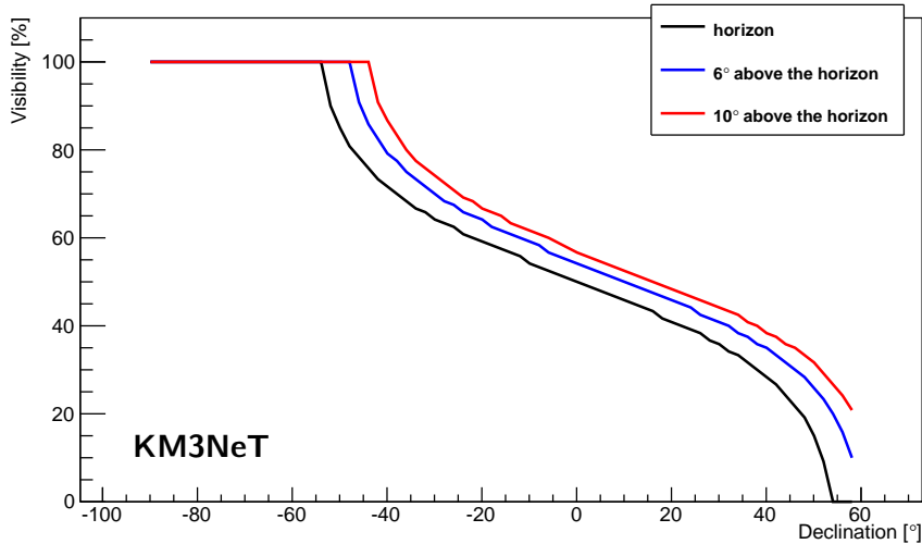
Figure 37: KM3NeT/ARCA visibility as a function of source declination for the muon-track analysis, for 2\pi downward coverage, i.e. tracks below the horizon (black line); tracks up to 6^\circ above the horizon (blue line); and tracks up to 10^\circ above the horizon (red line).
