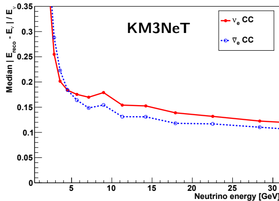
Figure 86: Median fractional energy resolution ( |E_{\text{reco}} - E_{\nu}|/E_{\nu} ) as a function of neutrino energy for \nu_e CC (red) and \bar{\nu}_e CC (blue) events weighted according to the Bartol flux model.
