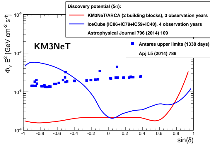
Figure 43: KM3NeT/ARCA (2 building blocks) 5\sigma discovery potential as a function of the source declination (red line) for one neutrino flavour, for point-like sources with a spectrum \propto E^{-2} and 3 years of data-taking. For comparison, the corresponding discovery potential for the IceCube detector [70] (blue line), and upper limits on particular sources for the ANTARES detector [71] (blue squares) are also shown.
