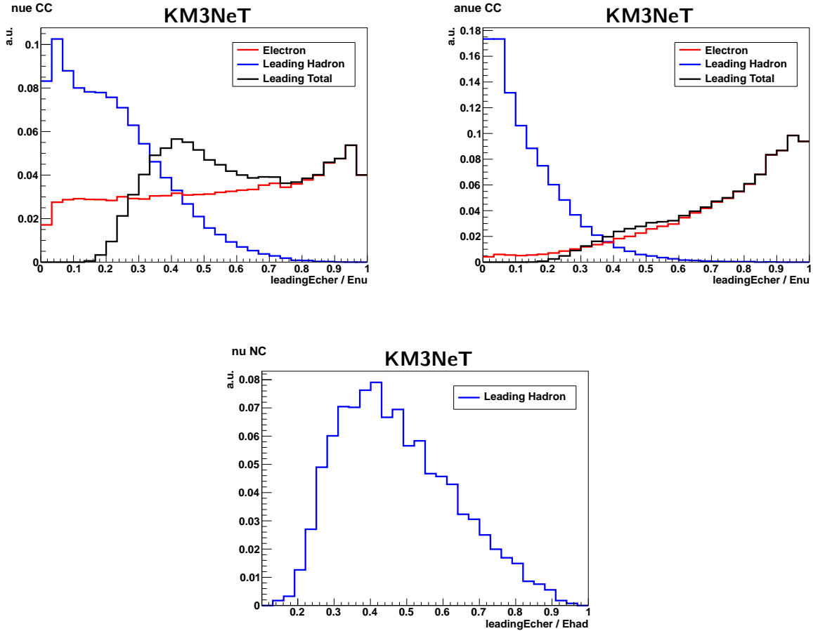
Figure 73: Distribution of E_e/E_\nu (red), the leading E_{\text{had}}^{\text{cher}}/E_\nu in the hadronic shower (blue) and the leading E_{\text{tot}}^{\text{cher}}/E_\nu of the total event (back). Top left: \nu_e CC events with 9 \text{ GeV} < E_\nu < 11 \text{ GeV} . Top right: \bar{\nu}_e CC events with 9 \text{ GeV} < E_\nu < 11 \text{ GeV} . Bottom: \nu_e and \bar{\nu}_e NC events with 9 \text{ GeV} < E_{\text{had}} < 11 \text{ GeV} .
