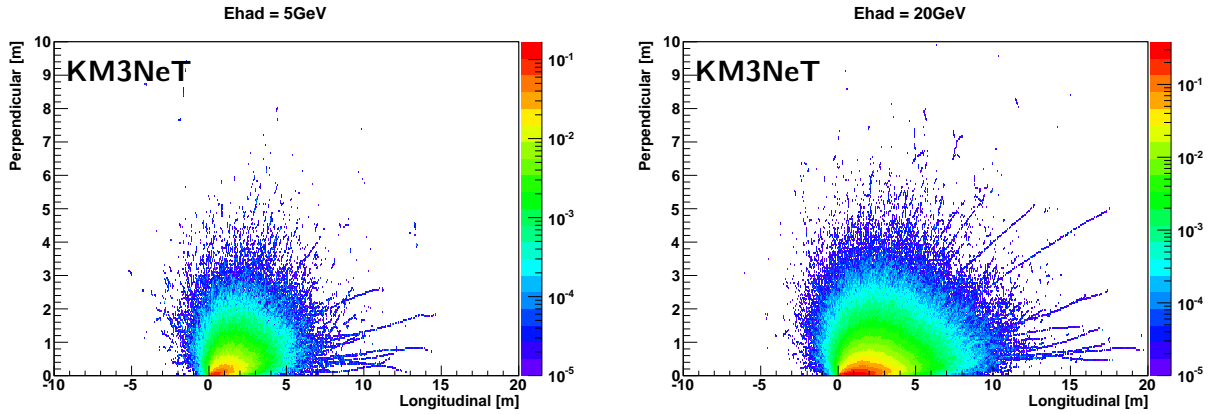
Figure 58: Simulated Cherenkov photon emission positions along and perpendicular to the direction of hadronic showers from \nu_e CC events. 3400 superimposed hadronic showers with E_{\text{had}} \approx 5 GeV (left). 4000 superimposed hadronic showers with E_{\text{had}} \approx 20 GeV (right).
