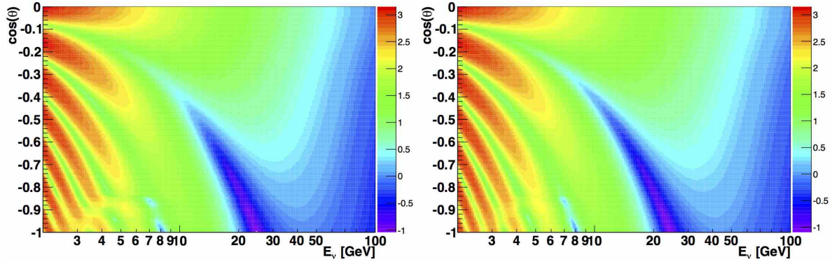
Figure 50: Neutrino “oscillograms”: \nu_\mu + \bar{\nu}_\mu event rate (in units of \text{GeV}^{-1} \cdot \text{y}^{-1} \cdot \text{sr}^{-1} in log scale) as a function of the neutrino energy and cosine of the zenith angle, for a 1 Mton target volume. The left (right) plot shows the distribution for the normal (inverted) mass hierarchy.
