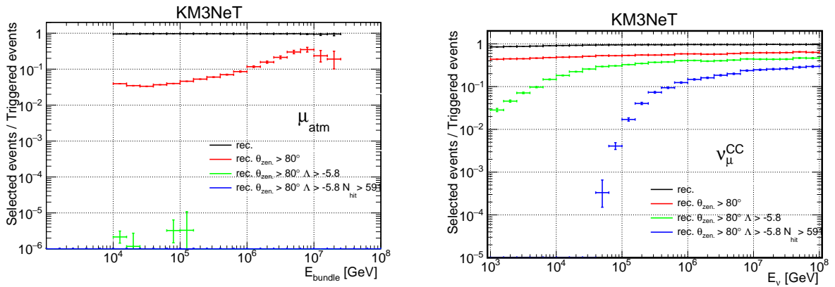
Figure 32: Ratio of the numbers of selected events and triggered events at each step of the track analysis (see text) for atmospheric muons (left) and \nu_{\mu} CC neutrino reactions (right) as a function of the primary energy.
