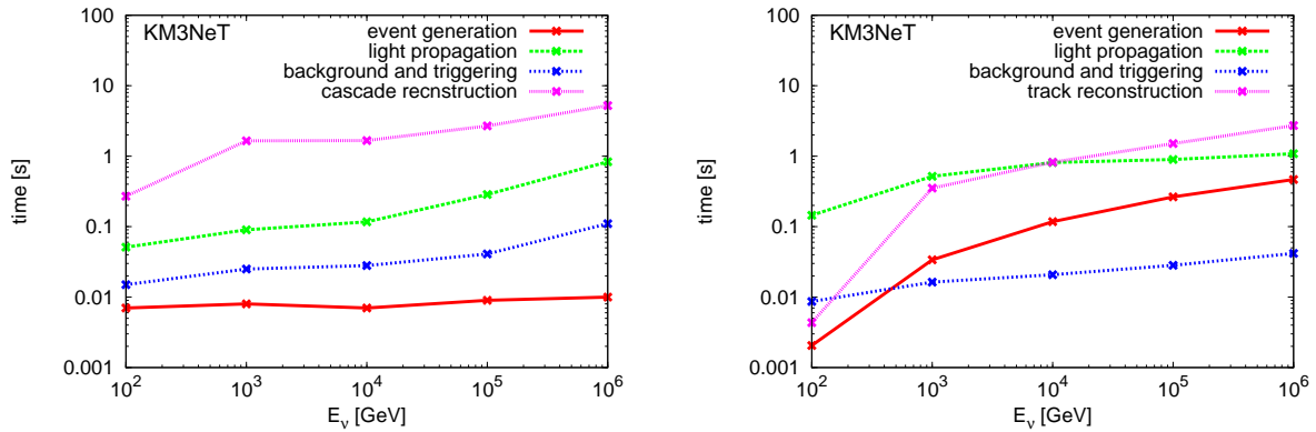
Figure 20: Simulation times per triggered event for different simulation stages, for \nu_e CC (cascade) events (left), and \nu_\mu CC (track) events (right). The times are calculated for simulations run on a single dedicated CPU at the Centre de Calcul de l'IN2P3/CNRS.
