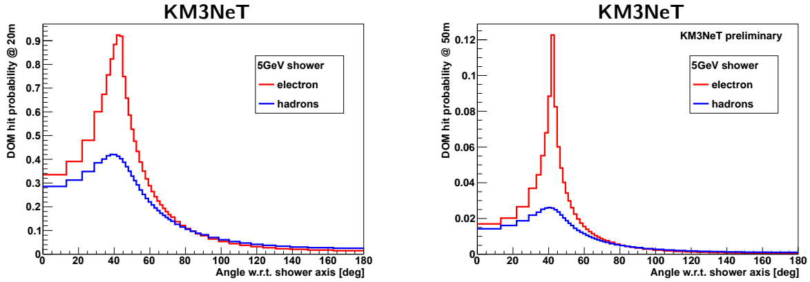
Figure 72: DOM-hit probability (probability to detect at least one photon in an entire multi-PMT optical module) at a distance of 20 m (left) and 50 m (right) away from the brightest point for showers with E_e = E_{\text{had}} = 5 GeV as a function of the angle \theta between shower direction and the vector from the brightest point to the DOM centre.
