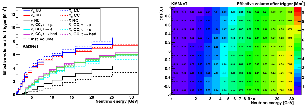
Figure 60: Effective volume at trigger level (left) for 6 m vertical spacing as a function of neutrino energy for different neutrino flavours (up-going events only) and effective volume at trigger level for \nu_e CC events as a function of neutrino energy and cosine of the neutrino zenith angle \theta_\nu (right).
