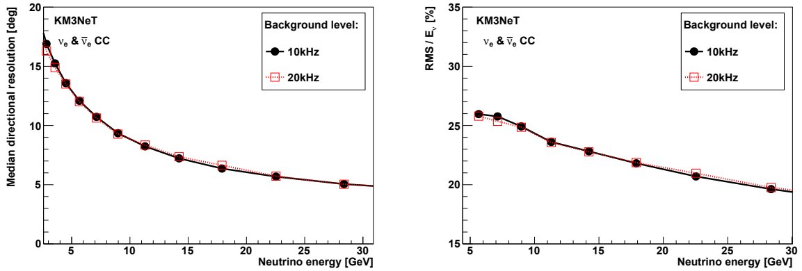
Figure 93: Resolution of the shower reconstruction for 10 kHz and 20 kHz single optical noise rates for up-going \nu_e CC and \bar{\nu}_e CC events. Median neutrino direction (left) and relative energy resolution \text{RMS}/E_\nu (right).
