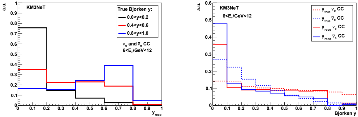
Figure 83: Distribution of reconstructed inelasticity y_{\text{reco}} for three different true y ranges ( 0 < y < 0.2 , 0.4 < y < 0.6 and 0.8 < y < 1 ) for \nu_e CC and \bar{\nu}_e CC events with 6 \text{ GeV} < E_\nu < 12 \text{ GeV} weighted according to the Bartol flux model (left). Distributions of the reconstructed inelasticity y_{\text{reco}} (solid lines) and true inelasticity y_{\text{true}} (dashed lines) for \nu_e CC and \bar{\nu}_e CC events (right).
