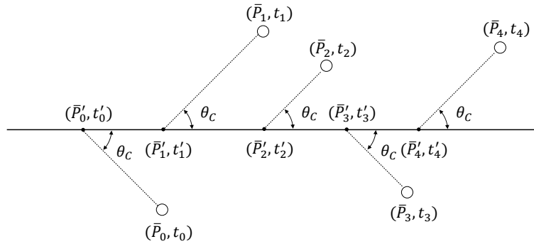
Figure 64: Schematic of the track length estimation procedure. The horizontal arrow indicate the reconstructed muon trajectory, the open circles the PMTs which recorded a hit and the solid dots their projections on the muon trajectory according the Cherenkov hypothesis.
