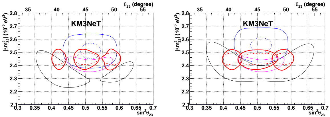
Figure 108: Measurement precision in \Delta M^2 and \sin^2 \theta_{23} after three years of data taking with ORCA with (solid red) and without (dashed red) energy scale uncertainty for three test points compared to present results from MINOS (black) [179] and T2K (blue) [105] and predicted performance of NOvA (magenta) [180] and T2K (blue, dashed) [105] in 2020. All contours are at 1\sigma , left for NH, right IH.
