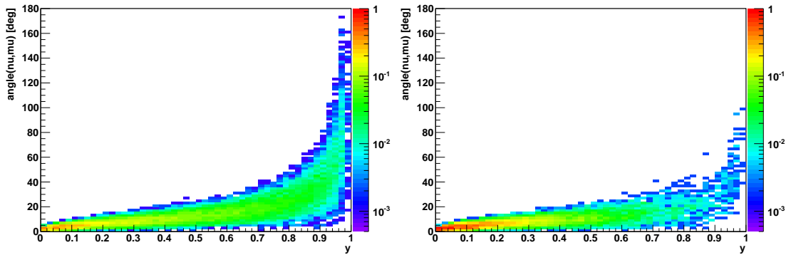
Figure 52: Scattering angle \phi_{\nu,\mu} as a function of Bjorken y for neutrinos (left) and antineutrinos (right) for (anti)neutrino energies of 10 GeV. The distributions are normalised to 1. [plot obtained with ORCA tools based on GENIE]
