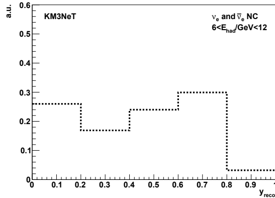
Figure 89: Distribution of reconstructed inelasticity y_{\text{reco}} for NC events with hadronic shower energies of 6 \text{ GeV} < E_{\text{had}} < 12 \text{ GeV} and an arbitrary true inelasticity.
