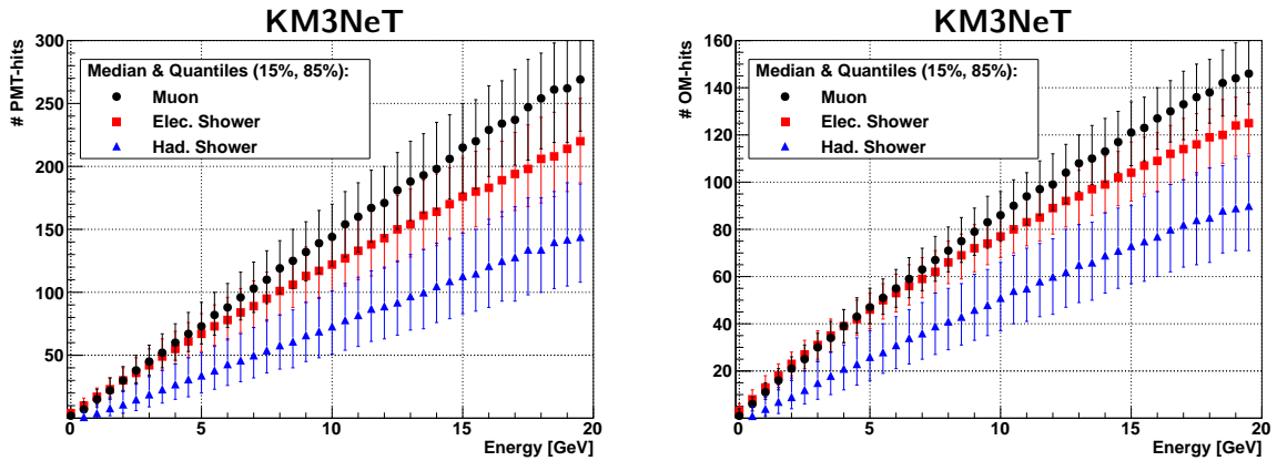
Figure 56: Median and 15 % / 85 % quantiles (vertical bars) for the distribution of the number of PMT (left) and DOM (right) hits generated by a muon, an electromagnetic and a hadronic shower as a function of their respective energy. The KM3SIM package has been used.
