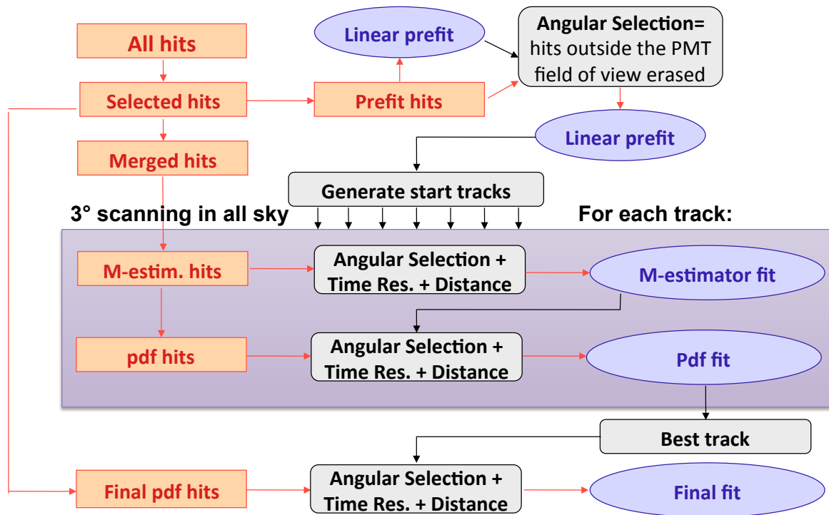
Figure 62: Schematic depiction of the reconstruction algorithm.
