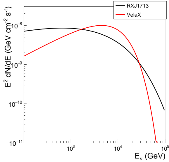
Figure 38: \nu_\mu + \bar{\nu}_\mu energy spectra for RX J1713 (Eq. 6, black line) and Vela-X (Eq. 7, red line).
