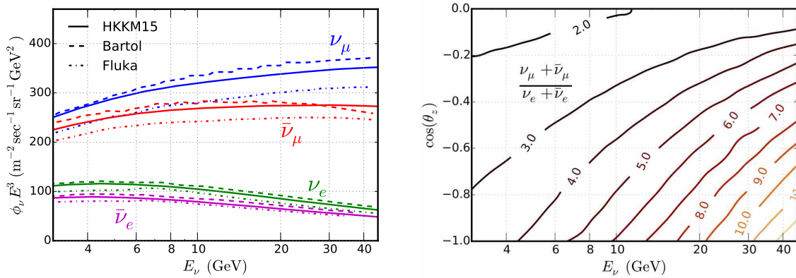
Figure 49: Atmospheric neutrino flux in its different flavour components: absolute values (left) and ratios (right). Taken from [144].
