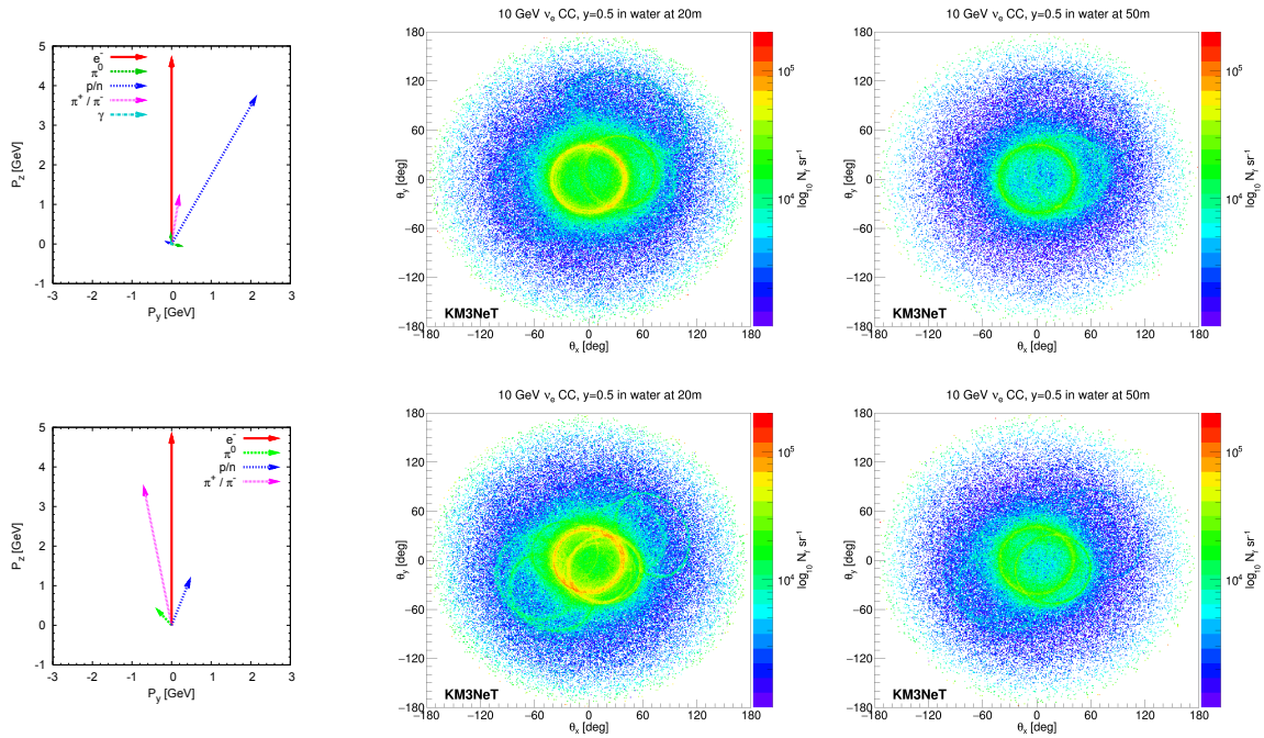
Figure 71: Two different simulated \nu_e CC events with E_\nu \approx 10 GeV and y \approx 0.5 in the upper and lower row. Each event is rotated in such a way that the electron is in the z -direction. Left: Illustration of the particles produced in the two events. Each arrow represents one particle. The arrow direction and length correspond to the particle momentum in the p_y - p_z -plane, and the arrow colour indicates the particle type. Middle and right: Photon distributions in sea water recorded on shells at 20 m and 50 m around the neutrino interaction vertex. Each photon is weighted with the solid angle averaged effective area of a PMT for the photon wavelength. The Cherenkov ring from the electron is centred around (0,0) with an opening angle of 42^\circ , as the electron moves in the z -direction.
