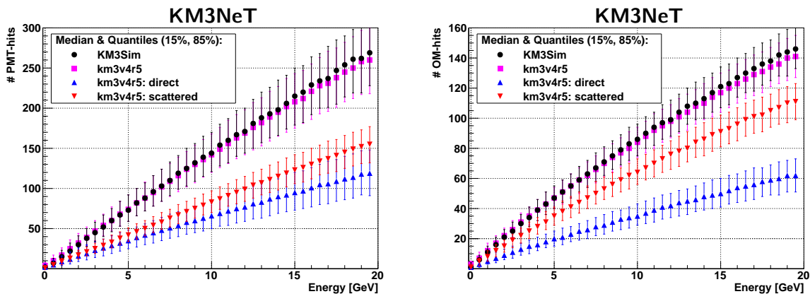
Figure 55: Median and 15% / 85% quantiles (vertical bars) for the distribution of the number of PMTs with hits (left) and DOMs with at least one hit (right) generated by a muon as a function of its energy. Shown are results for two different simulation packages (KM3 (v4r5) and KM3SIM); for the simulation with KM3 the light yield is differentiated into 'direct', 'scattered' and 'all' light.
