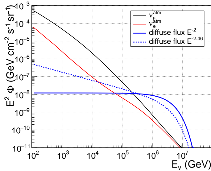
Figure 28: Diffuse signal fluxes according to Eq. 3 (full blue line) and Eq. 4 (dashed blue line) as a function of the neutrino energy. For comparison the atmospheric neutrino fluxes are also reported (Honda flux [18] for the conventional component and the Enberg flux [19] for the prompt component, see Sec. 2.1.2).
