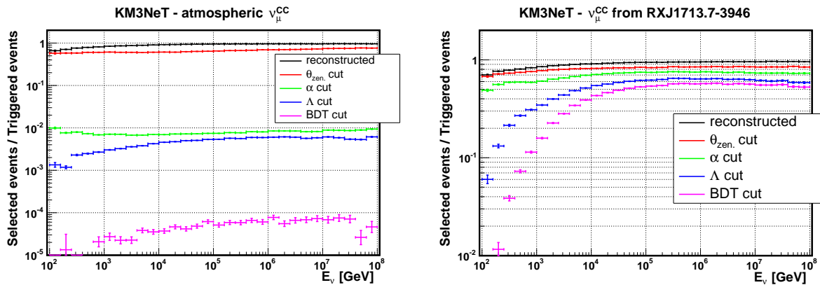
Figure 40: Ratios between the numbers of selected events and triggered events at each step of the analysis for atmospheric \nu_\mu CC neutrinos (left panel) and \nu_\mu CC neutrinos from the source (right panel) as a function of the neutrino energy.
