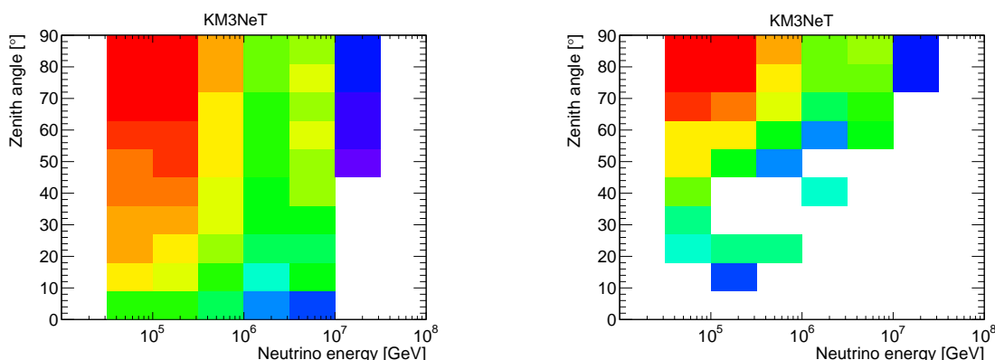
Figure 27: Effect of the self-veto on down-going \bar{\nu}_e events as a function of energy and zenith angle, showing the yearly rate both before (left) and after (right) the self-veto effect is taken into account. Figure taken from [35] (Fig. 4).
