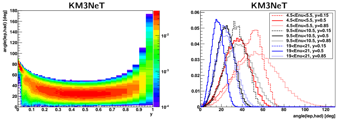
Figure 66: Angle between the outgoing muon and the outgoing hadronic shower \phi_{\mu,lep} from \nu_{\mu}CC interactions with 9.5 < E_{\nu}/GeV < 10.5 as a function of inelasticity y . The kinematics looks very similar for \nu_eCC interactions. The features at 0 < y < 0.2 are due to the different neutrino interaction channels (cf. Fig. 57). Each column of bins in y is normalised to 1 (left). Distribution of the opening angle \phi_{\mu,lep} in \nu_{\mu}CC interactions for three different inelasticities y and neutrino energies (right).
