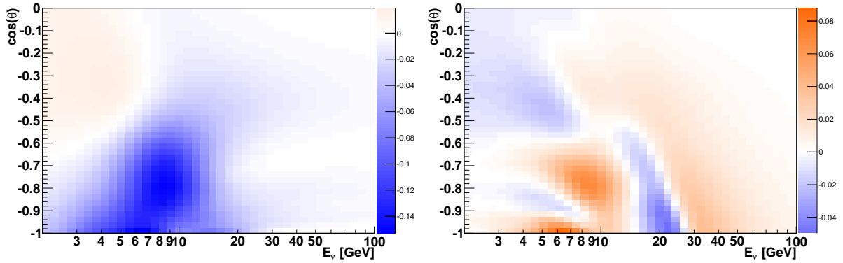
Figure 53: Asymmetry (as defined by Eq. 19) between the number of \nu + \bar{\nu} CC interactions expected in case of NH and IH, expressed as a function of the energy and the cosine of the zenith angle. The right (left) plot applies to muon (electron) neutrinos. A smearing of 25% is applied on the energy. On the angle, a smearing \sigma_\theta = \sqrt{\frac{m_p}{E_\nu}} is applied, where m_p denotes the nucleon mass and E_{nu} the neutrino energy in GeV.
