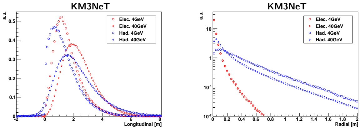
Figure 70: Light emission profiles of electromagnetic (red) and hadronic showers (blue) with 4 GeV and 40 GeV energy, depicted in shower direction (left, longitudinal) and perpendicular to the shower direction (right, transverse).
