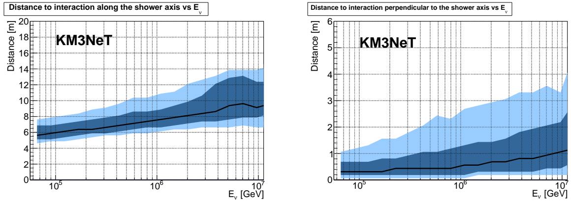
Figure 23: ARCA vertex resolutions for contained \nu_e CC events using Algorithm 1, after the event selection of Sec. 2.3.1. Left: resolution in the longitudinal direction, showing the offset from the MC vertex to the shower maximum. Right: directional resolution in the lateral direction, which gives the characteristic accuracy of \sim 0.5 m. For both plots, the black line shows the median value; dark blue shaded regions give the 68% range, while light blue shaded regions give the 90% range.
