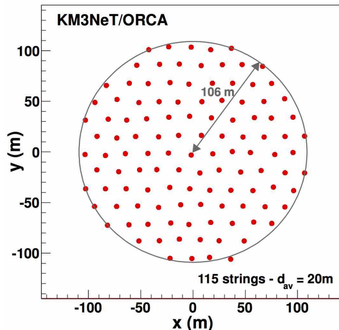
Figure 54: Footprint of the ORCA benchmark detector (top view), with 115 strings (20 m spacing) with 18 OMs each (6 m spacing). The instrumented volume is 3.6 \times 10^6 \text{ m}^3 (cylinder: R=106 \text{ m} , z=102 \text{ m} )
