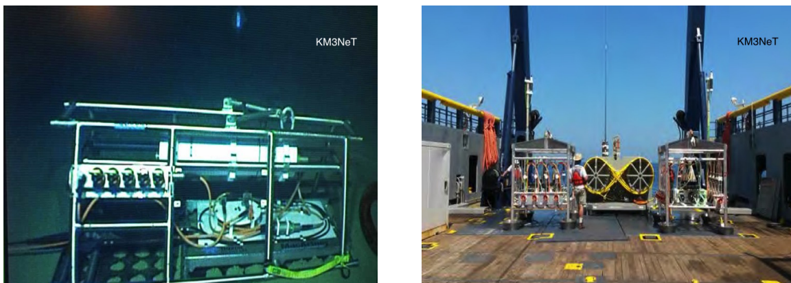
Figure 5: Photograph of the CTF after deployment on the seabed (left). Photograph of two secondary junction boxes on the boat prior to deployment (right).
