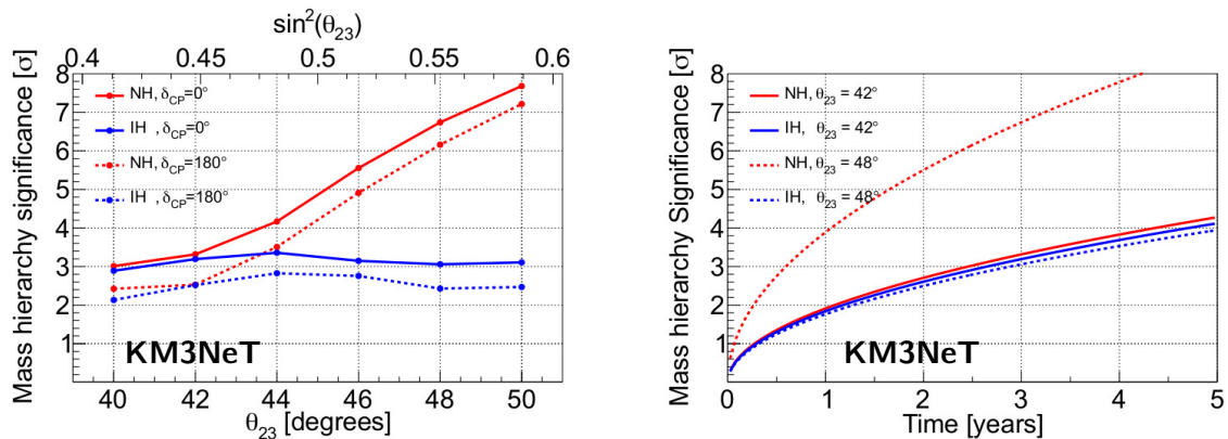
Figure 106: The mass hierarchy sensitivity for 9 m spacing, using the default settings. This includes a fit of \theta_{23} , \Delta M^2 , \delta_{CP} and the five systematics. The left plot shows its dependency on \theta_{23} for two values \delta_{CP} for three years of operation time whereas the right plot illustrates its improvement over time for two selected values of \theta_{23} and \delta_{CP} = 0^\circ .
