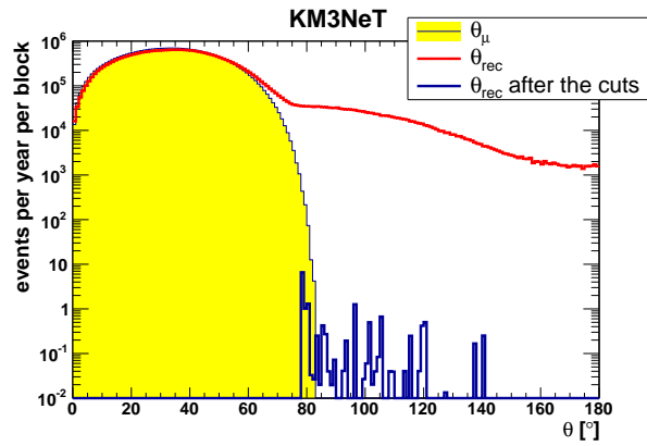
Figure 39: Distributions of the zenith angle \theta_{\text{rec}} of atmospheric muons for one KM3NeT/ARCA building block at generation level (yellow area), reconstruction level (red line), and after the preselection cut and the cut on \Lambda (blue histogram).
