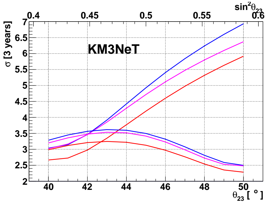
Figure 107: NMH Sensitivity for 3 years of data taking as function of the true mixing angle \theta_{23} for both hierarchy hypotheses. Different vertical distances between adjacent DOMs are simulated: red 6 m, blue 9 m, magenta 12 m.
