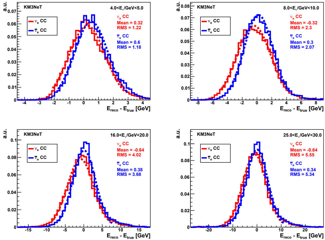
Figure 85: Difference between corrected reconstructed energy and neutrino energy in different neutrino energy bins for \nu_e CC (red) and \bar{\nu}_e CC (blue) events weighted according to the Bartol flux model. Dashed lines show Gaussian fits.
