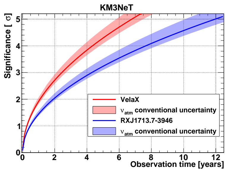
Figure 42: Significance as a function of KM3NeT/ARCA (2 building blocks) observation time for the detection of the Galactic sources RX J1713 and Vela-X. The bands represent the effect of the uncertainties on the conventional component of the atmospheric neutrino flux.
