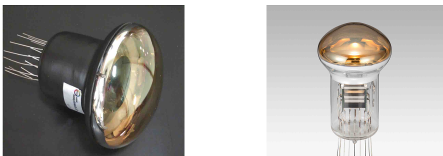
Figure 13: Photographs of the PMTs. ETEL D792KFL (left) and Hamamatsu R12199-02 (right).
