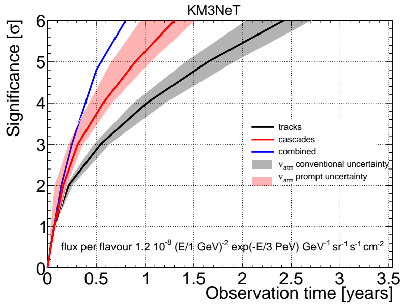
Figure 35: Significance as a function of KM3NeT/ARCA (2 building blocks) observation time for the detection of a diffuse flux of neutrinos corresponding to the signal reported by IceCube (Eq. 3) for the cascade channel (red line) and muon channel (black line). The black and red bands represent the uncertainties due to the conventional and prompt component of the neutrino atmospheric flux. The blue line represents the results of the combined analysis (see text).
