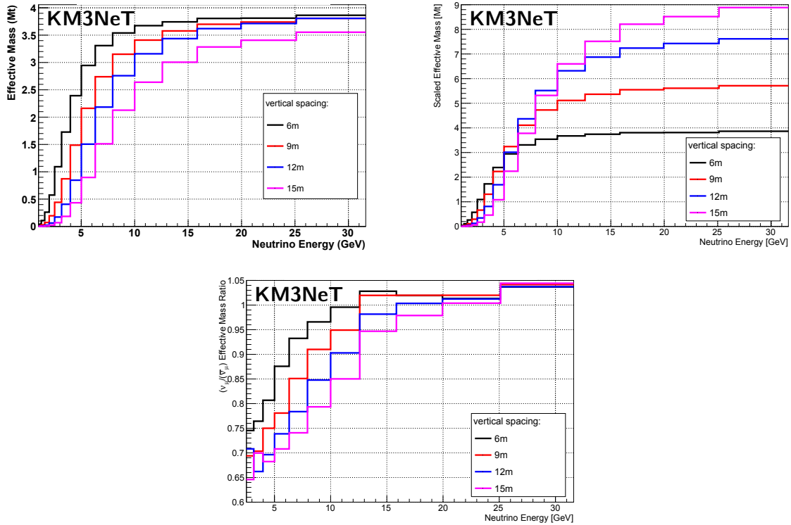
Figure 69: Top left: effective mass for \nu_\mu and \bar{\nu}_\mu as a function of the neutrino energy for events reconstructed as up-going and whose vertex is reconstructed inside the instrumented volume with a reconstruction quality \Lambda > -5.0 , for 4 different vertical spacings. Top right: effective masses for 6 m/9 m/12 m/15 m scaled by a factor 1/1.5/2/2.5. Lower plot: ratio between neutrino and antineutrino effective masses as a function of the neutrino energy.
