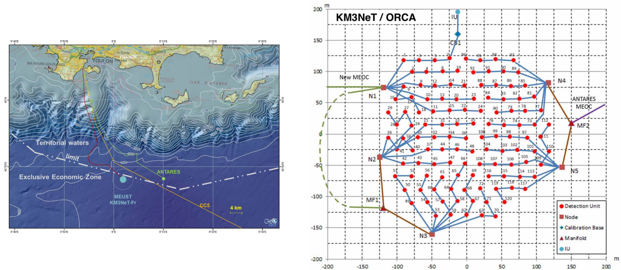
Figure 6: Map of the Mediterranean Sea south of Toulon, France. The location of the KM3NeT-France and ANTARES installations are indicated (left). Layout of the ORCA array (right), depicting the 115 (+5 contingency) Detection Units, cables and connection devices of the full array.
