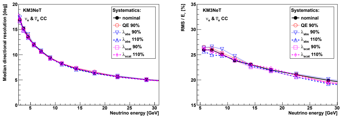
Figure 92: Resolution of the shower reconstruction for different water properties ( \lambda_{\text{abs}} and \lambda_{\text{scat}} ) and quantum efficiencies (QE) for up-going \nu_e CC and \bar{\nu}_e CC events. Median neutrino direction (left) and relative energy resolution \text{RMS}/E_\nu (right).
