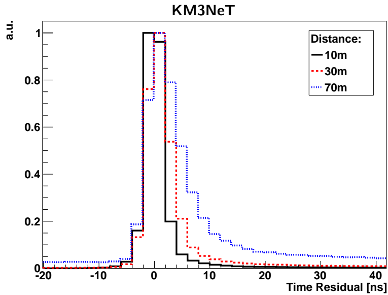
Figure 74: Time residual distribution for three different distances d between the vertex and the PMT, obtained from simulations of fully contained \nu_e CC and \bar{\nu}_e CC events with 5 kHz noise rate. The time residual is defined with respect to the brightest point of the shower. The distributions are normalised so that the maximum is 1.
