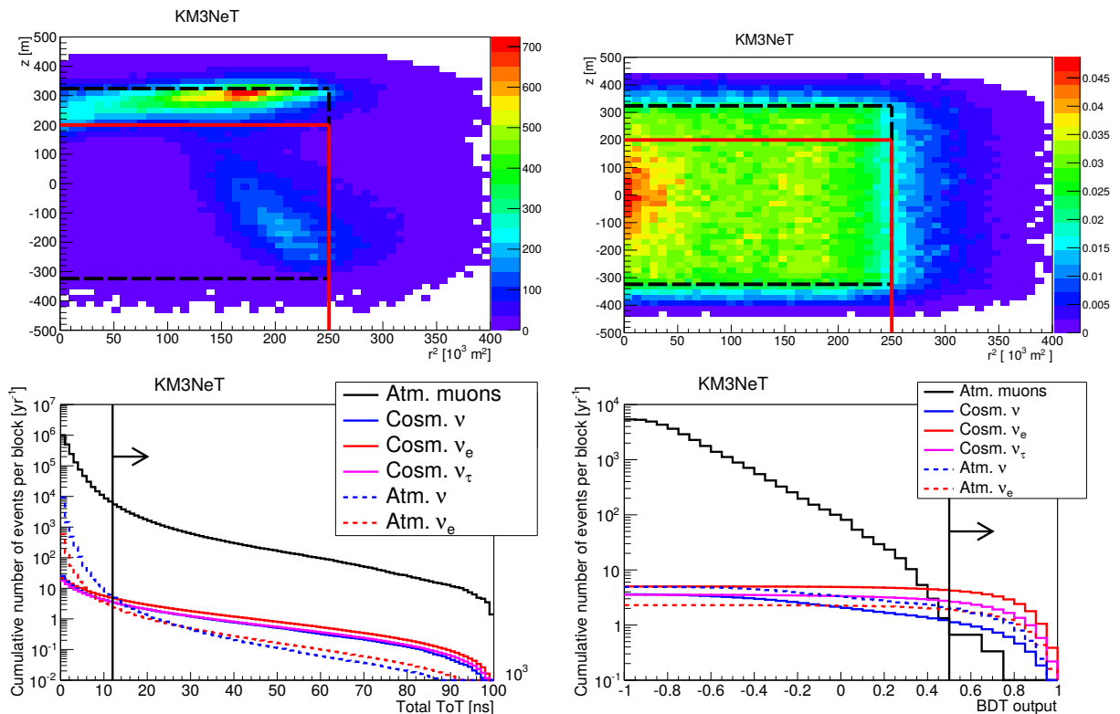
Figure 29: Reconstructed vertex positions ( r and z are the radial and vertical distances from the detector centre) for atmospheric muon events (left top) and \nu_e CC events (right top), for one KM3NeT/ARCA building block in one year of operation (events \text{yr}^{-1} \text{bin}^{-1} ). The black dashed lines show the instrumented volume of one building block. The red line shows the selected fiducial volume defined by r < 500 m and z < 200 m. Left bottom: cumulative distribution of \text{ToT}_{\text{evt}} (see text) for events contained in the fiducial volume, for the different event classes. Right bottom: cumulative distribution of the BDT output \rho for the preselected events (see text) for the different event classes. Vertical lines represent the selection cuts applied.
