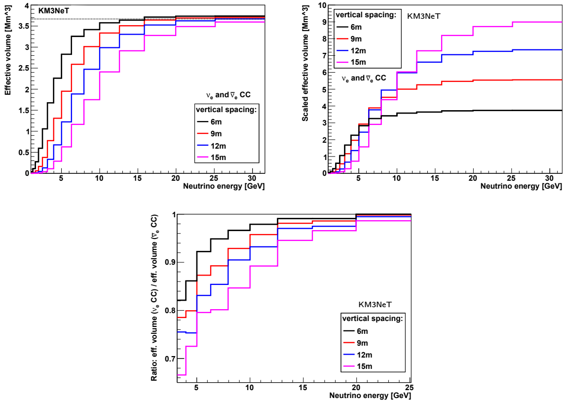
Figure 90: Effective volumes for the different vertical spacings (top left). Effective volumes for 6m/9m/12m/15m scaled by a factor 1/1.5/2/2.5 (top right). Ratio of neutrino and antineutrino effective volumes for charged-current electron neutrino events for the different vertical spacings (bottom).
