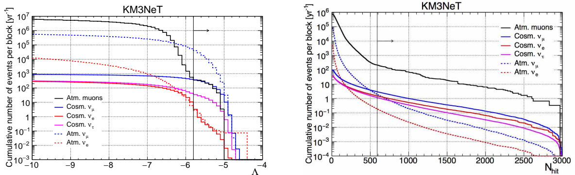
Figure 33: Cumulative distribution of the \Lambda parameter (left) and of the number of hits, N_{\text{hit}} , (right) for events per KM3NeT/ARCA building block with \theta_{\text{rec}} > 80^\circ . The cosmic neutrino signal corresponds to the flux given in Eq. 3. The vertical lines indicate the final cut values applied in the analysis (see text).
