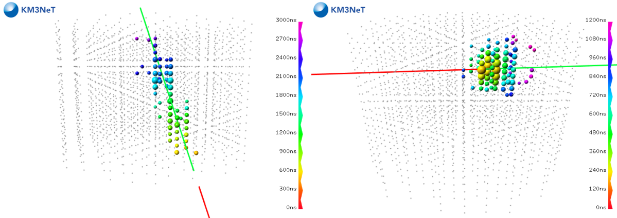
Figure 21: Event displays for a simulated \nu_\mu CC event (left) and a contained \nu_\mu NC event (right), showing only DOMs with a total ToT (summed over all 31 PMTs) of more than 30 ns in a narrow time window. In both cases, the incoming neutrino is indicated by the red line, and the outgoing lepton (muon or neutrino) by the green line. The colour scale gives the hit times with respect to the time of the neutrino interaction, while the size of the circles are proportional to the total ToT on each DOM. DOMs without hits are shown by grey dots.
