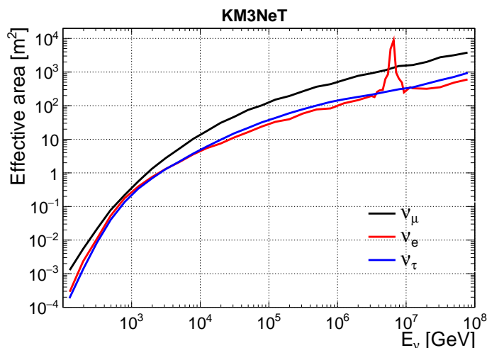
Figure 19: Effective areas of ARCA (two blocks) at trigger level for \nu_\mu , \nu_e , and \nu_\tau , as a function of neutrino energy E_\nu . The effective area is defined relative to an isotropic neutrino flux incident on the Earth, is averaged over both \nu and \bar{\nu} , and includes both NC and CC interactions. The peak at 6.3 PeV is due to the Glashow resonance of \bar{\nu}_e .
