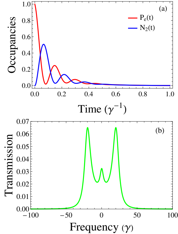
Figure 6.3: \kappa_2 = 10\gamma . (a) Time evolution of the photon numbers N_2(t) and the probability P_e(t) . (b) Frequency spectrum of the coupled cavities system.
