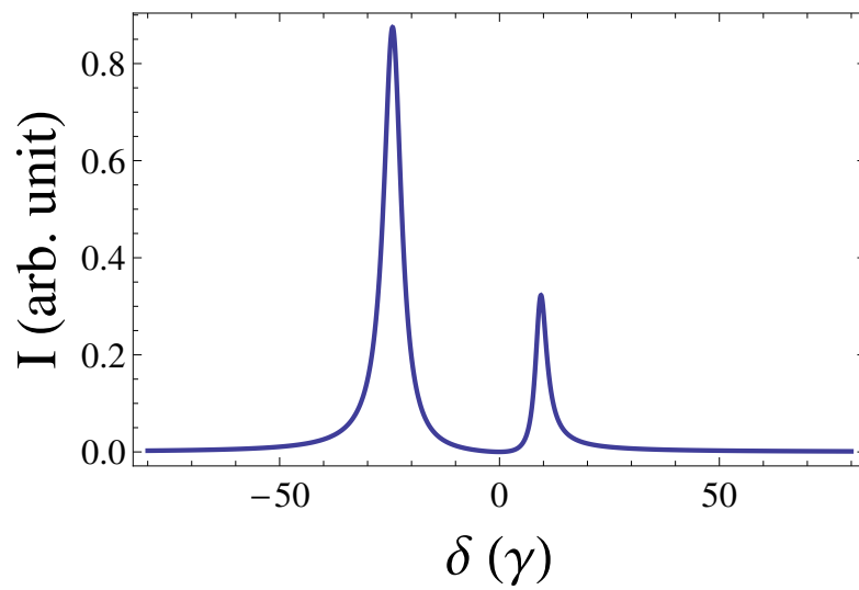
Figure 2.4: The radiation spectrum when C \gg (\Gamma - 2\gamma) and \phi \gg (\Gamma - 2\gamma) . The following numerical parameters were used: C = 15\gamma , \Gamma = 3\gamma , \phi = 30\gamma .
