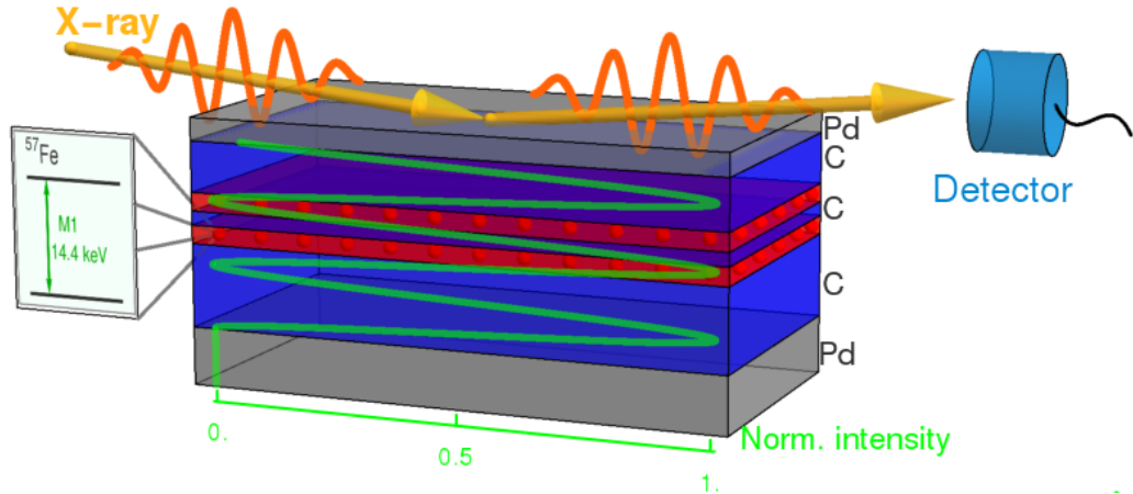
Figure 6.4: Schematic of the x-ray cavity containing two ^{57}\text{Fe} layers placed at a node and an antinode of the standing wave.
