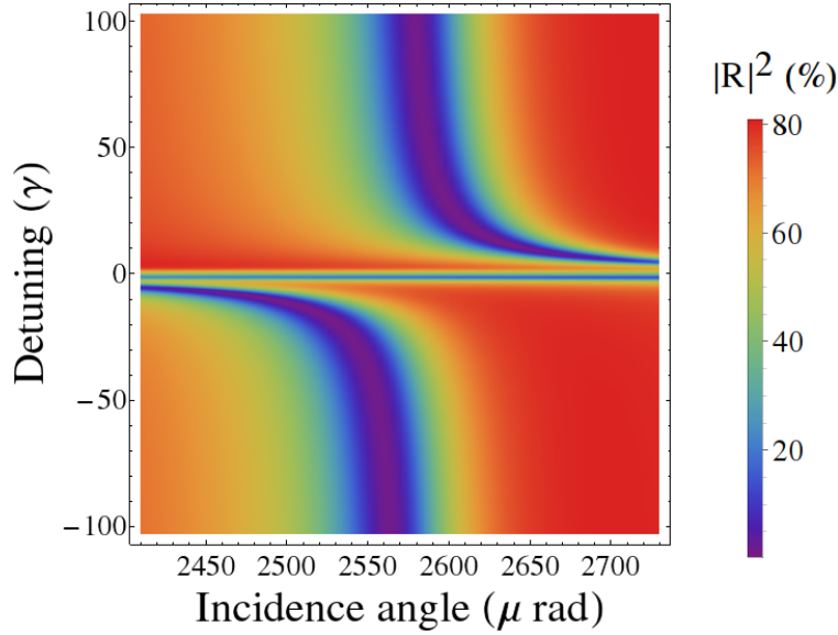
Figure 6.10: CONUSS reflectivity as a function of the incidence angle and the detuning for the cavity structure presented in Table 6.3.
